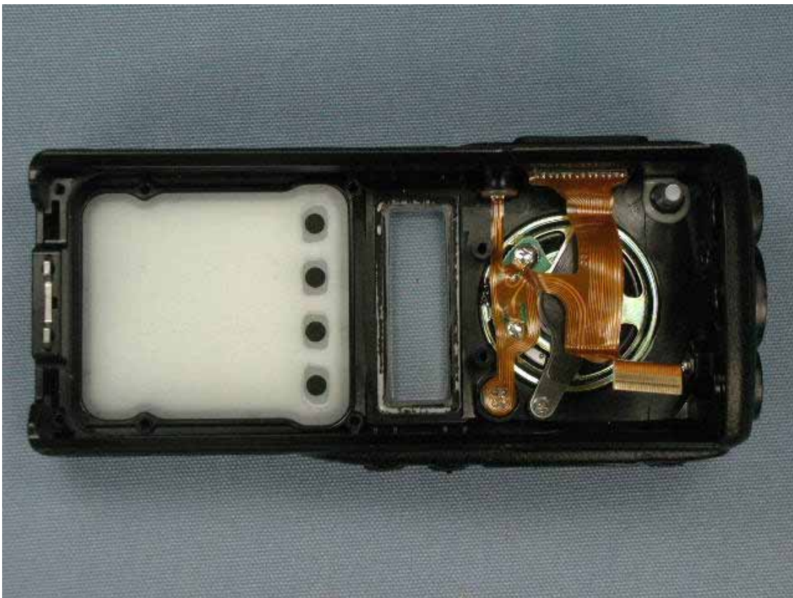
Inside of front panel (for VX-924/974)
