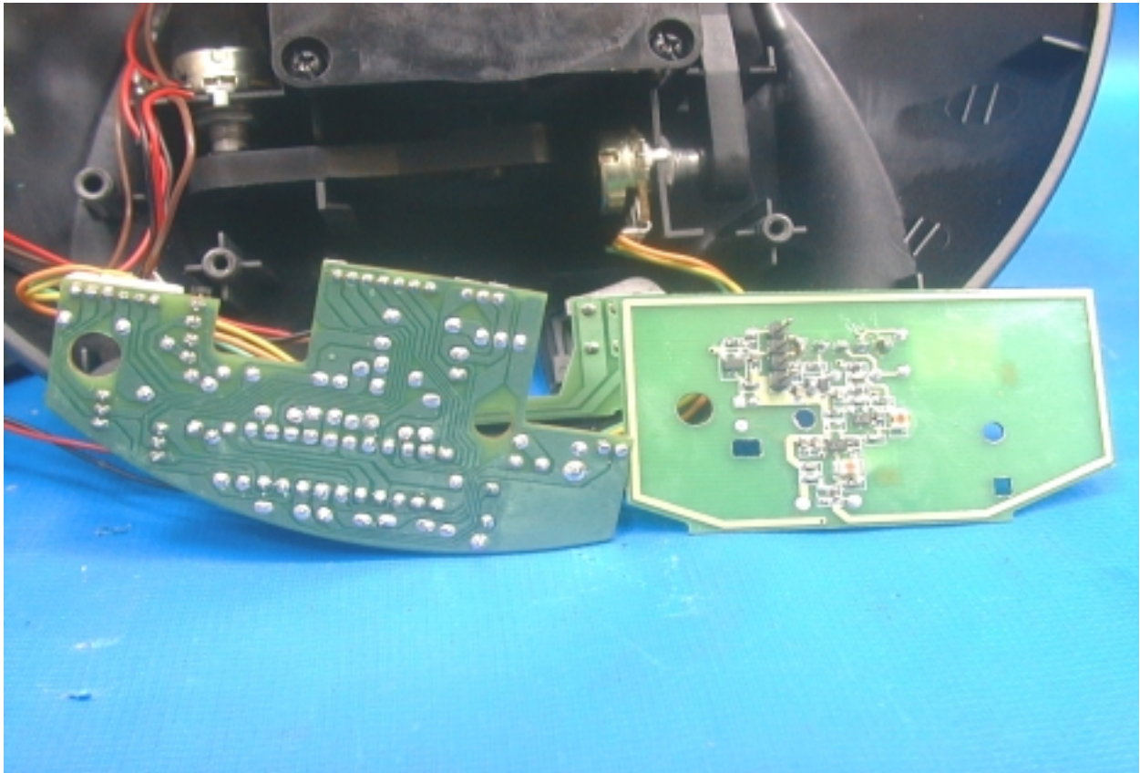
PHOTO. 7. COMPONENT SIDE VIEW OF EUT'S RECEIVER
