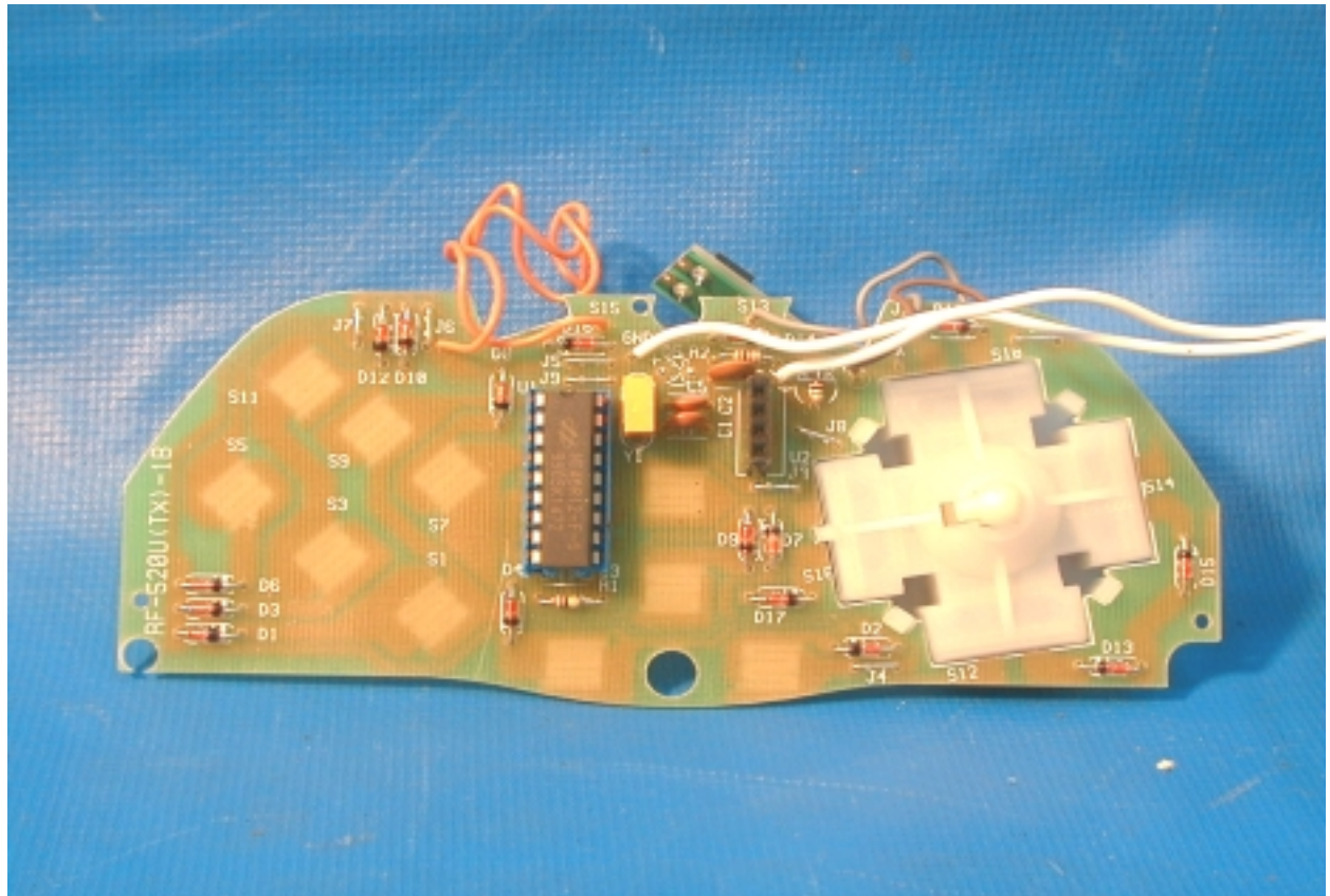
PHOTO. 7. EUT COMPONENT SIDE VIEW
