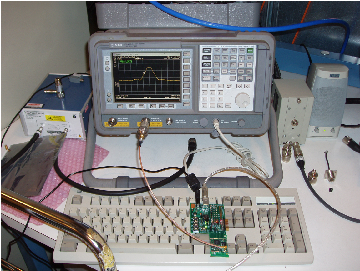
Photo 3 – Conducted Test Set-up
