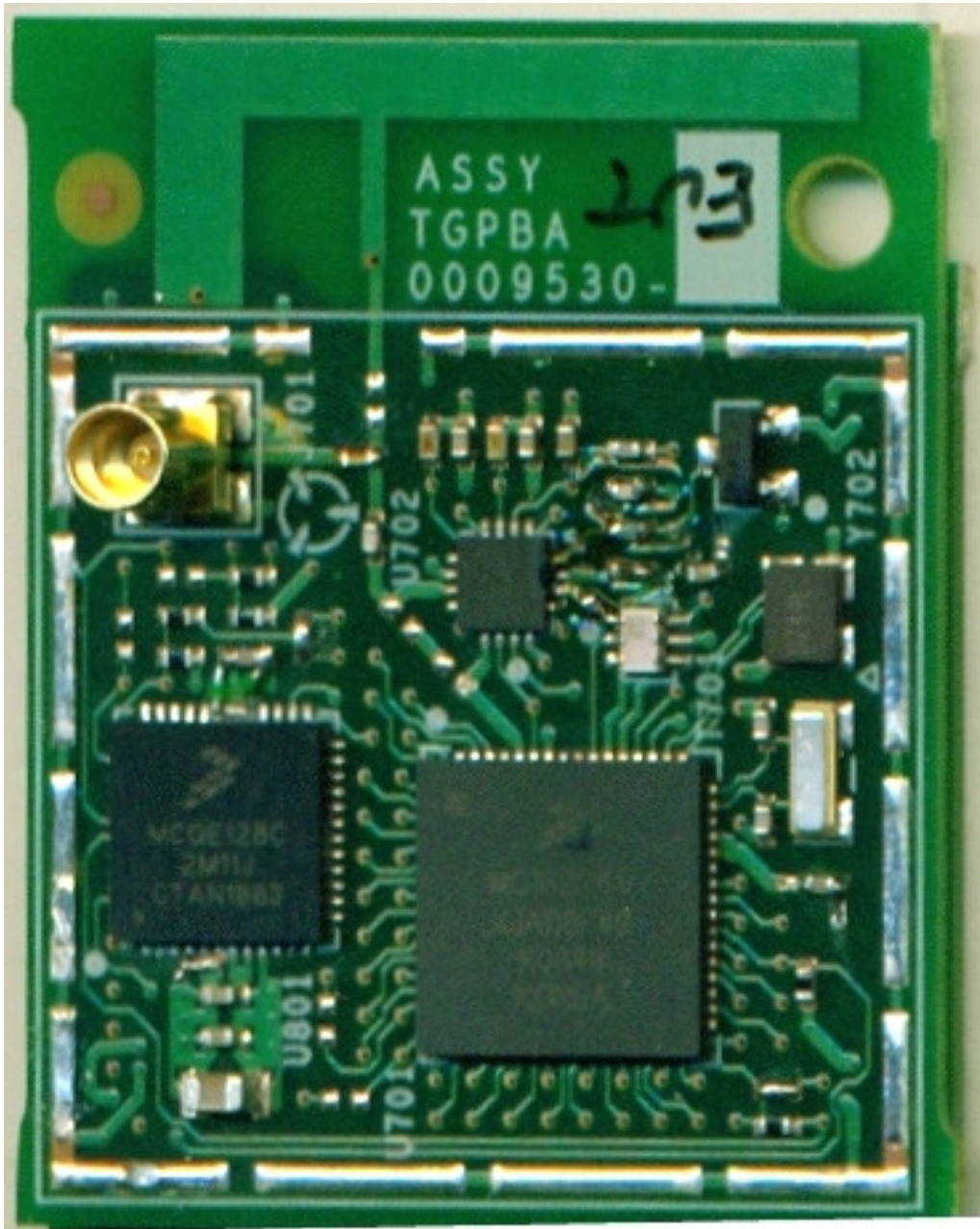
Photo 1 – EUT Top View with Shield Removed and MMCX Connector Populated 1
