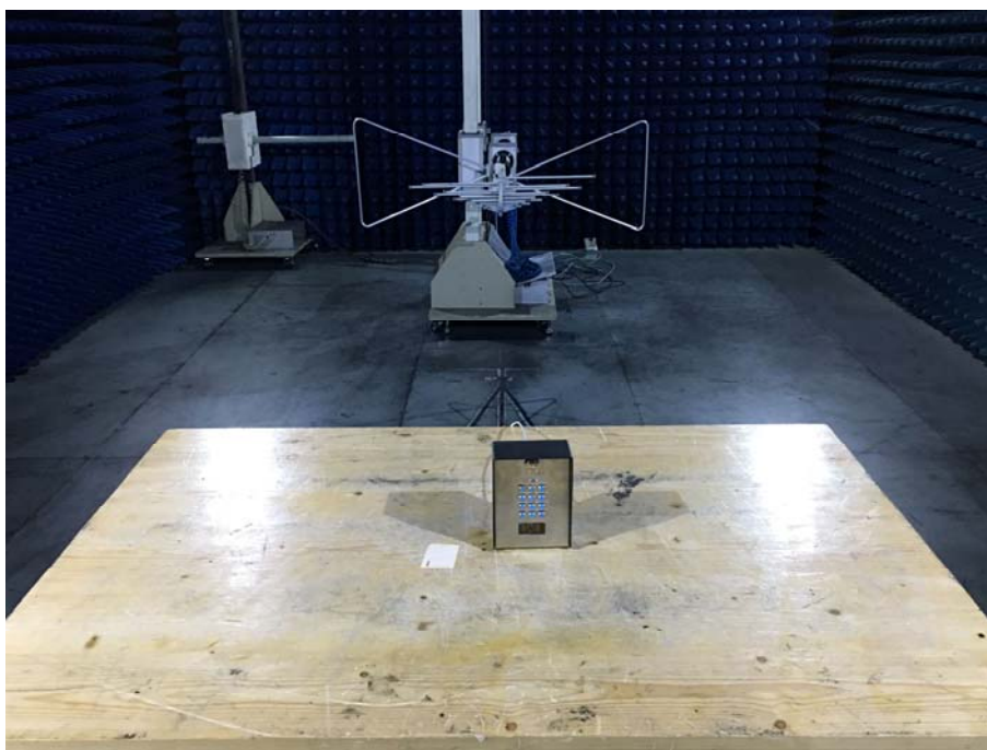
Photo of Radiation Emission Measurement: 30MHz to 1GHz
