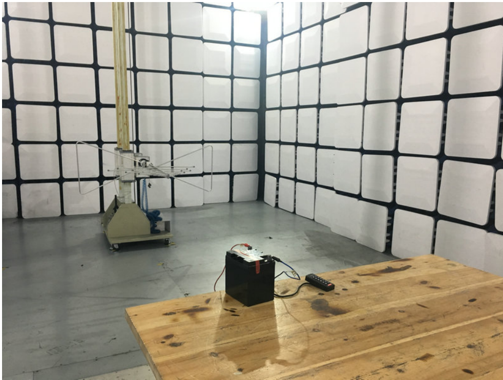
FCC ID: K4E2612SPQ Photo of Radiation Emission Test
