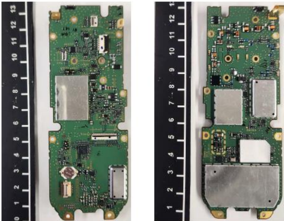
TX-RX UNIT with shield case
