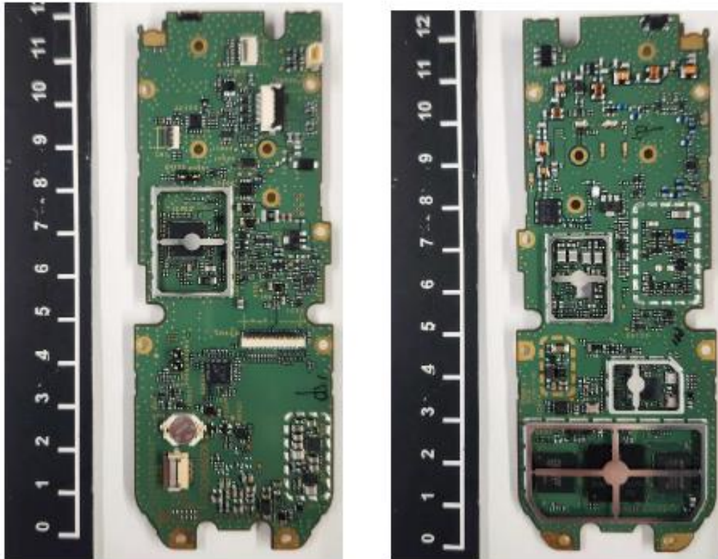
TX-RX UNIT without shield case
