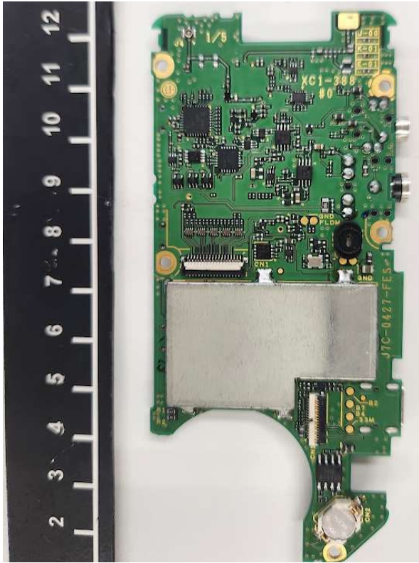
CONTROL Unit with Shielding case
