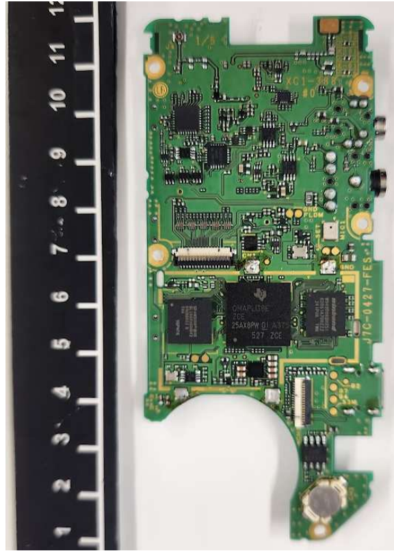
CONTROL Unit without Shielding case
