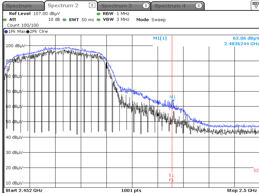
Radiated Restricted Band Edges plot –Peak Reading (802.11n (HT20) Ch.11, X-H)
