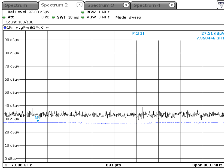
Radiated Spurious Emissions plot – Average Reading (802.11b, Ch.11 3rd Harmonic)
