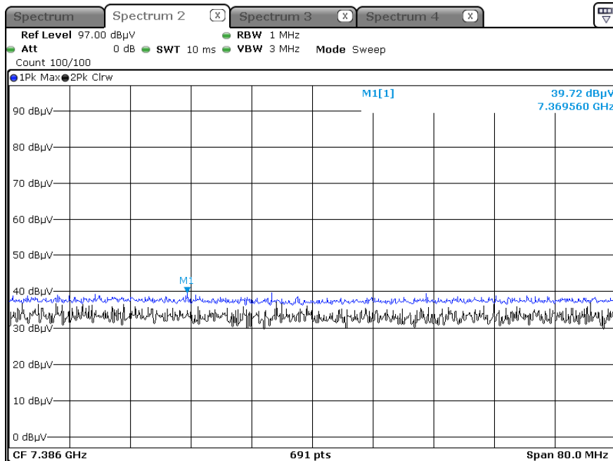
Radiated Spurious Emissions plot – Peak Reading (802.11b, Ch.11 3rd Harmonic)
