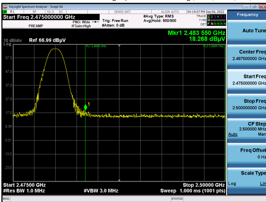
Radiated Restricted Band Edges plot –Peak Reading (GFSK, Ch.78, Z-H)
