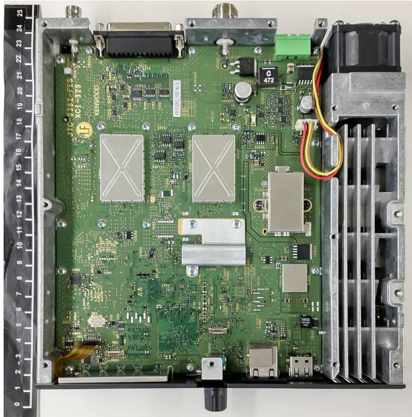
Top Internal View of MAIN Unit
