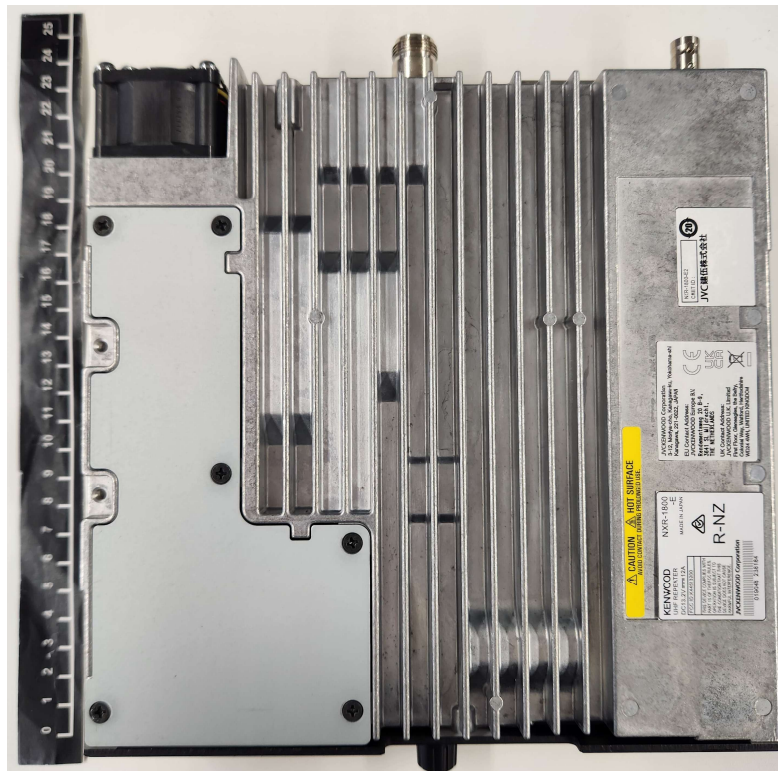
Bottom View
