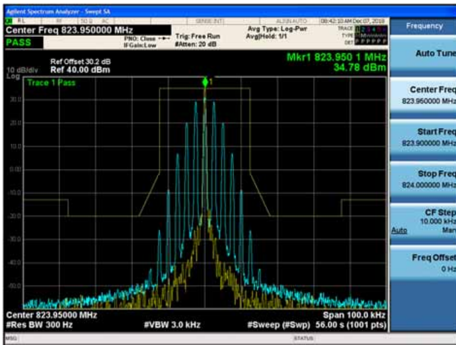
(14K0F3E _ 823.95 MHz)_High
