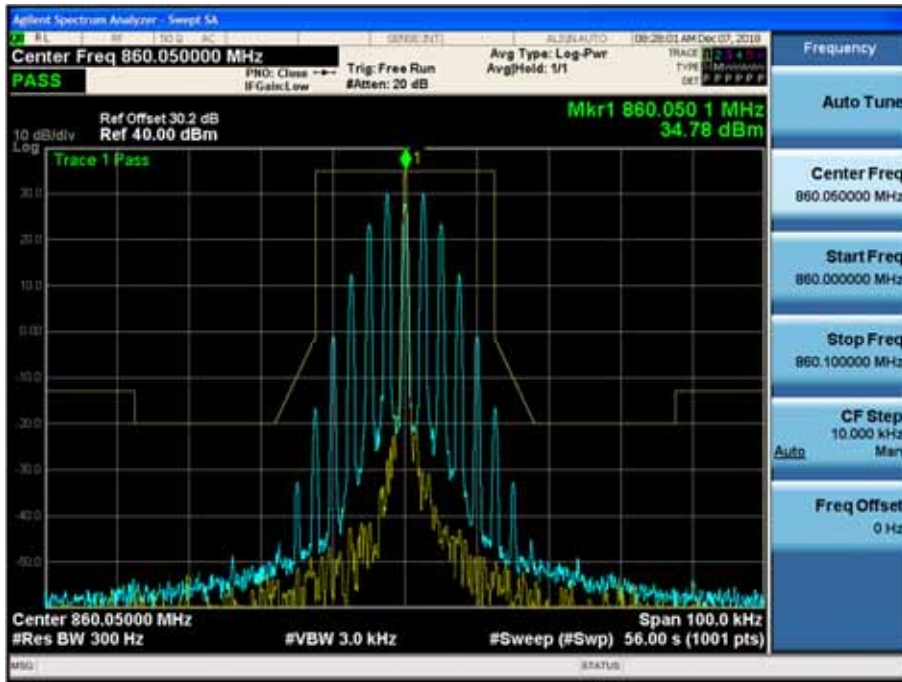
(16K0F3E _ 860.05 MHz)_High
