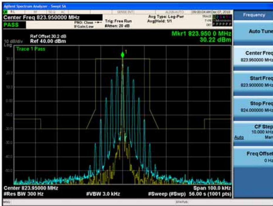
(14K0F3E _ 823.95 MHz)_Low
