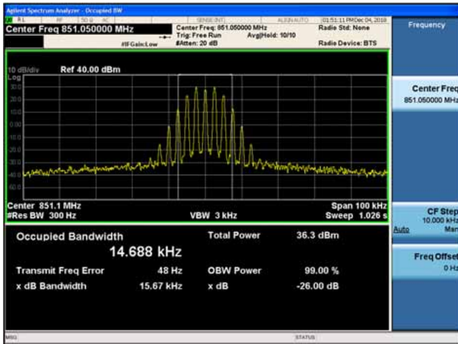
(16K0F3E _ 851.05 MHz)_High
