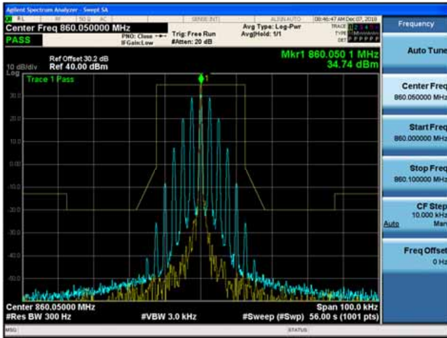
(14K0F3E _ 860.05 MHz)_High
