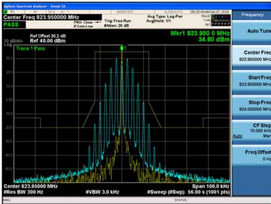
(16K0F3E _ 823.95 MHz)_High
