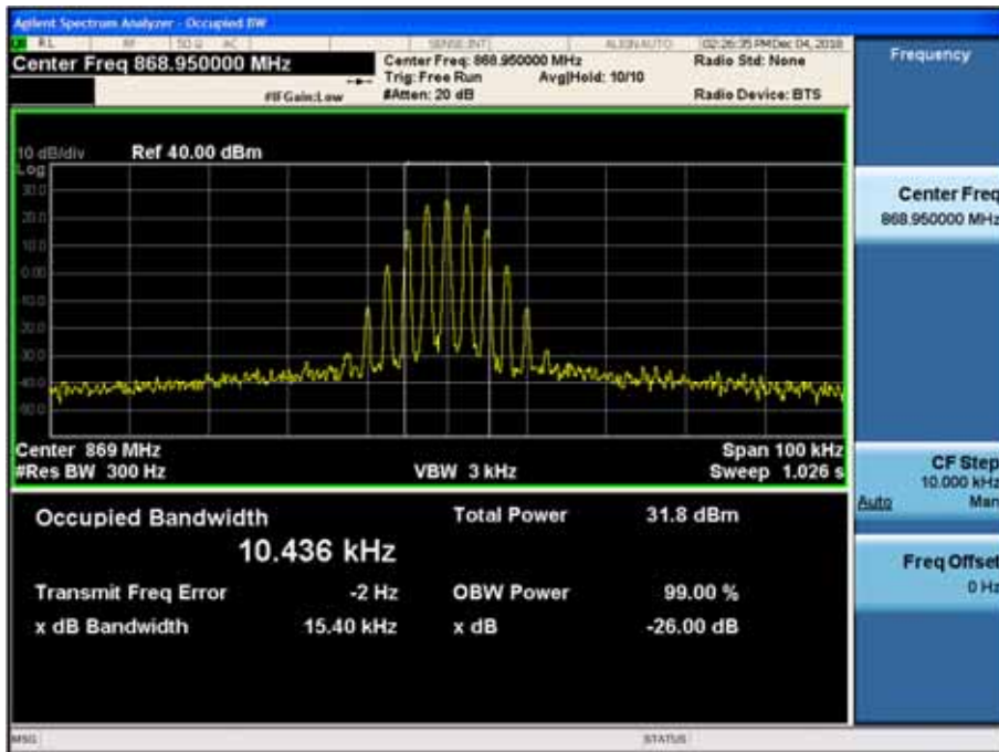
(14K0F3E _ 868.95 MHz)_Low
