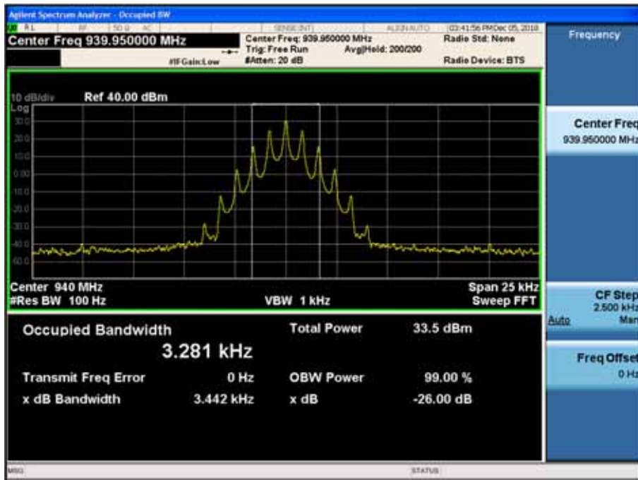
(4K00F2D _ 939.95 MHz)_Low
