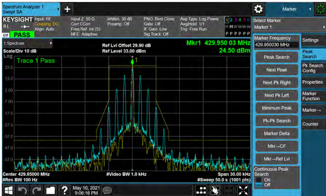
(429.95 MHz)_Low
