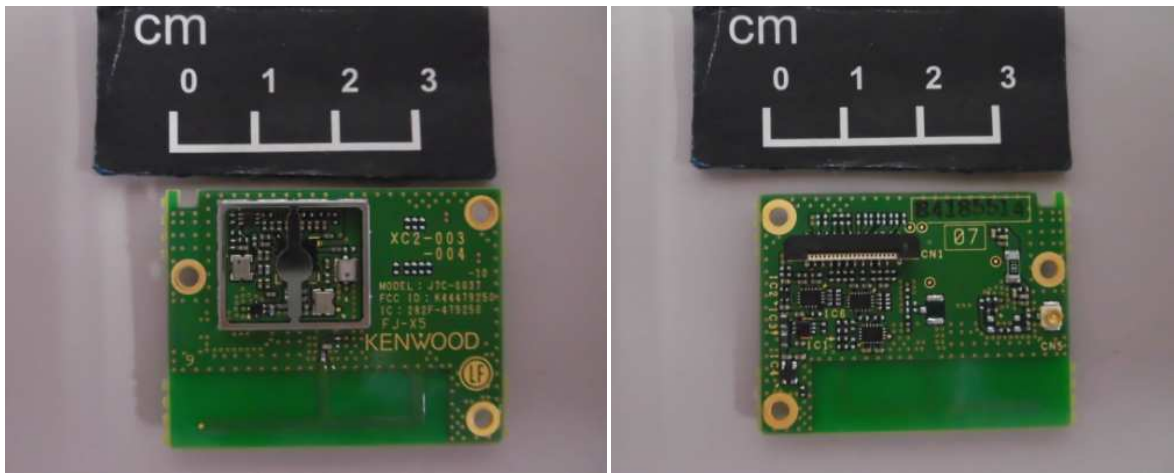
Certificated Bluetooth Module (FCC ID: K44479250, MODEL: J7C-0037)
