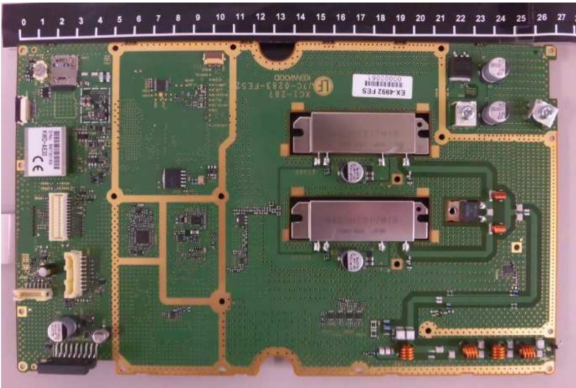
MAIN Unit
