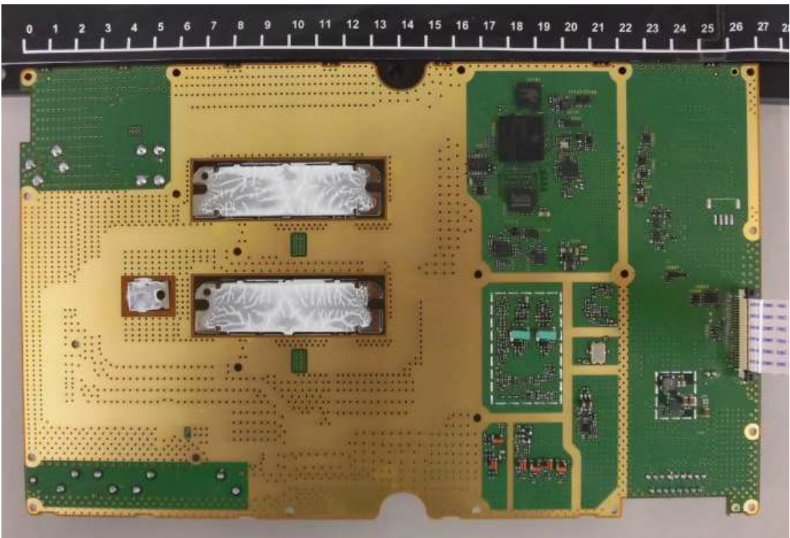
MAIN Unit
