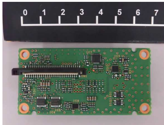
INTERFACE Unit
