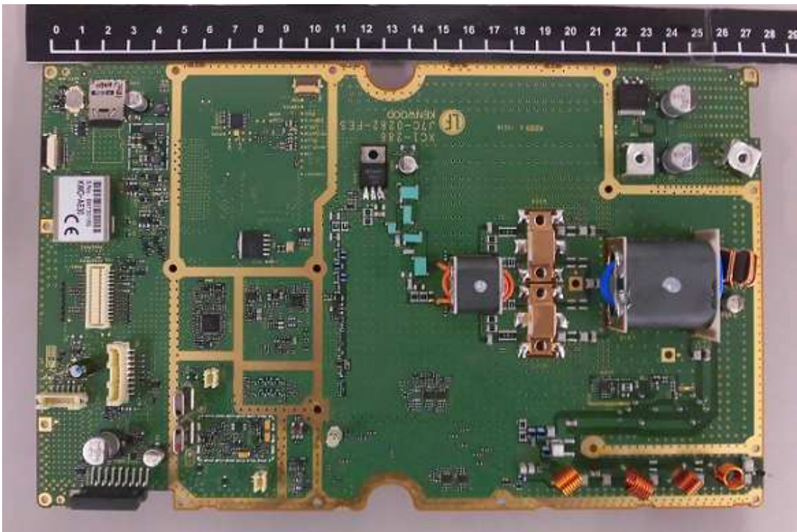
MAIN UNIT
