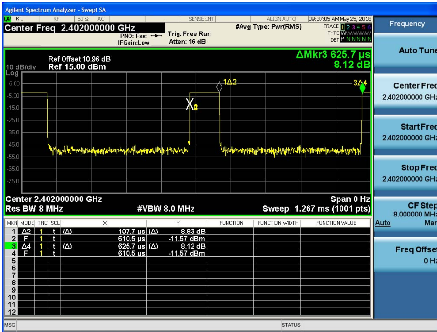
Duty Cycle plot (Low-CH 0)
