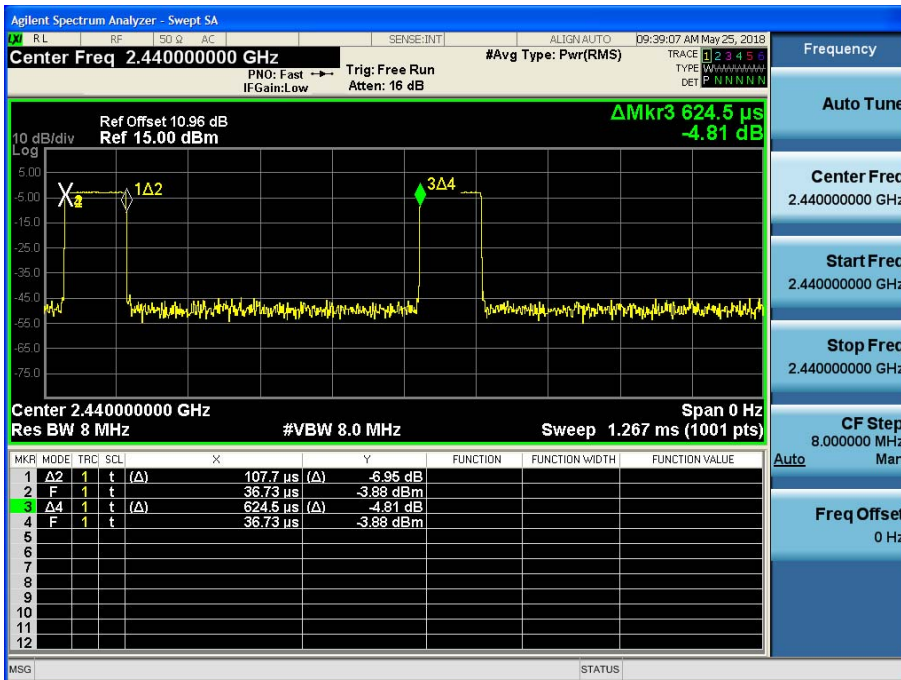
Duty Cycle plot (Mid-CH 19)
