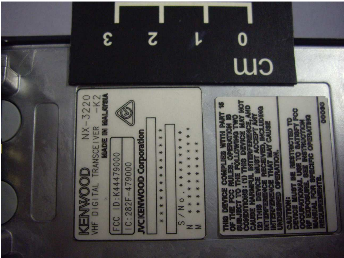
MODEL NAME PLATE and CAUTION STICKER of NX-3220-K2
