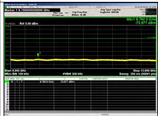
9 – 13 GHz
