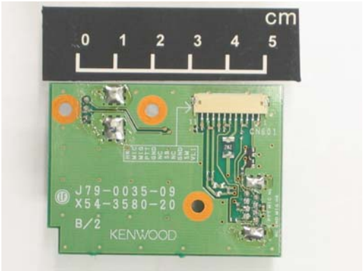
Display B Component Side View
