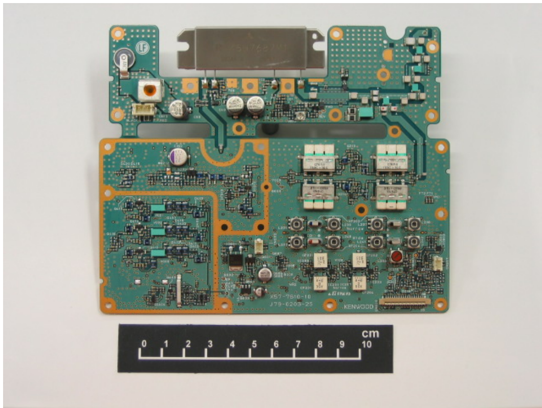
TXRX Component Side View
