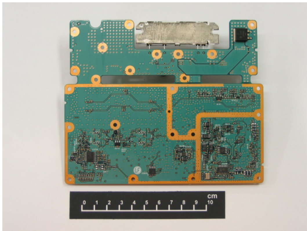
TXRX Foil Side View
