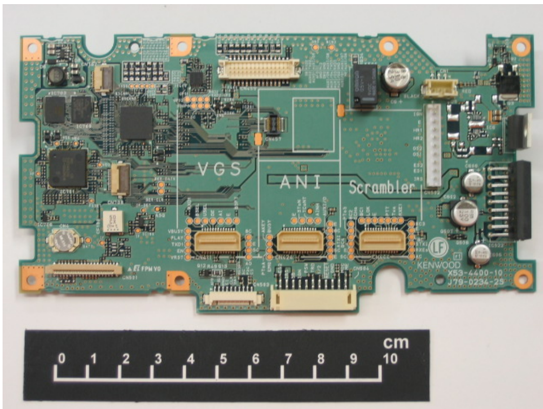
Control Component Side View
