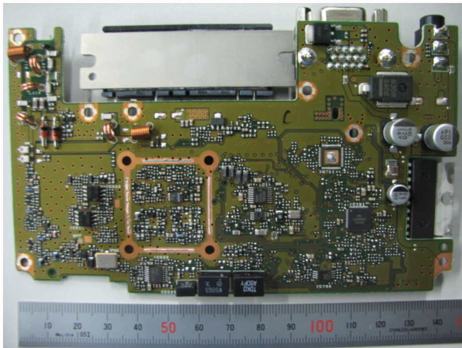
TXRX Foil Side View
