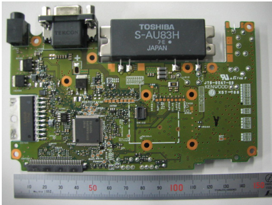
TXRX Component Side View
