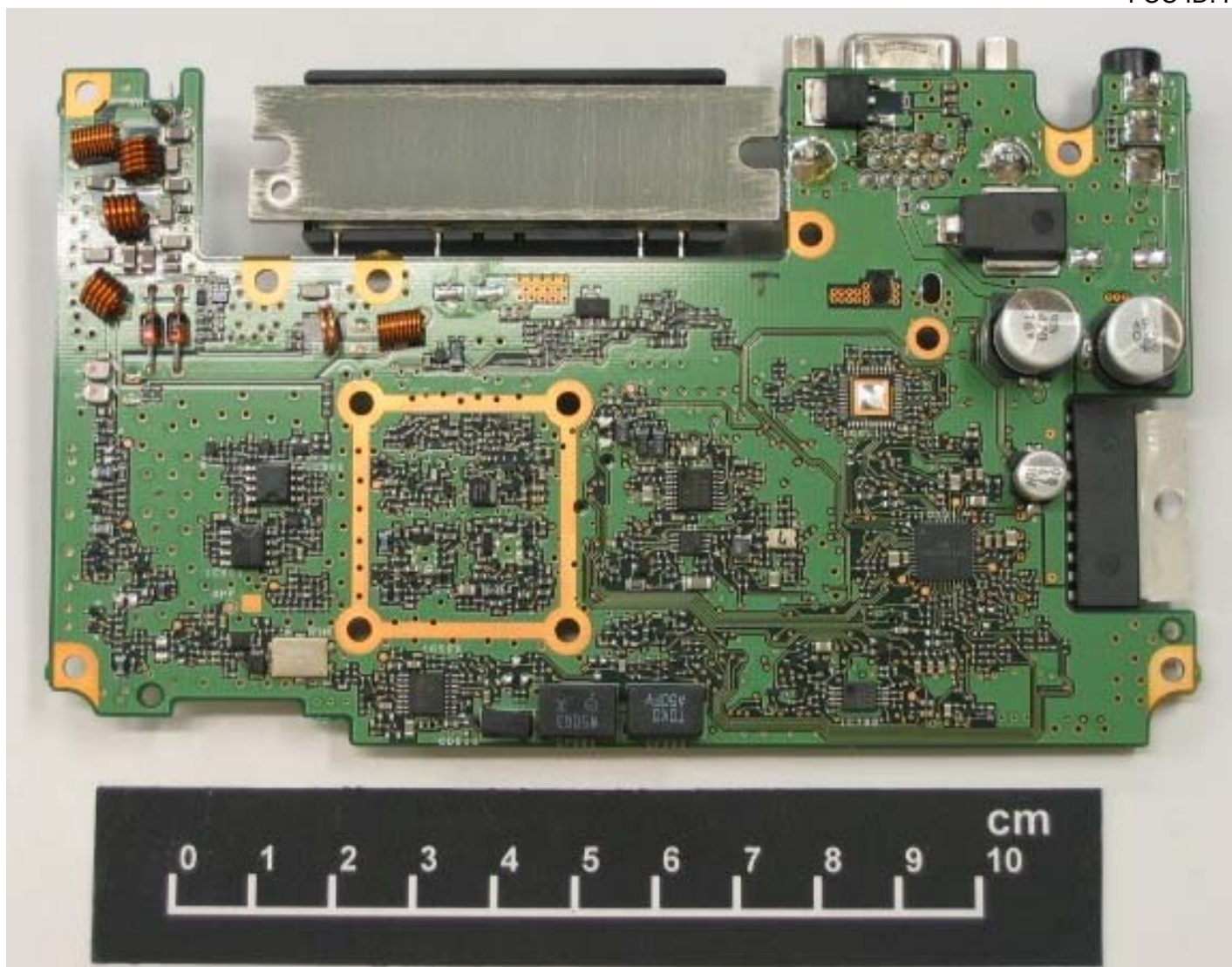
TXRX Foil Side View
