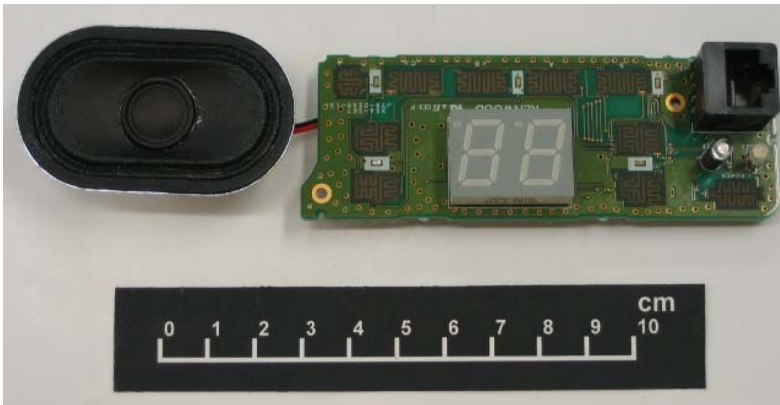
Display Component Side View
