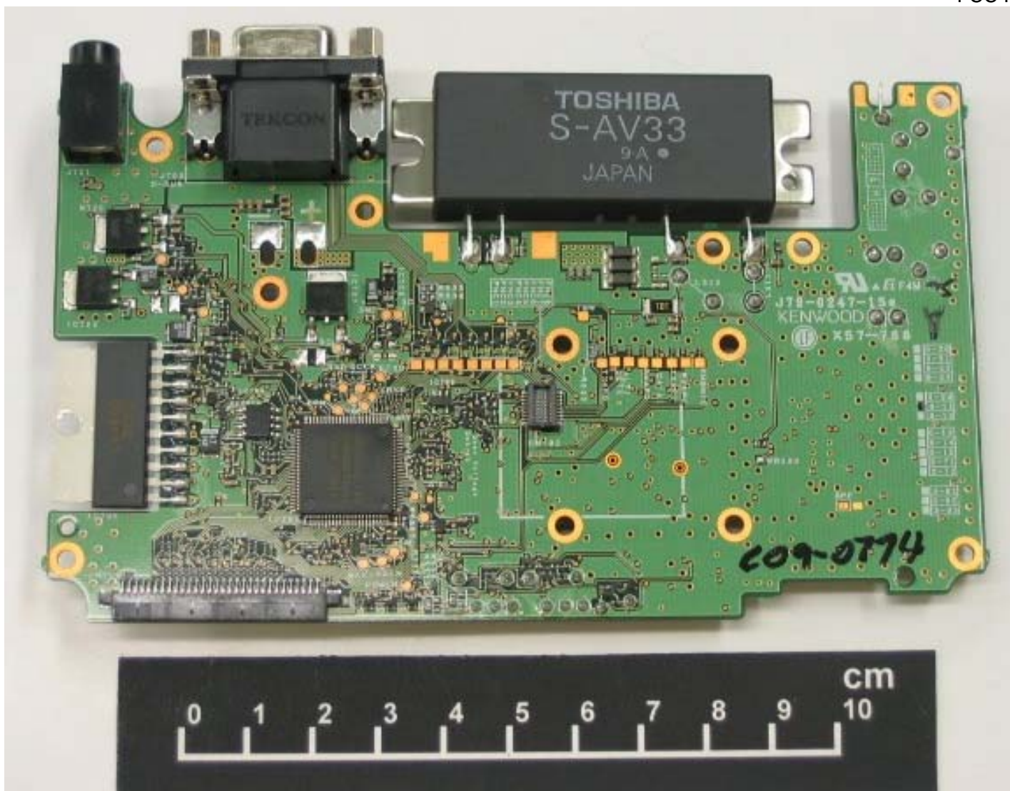
TXRX Component Side View
