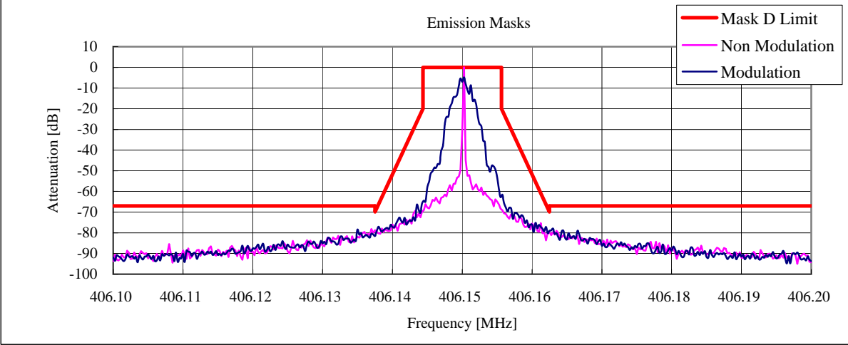
State : Low Power / 12.5 kHz channel bandwidth:GMSK / 406.15 MHz
