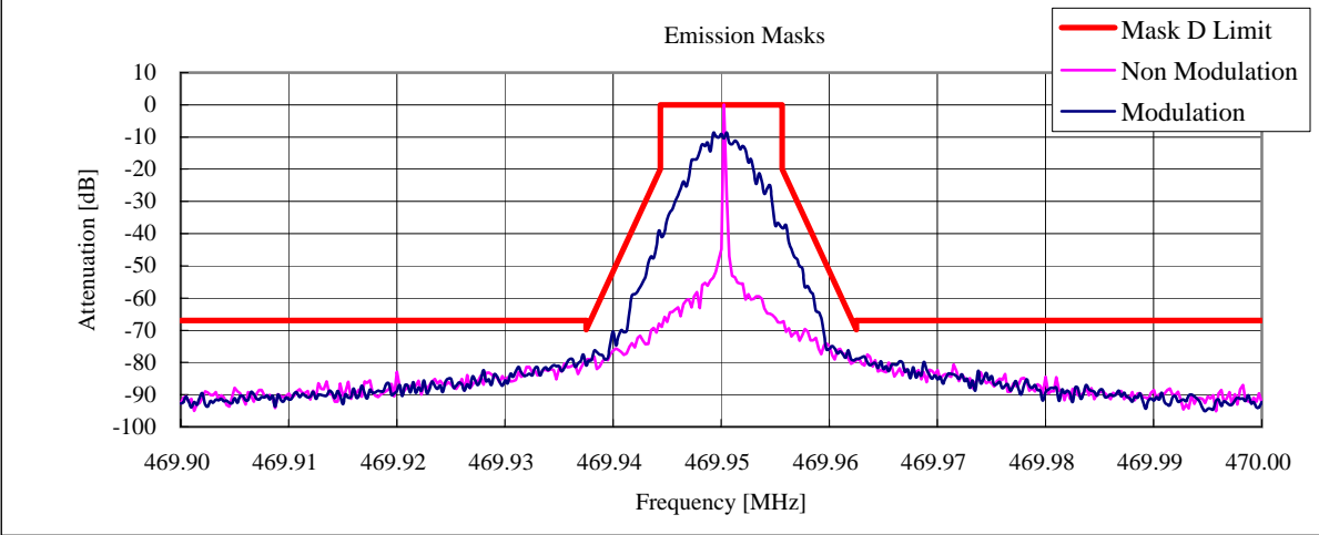
State : Low Power / 12.5 kHz channel bandwidth:C4FM / 469.95 MHz
