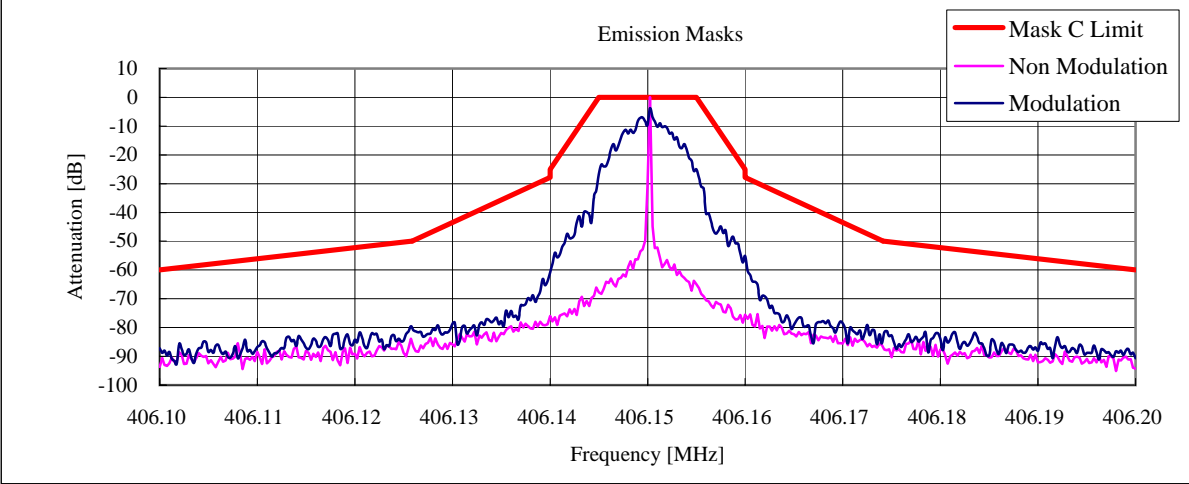
State : Low Power / 25 kHz channel bandwidth:GMSK / 406.15 MHz
