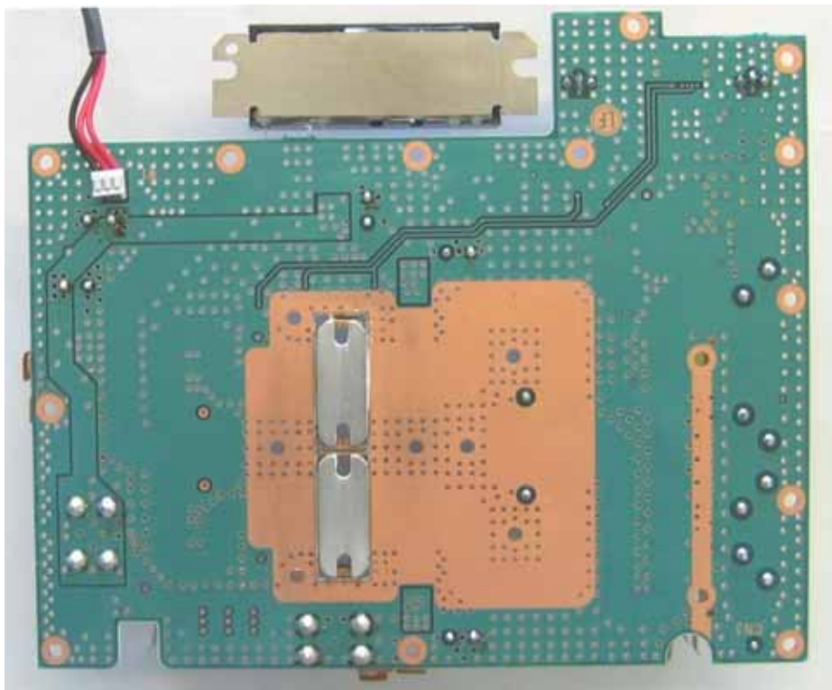
Final Foil Side View
