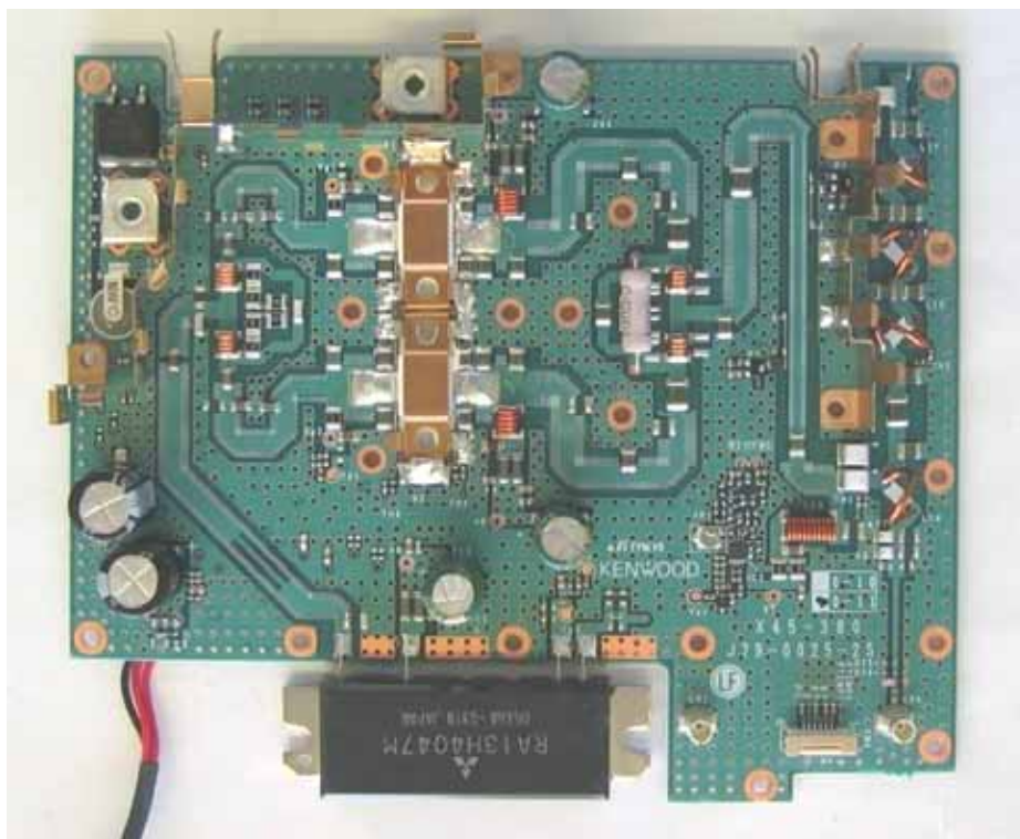
Final Component Side View
