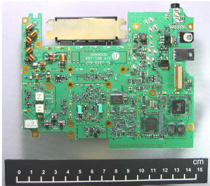
TXRX Foil Side View 1/2
