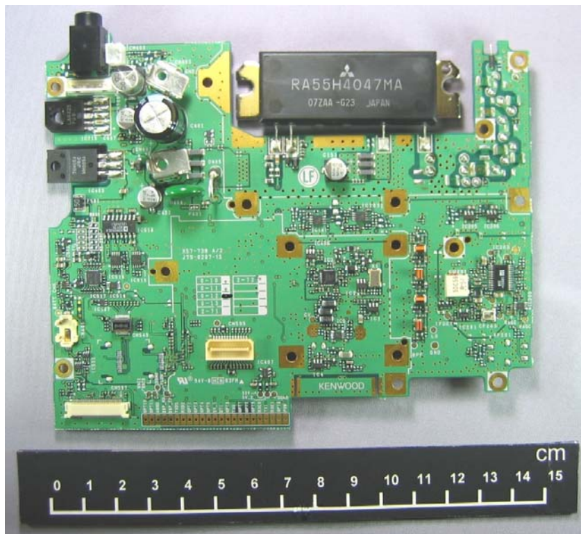
TXRX Component Side View 1/2
