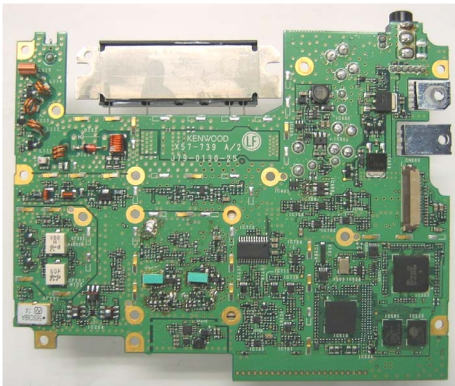
TXRX Foil Side View 1/2
