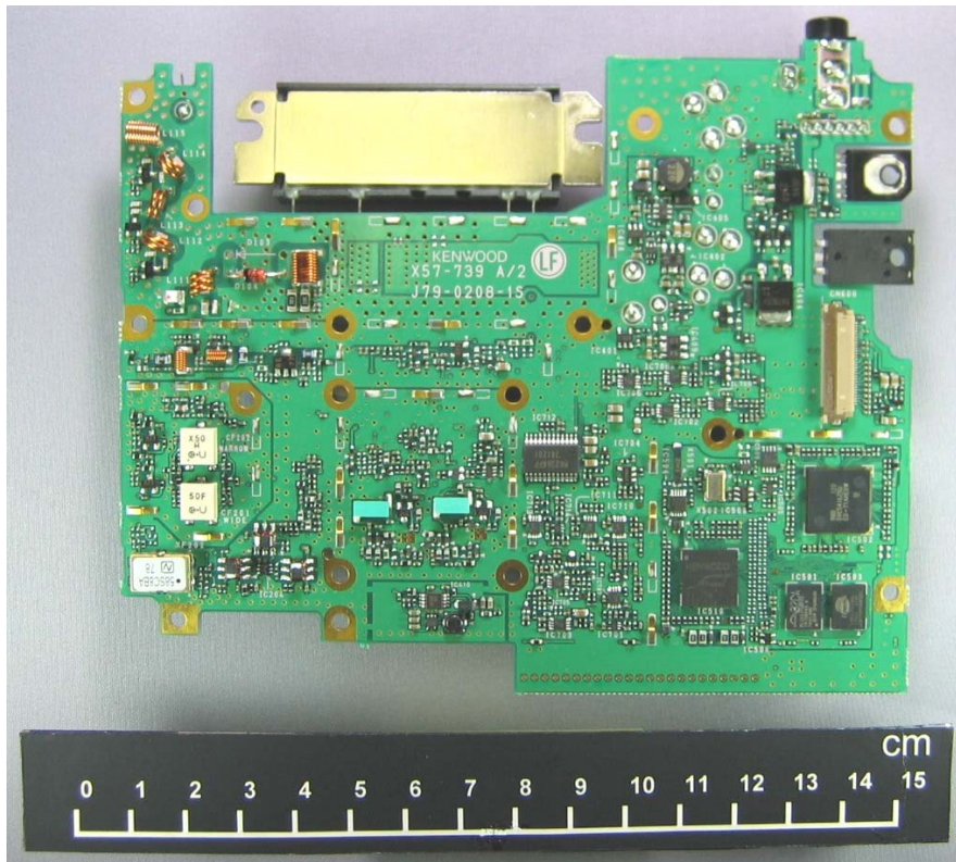
TXRX Foil Side View 1/2
