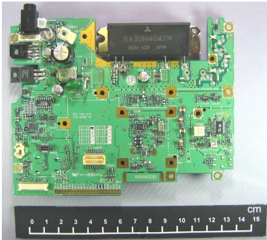
TXRX Component Side View 1/2
