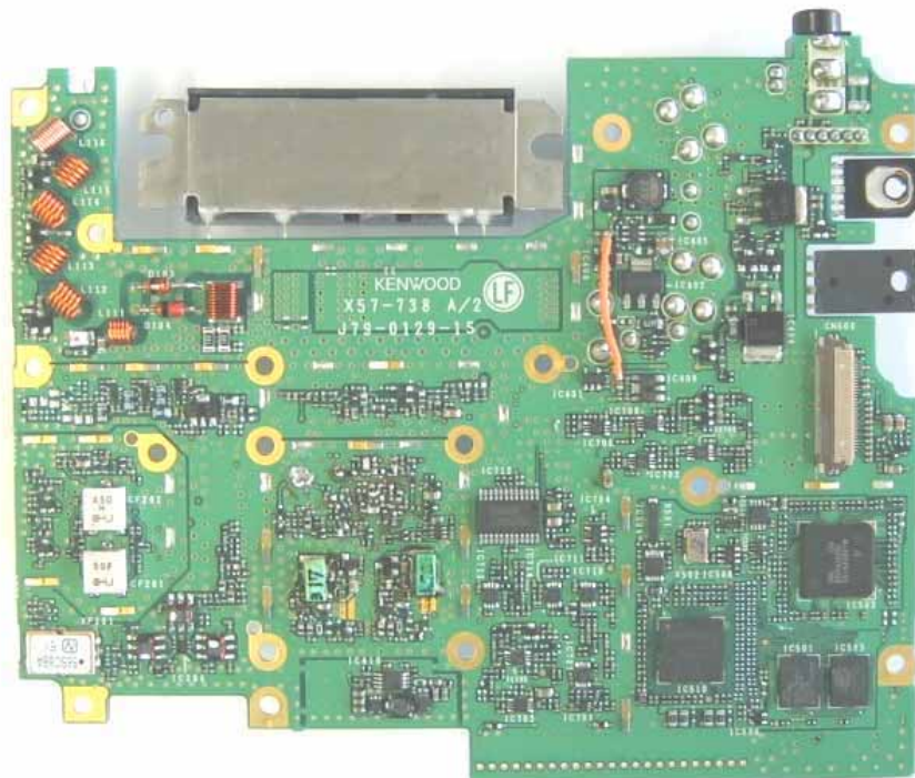
TXRX Component Side View 1/2
