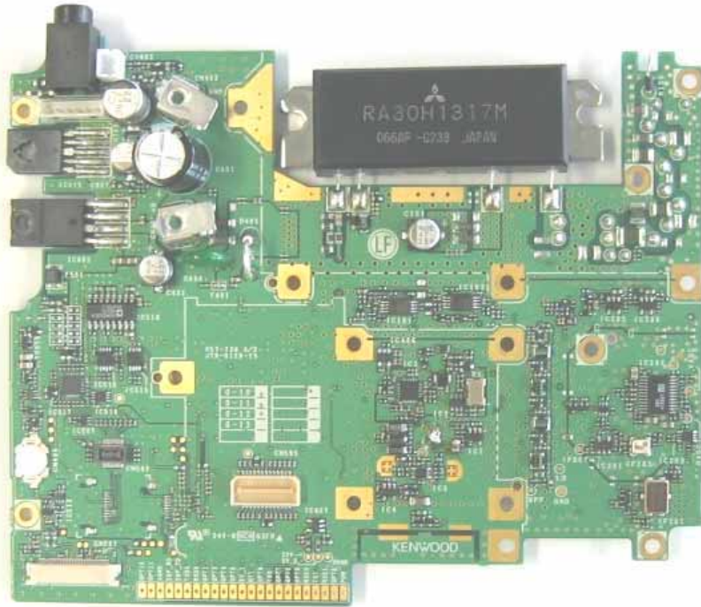
TXRX Component Side View 1/2
