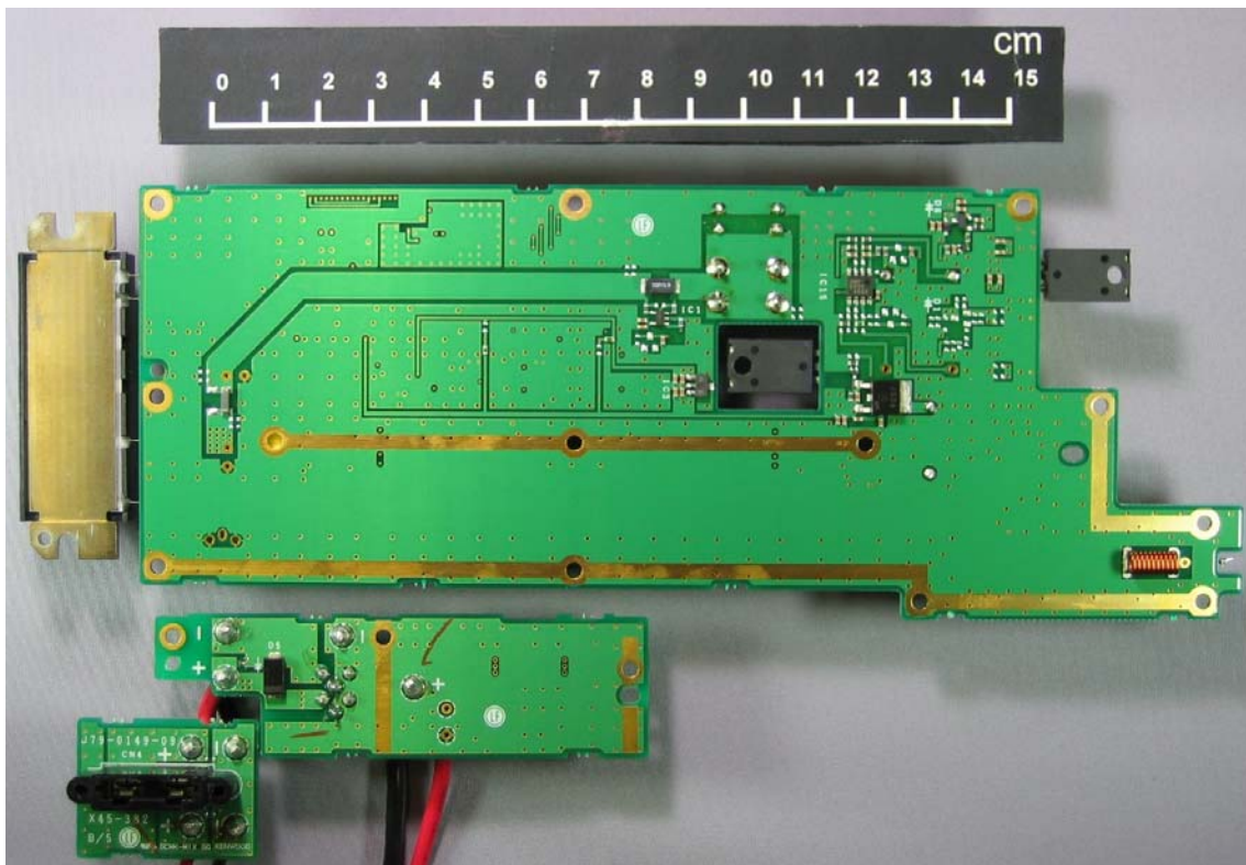
Final Foil Side View
