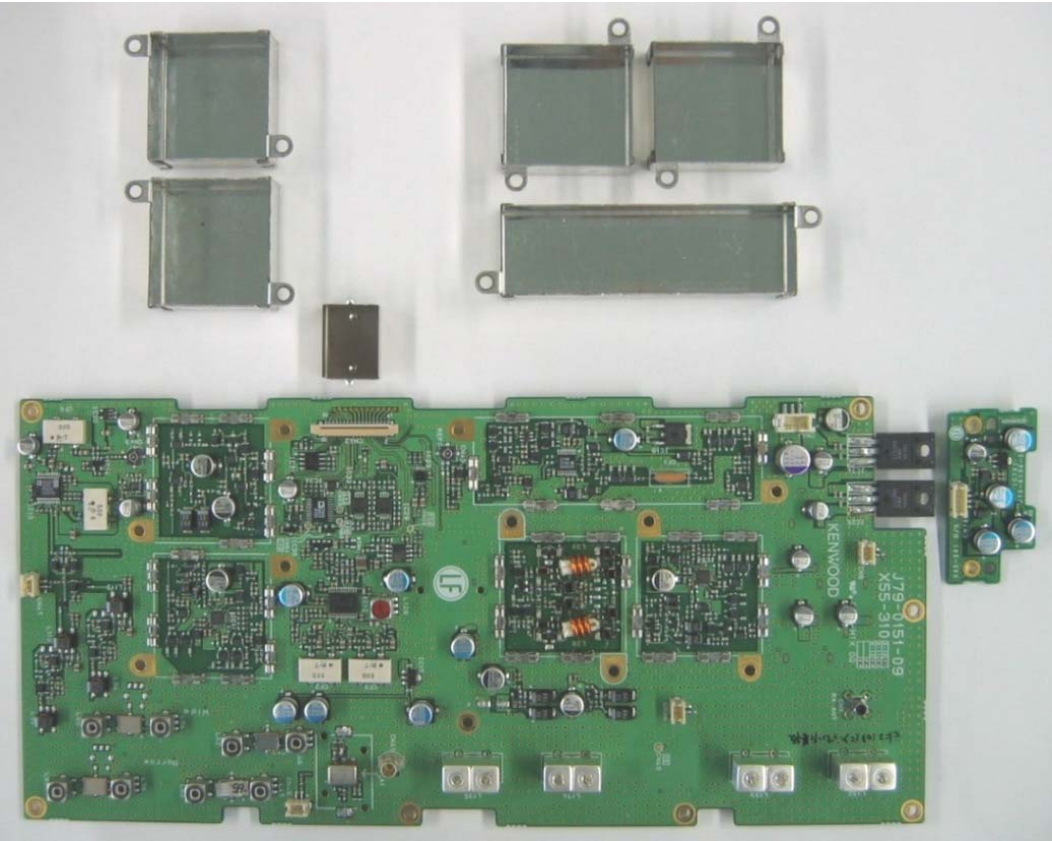
RX Component Side View
