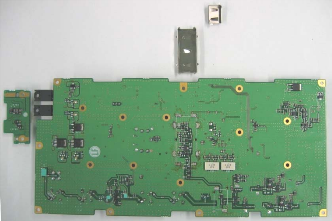
RX Foil Side View
