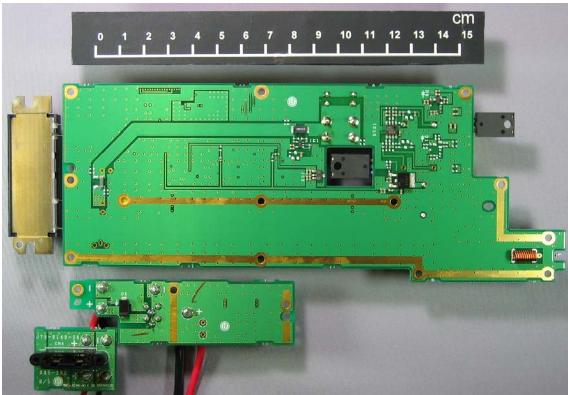
Final Component Side View
