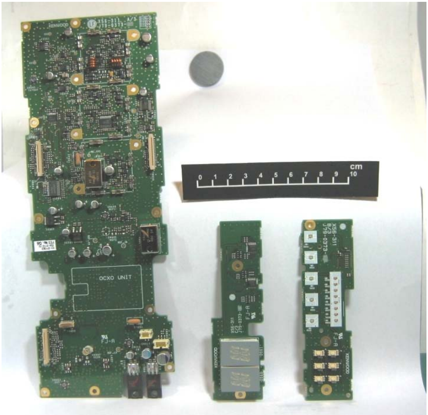
TX Component Side View
