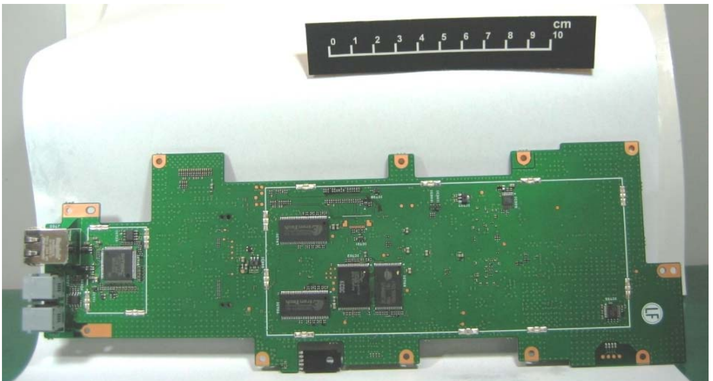
Control2 Foil Side View
