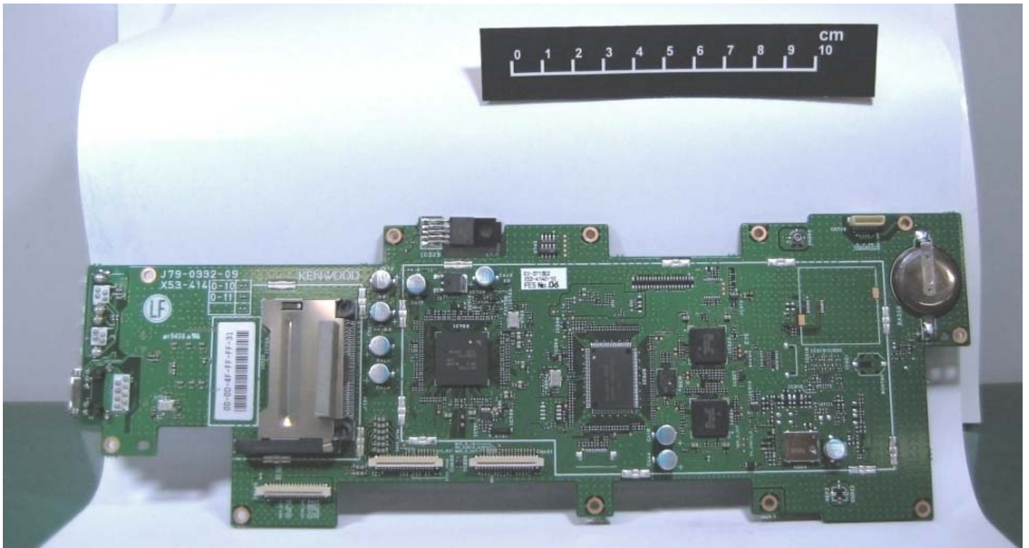
Control2 Component Side View
