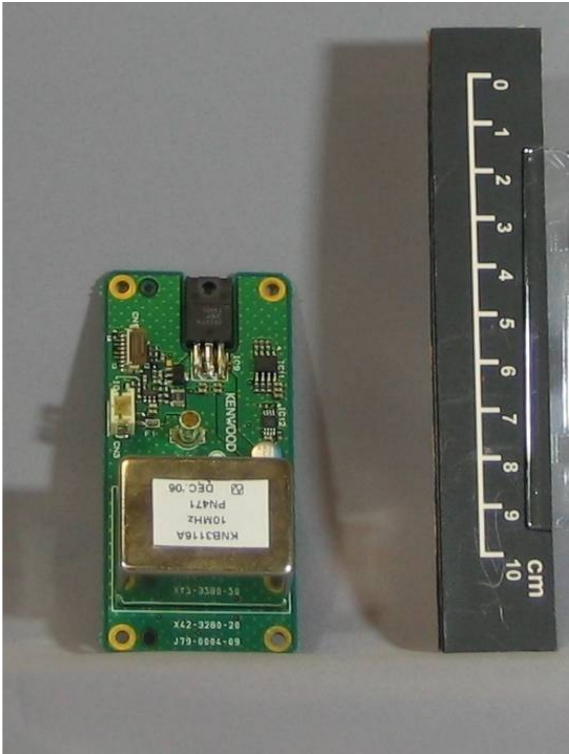
KKK-3 OCXO UNIT Component Side View
