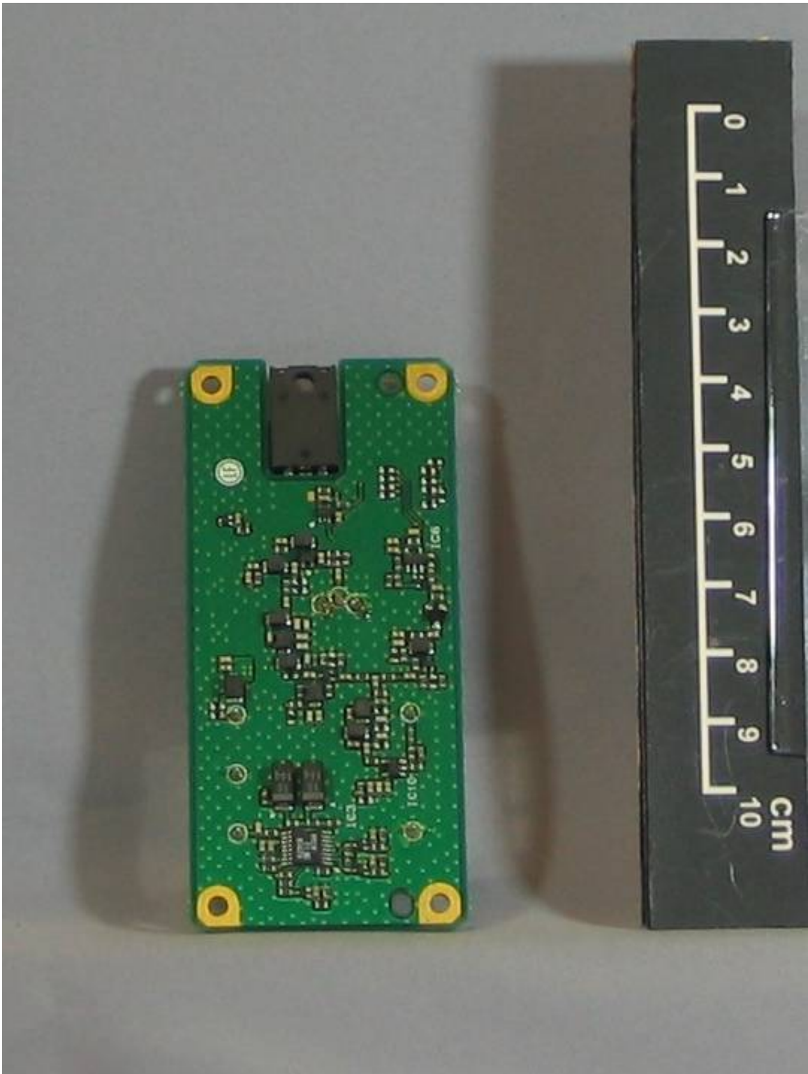
KXK-3 OXCO UNIT Foil Side View
