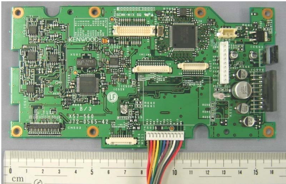
Control Component Side View
