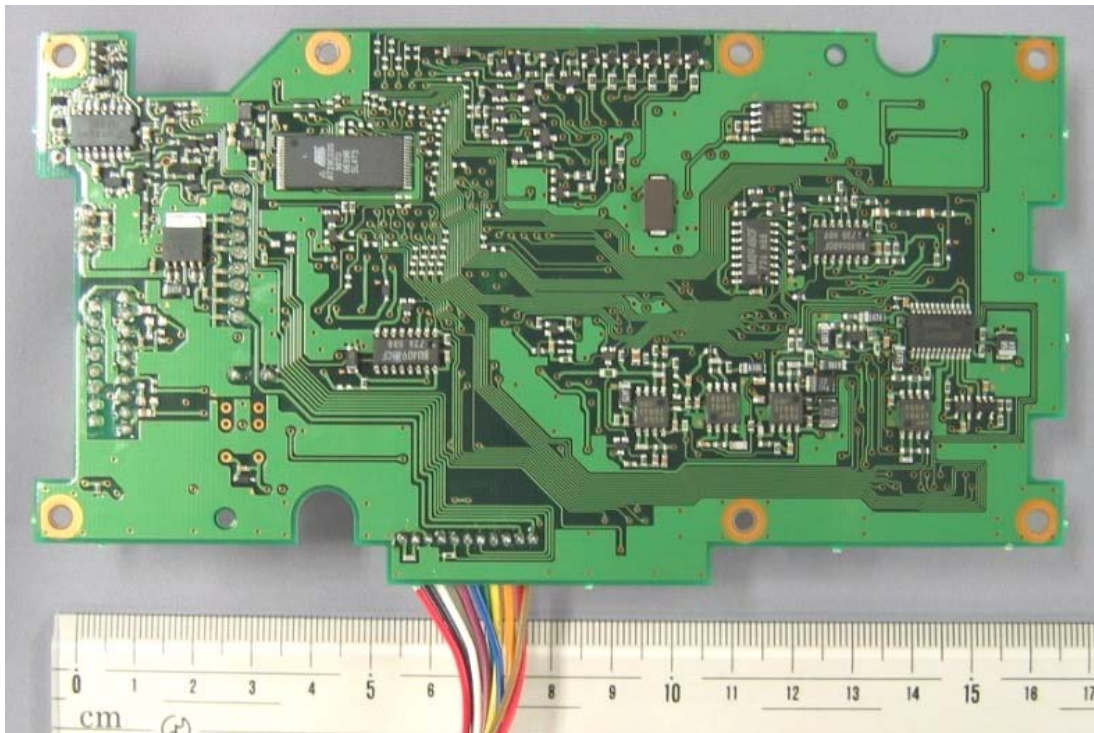
Control Foil Side View
