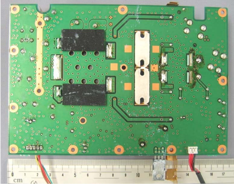
PA Foil Side View
