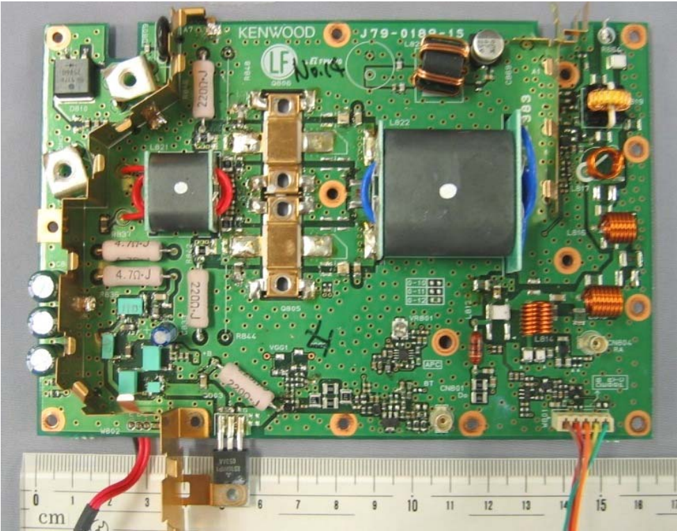
PA Component Side View
