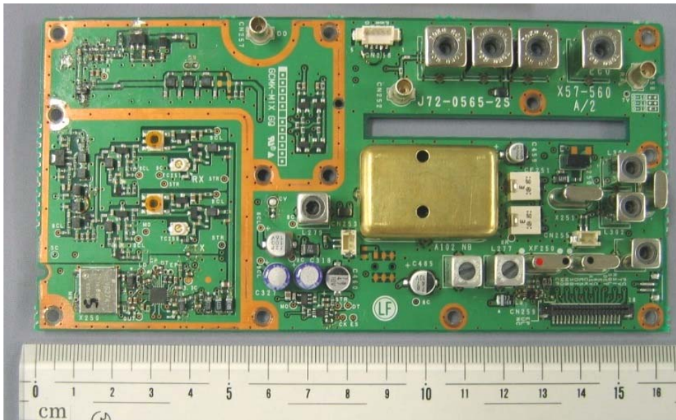
TXRX Component Side View with shielding
