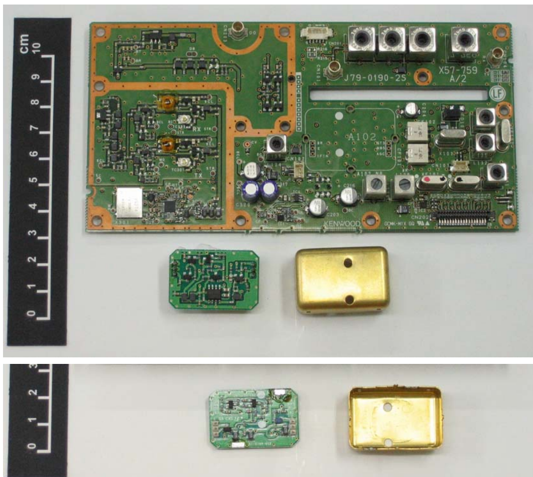
TXRX Component Side View without shielding
