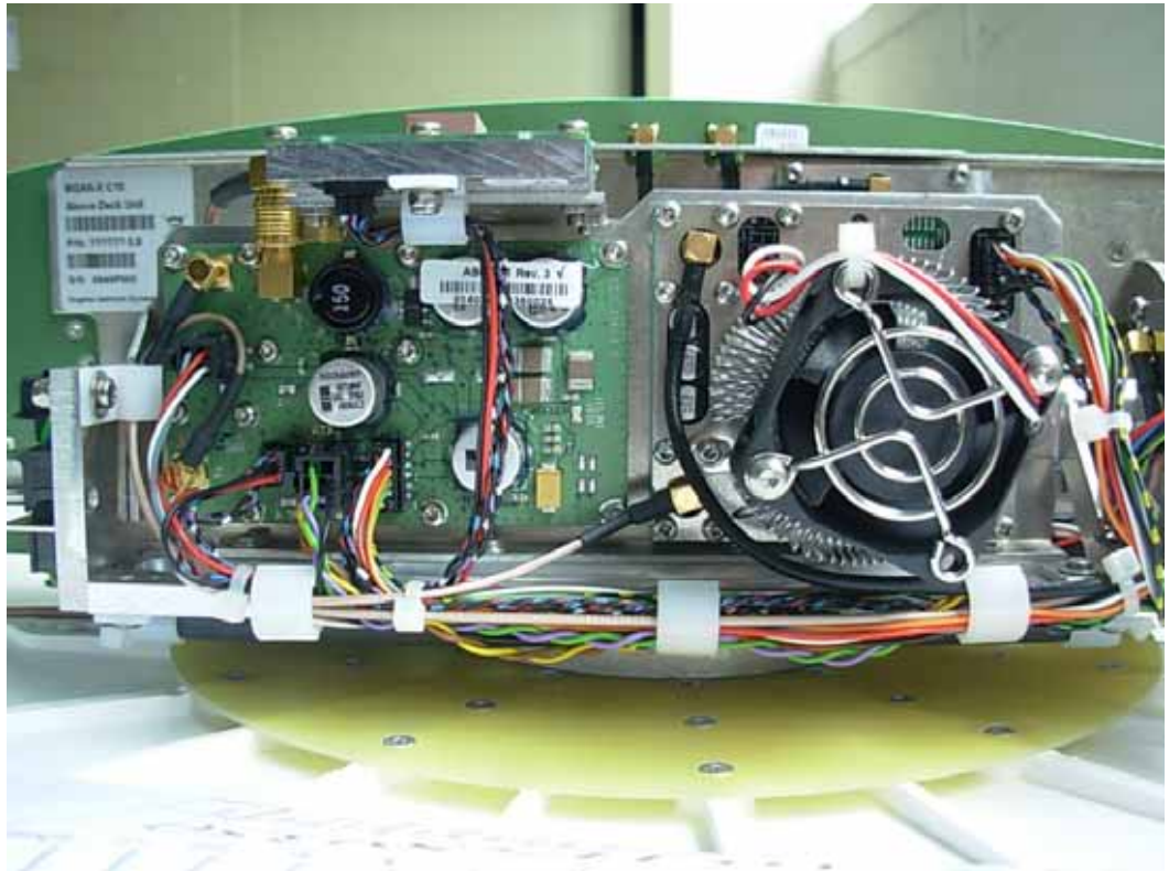
FIGURE 25 LAND MOBILE TERMINAL (M/N: 9350-10) SATELLITE ANTENNA – INSIDE REAR VIEW
