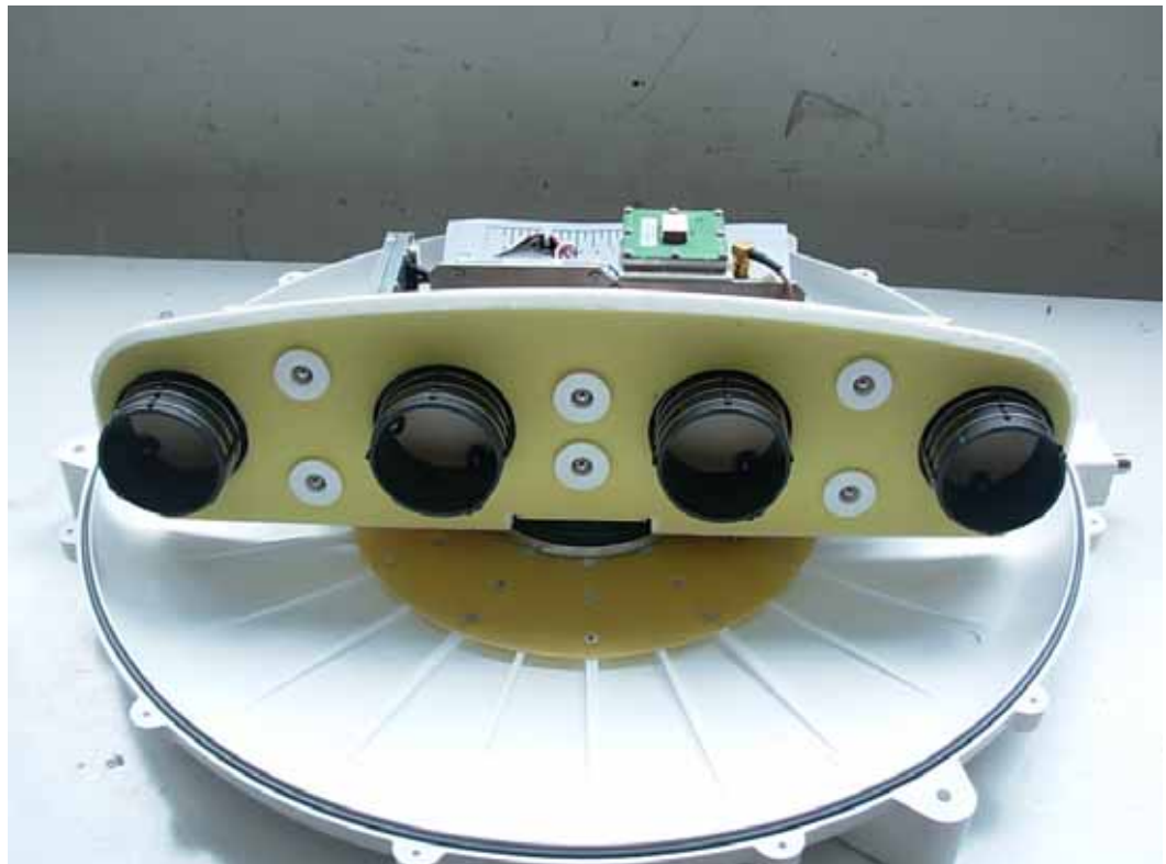
FIGURE 24 LAND MOBILE TERMINAL (M/N: 9350-10) SATELLITE ANTENNA – INSIDE FRONT VIEW
