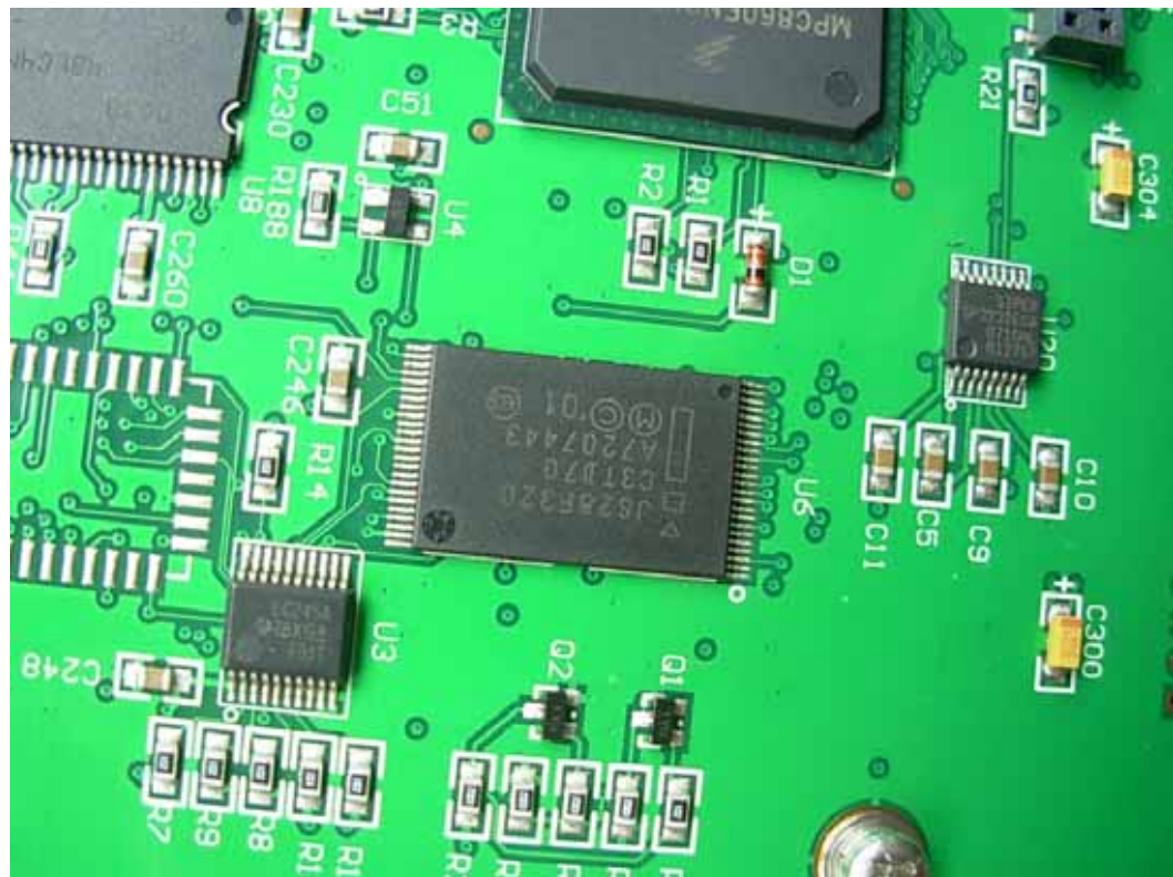
FIGURE 9 LAND MOBILE TERMINAL (M/N: 9350-10) MAIN BOARD – IC 5
