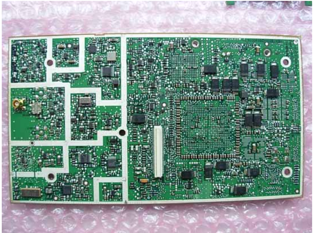
FIGURE 15 LAND MOBILE TERMINAL (M/N: 9350-10) MAIN BOARD - MODULE – SIDE 2
