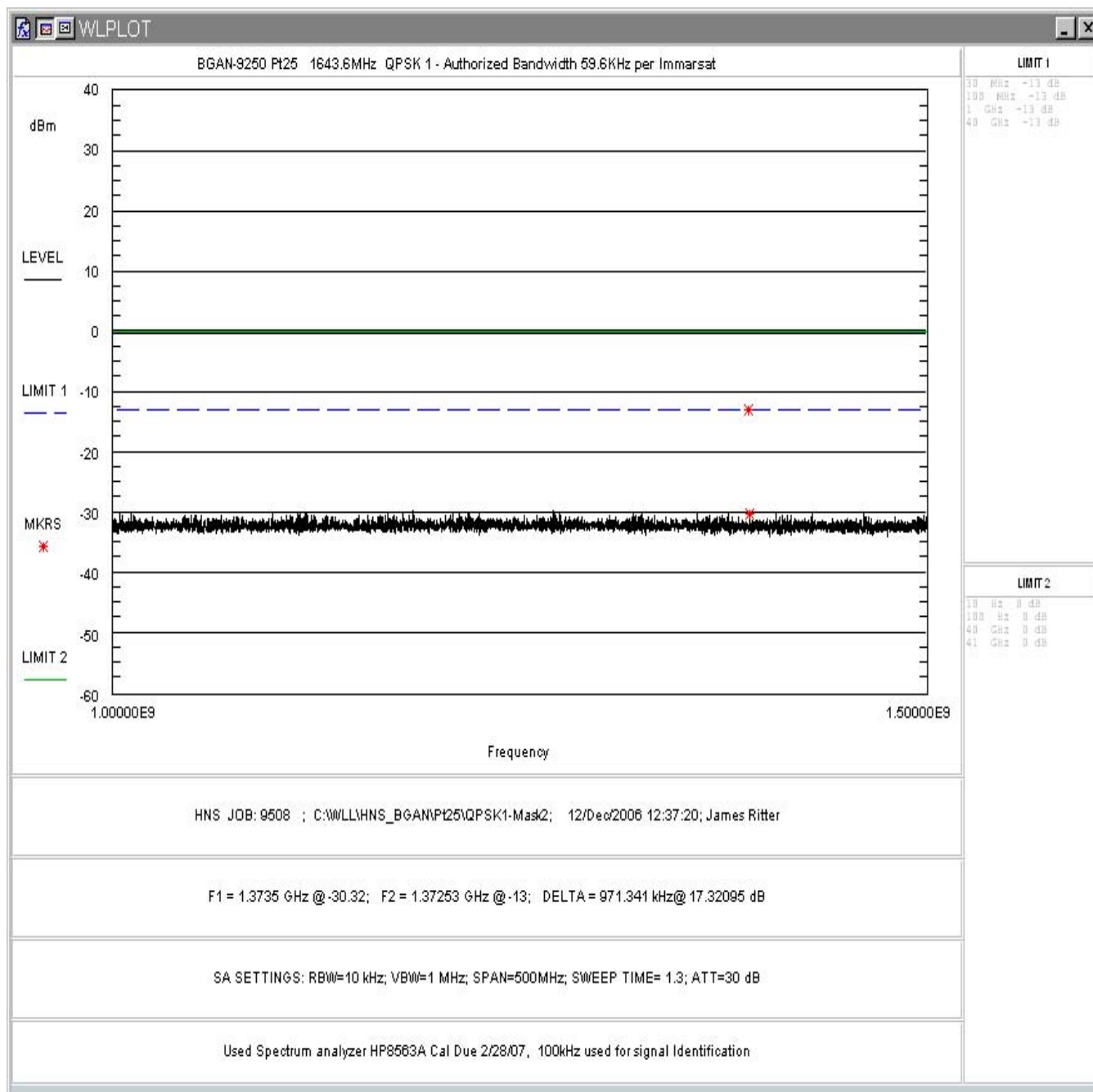
Figure 49: FCC Part 25 Conducted Spurious Emissions Data, QPSK 1 1000 – 1500MHz
