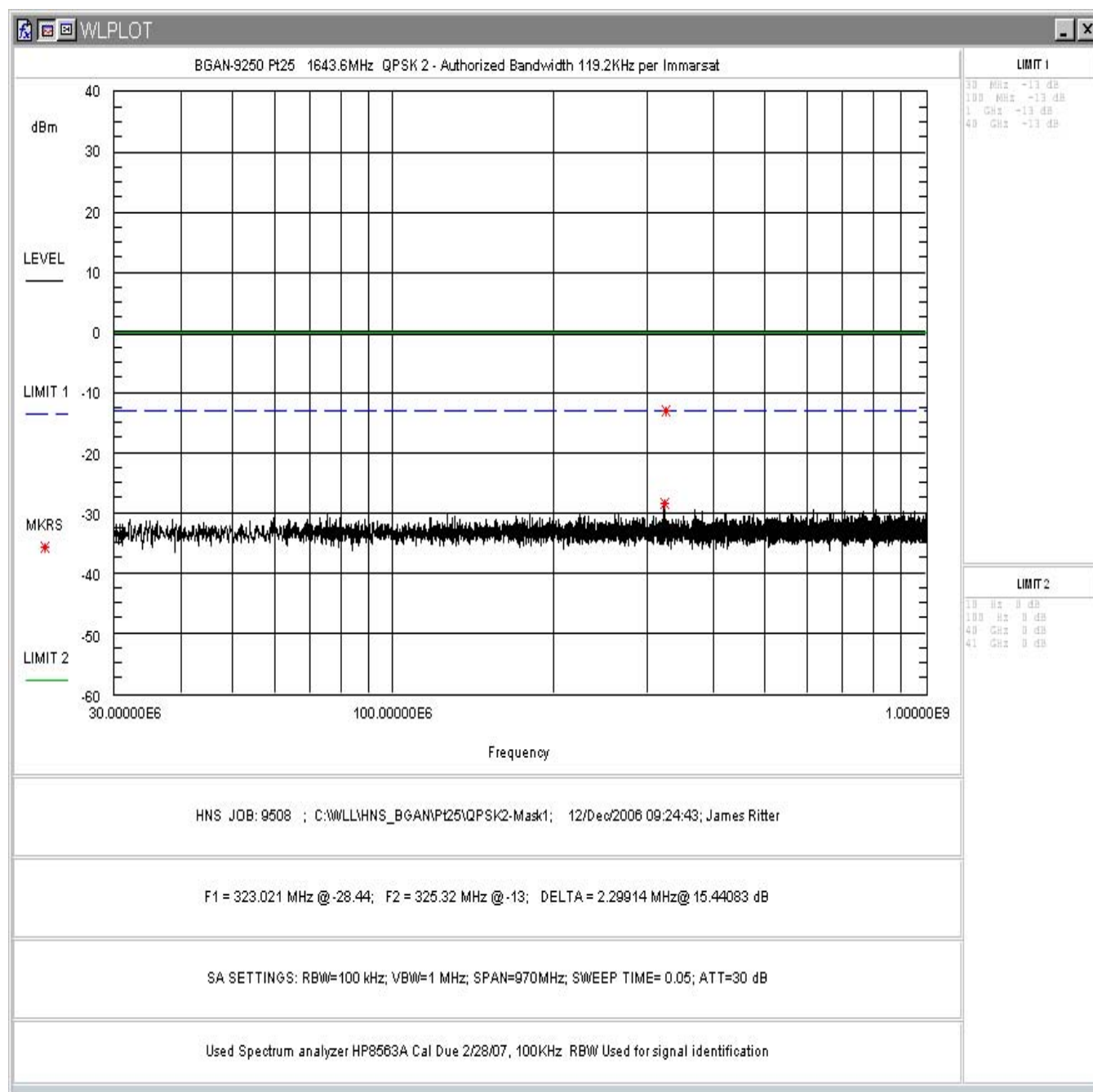
Figure 56: FCC Part 25 Conducted Spurious Emissions Data, QPSK 2 30MHz - 1000MHz
