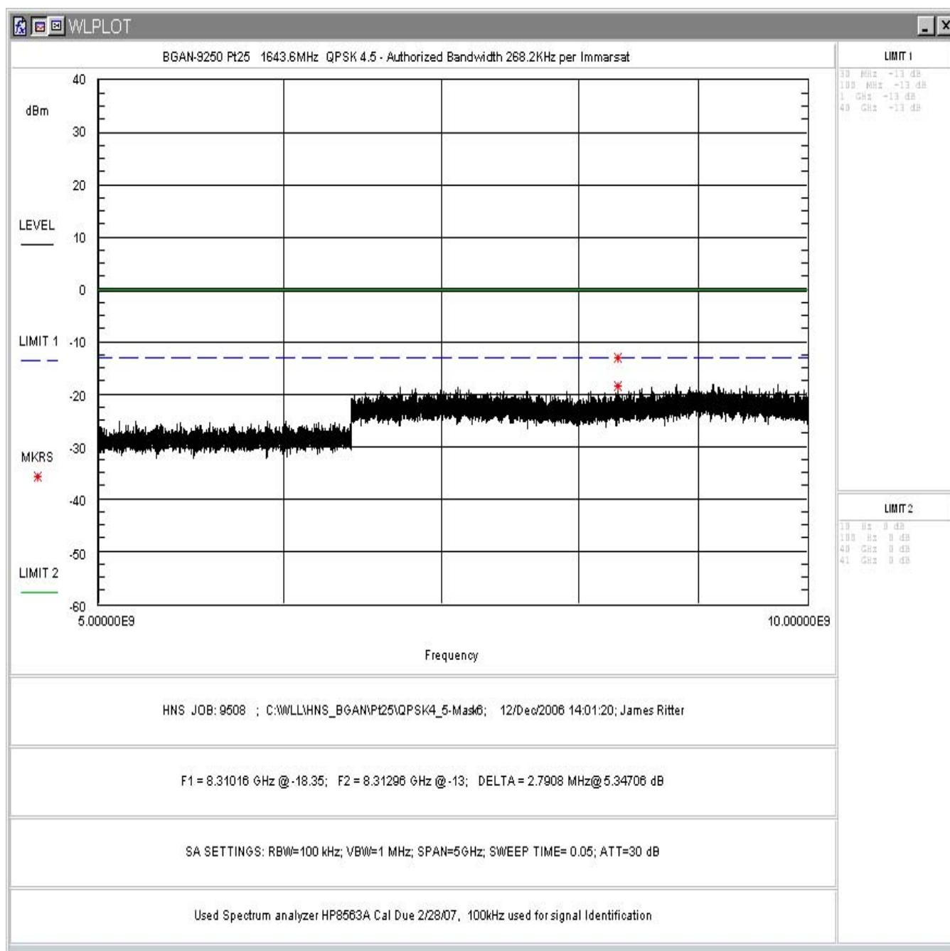
Figure 69: FCC Part 25 Conducted Spurious Emissions Data, QPSK 4.5 5 – 10GHz
