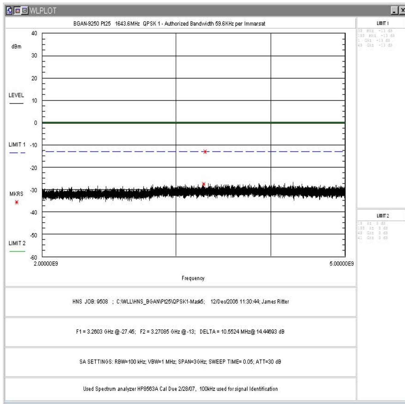
Figure 52: FCC Part 25 Conducted Spurious Emissions Data, QPSK 1 2 – 5GHz
