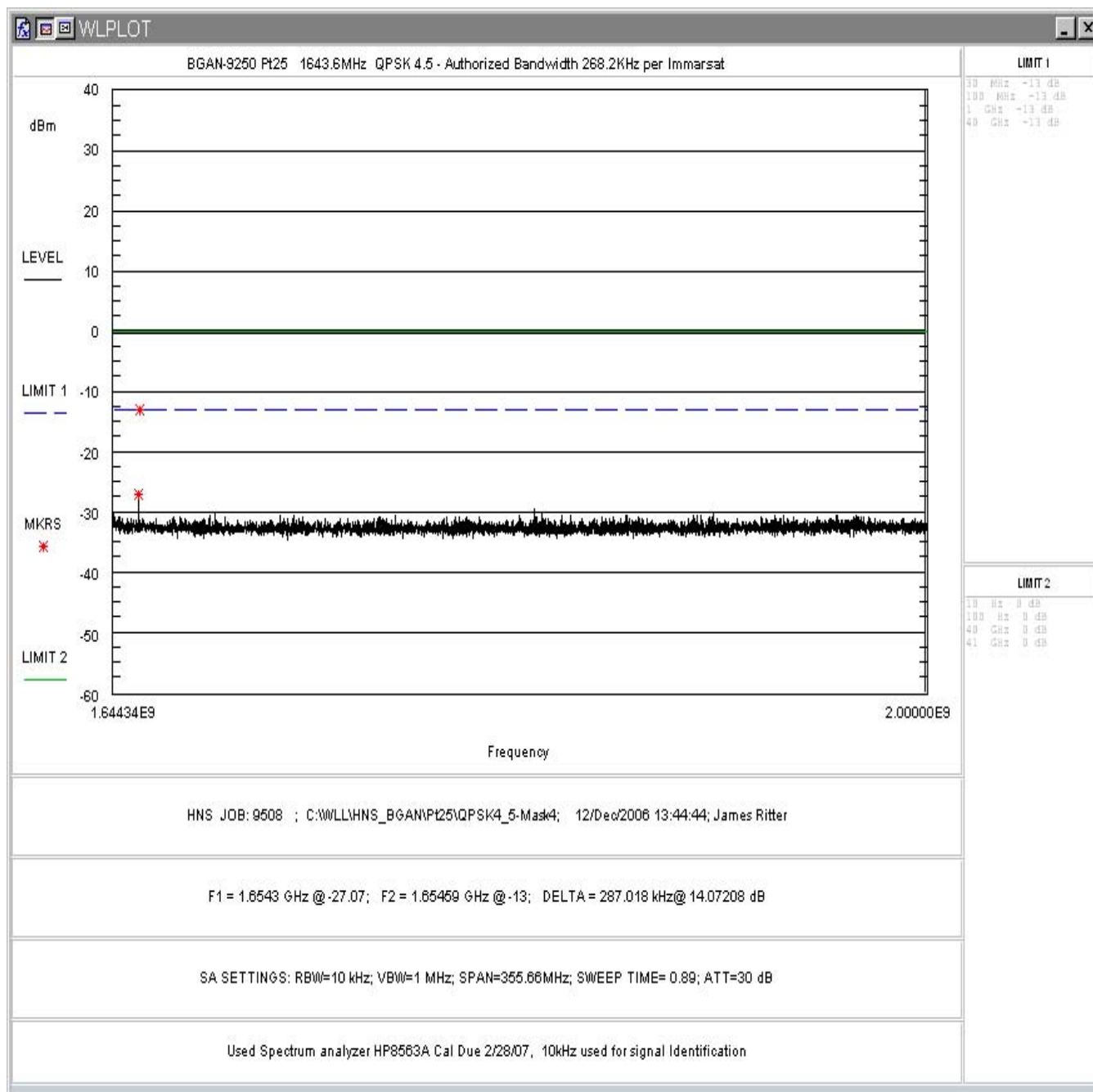
Figure 67: FCC Part 25 Conducted Spurious Emissions Data, QPSK 4.5 1643MHz – 2GHz
