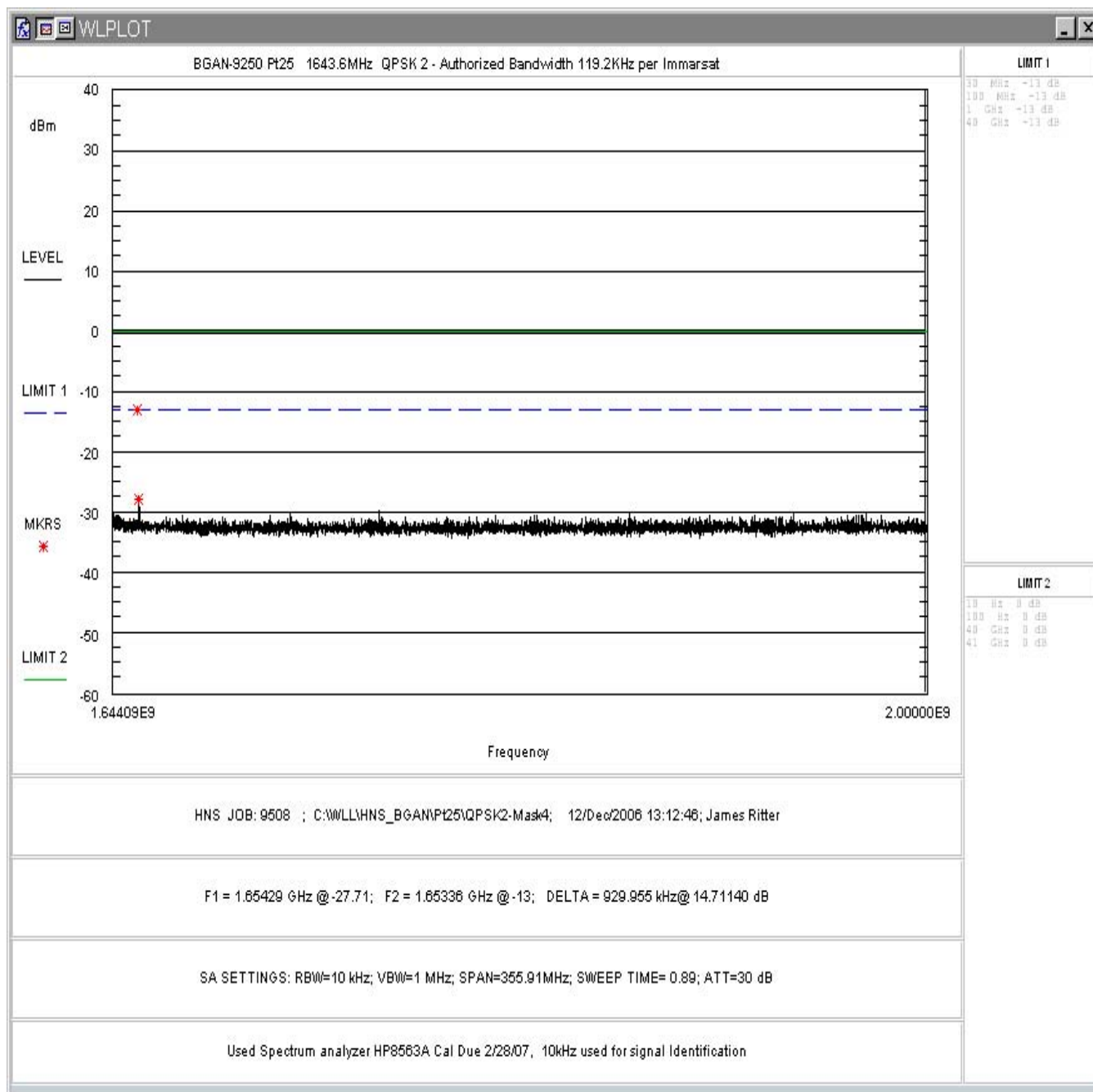
Figure 59: FCC Part 25 Conducted Spurious Emissions Data, QPSK 2 1 1643MHz – 2GHz
