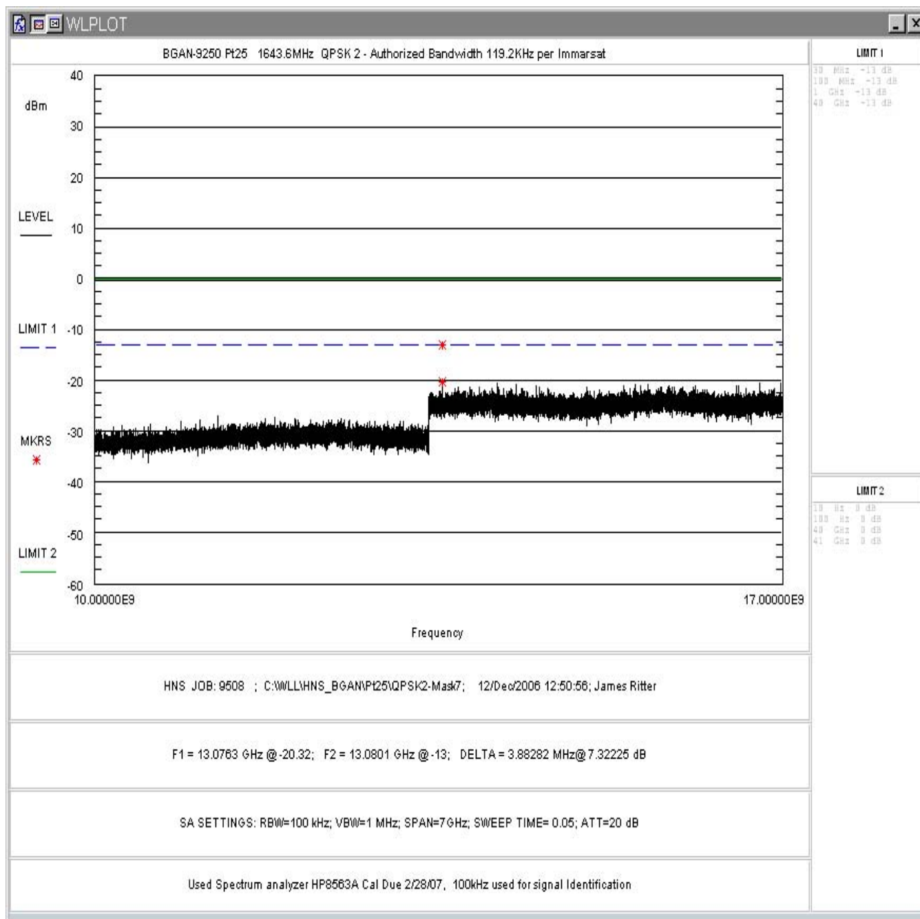
Figure 62: FCC Part 25 Conducted Spurious Emissions Data, QPSK 2 10 – 17GHz
