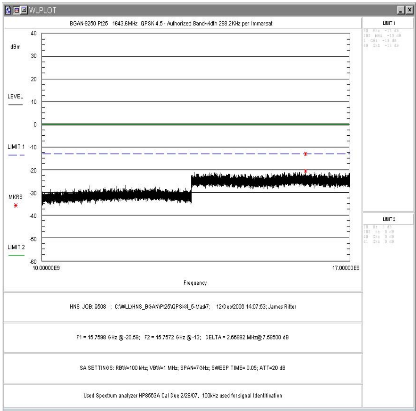
Figure 70: FCC Part 25 Conducted Spurious Emissions Data, QPSK 4.5 10 – 17GHz
