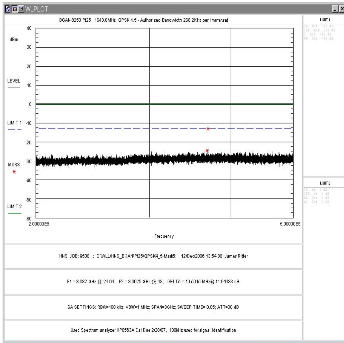
Figure 68: FCC Part 25 Conducted Spurious Emissions Data, QPSK 4.5 2 – 5GHz
