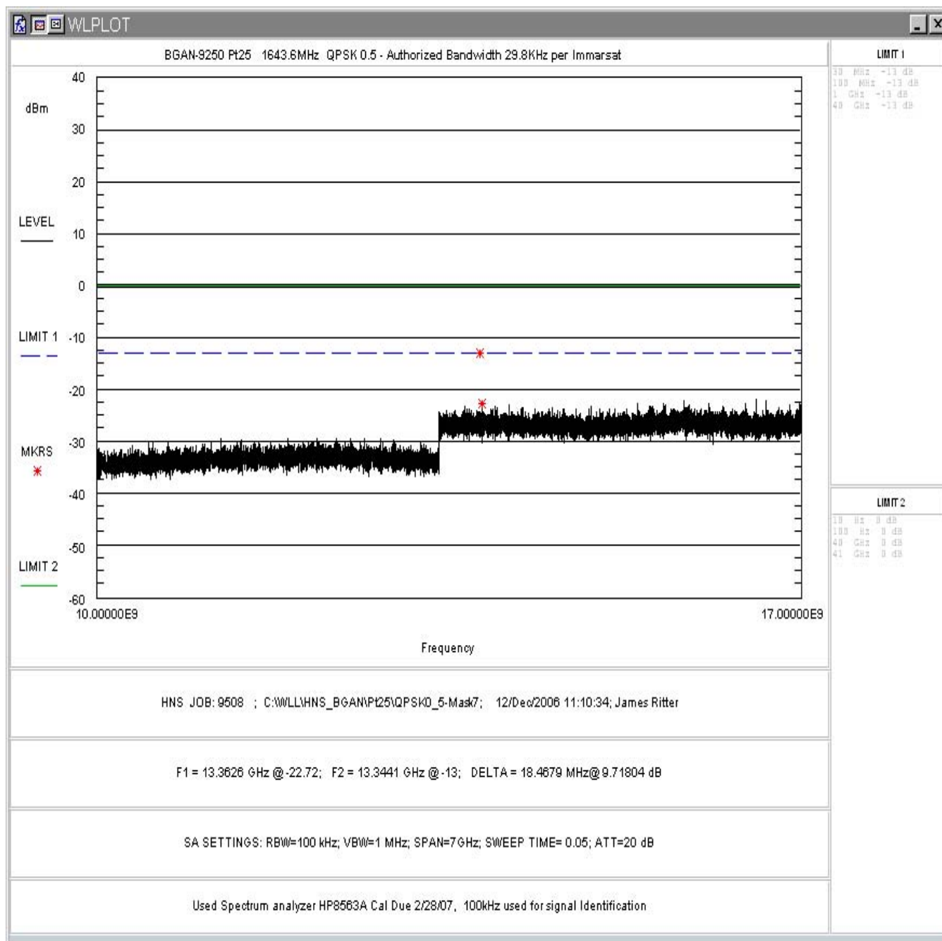
Figure 46: FCC Part 25 Conducted Spurious Emissions Data, QPSK 0.5 10 – 17GHz
