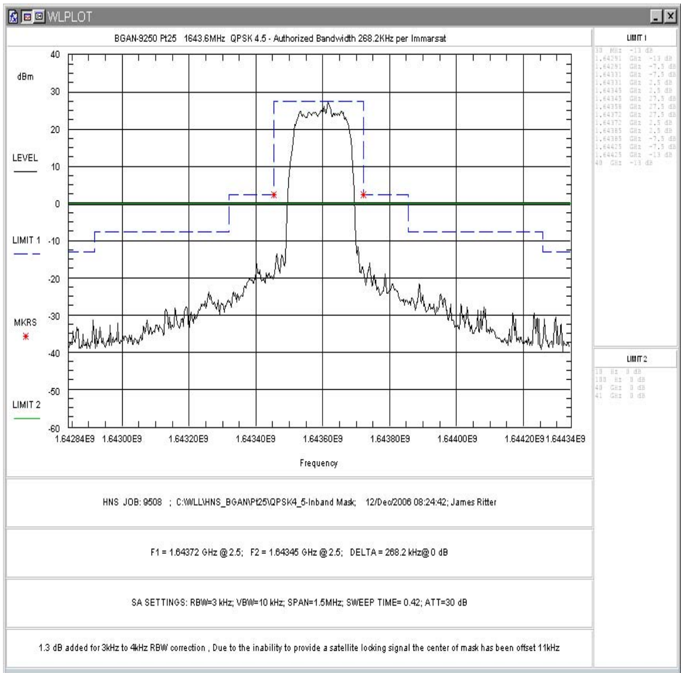
Figure 63: FCC Part 25 QPSK 4.5 Emission Mask
