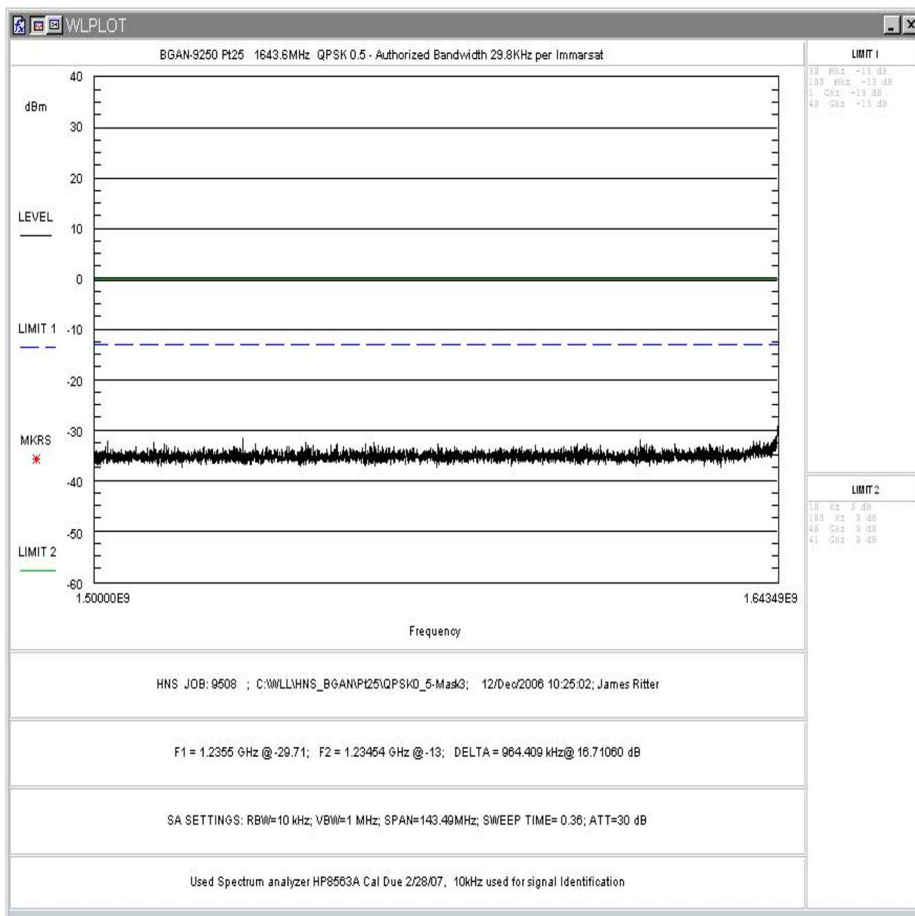
Figure 42: FCC Part 25 Conducted Spurious Emissions Data, QPSK 0.5 1500 – 1643MHz
