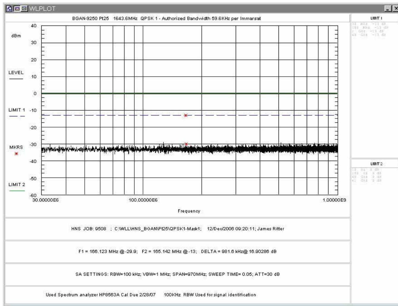
Figure 48: FCC Part 25 Conducted Spurious Emissions Data, QPSK 1 30MHz - 1000MHz
