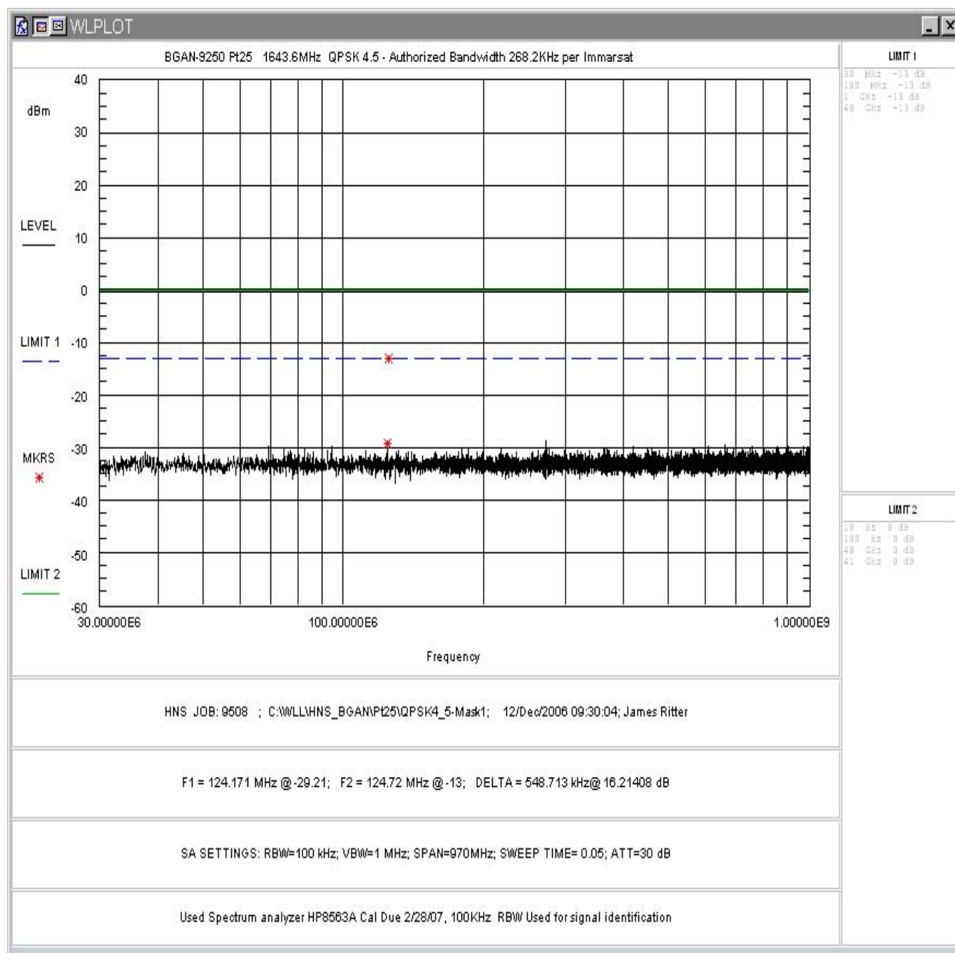
Figure 64: FCC Part 25 Conducted Spurious Emissions Data, QPSK 4.5 30MHz - 1000MHz
