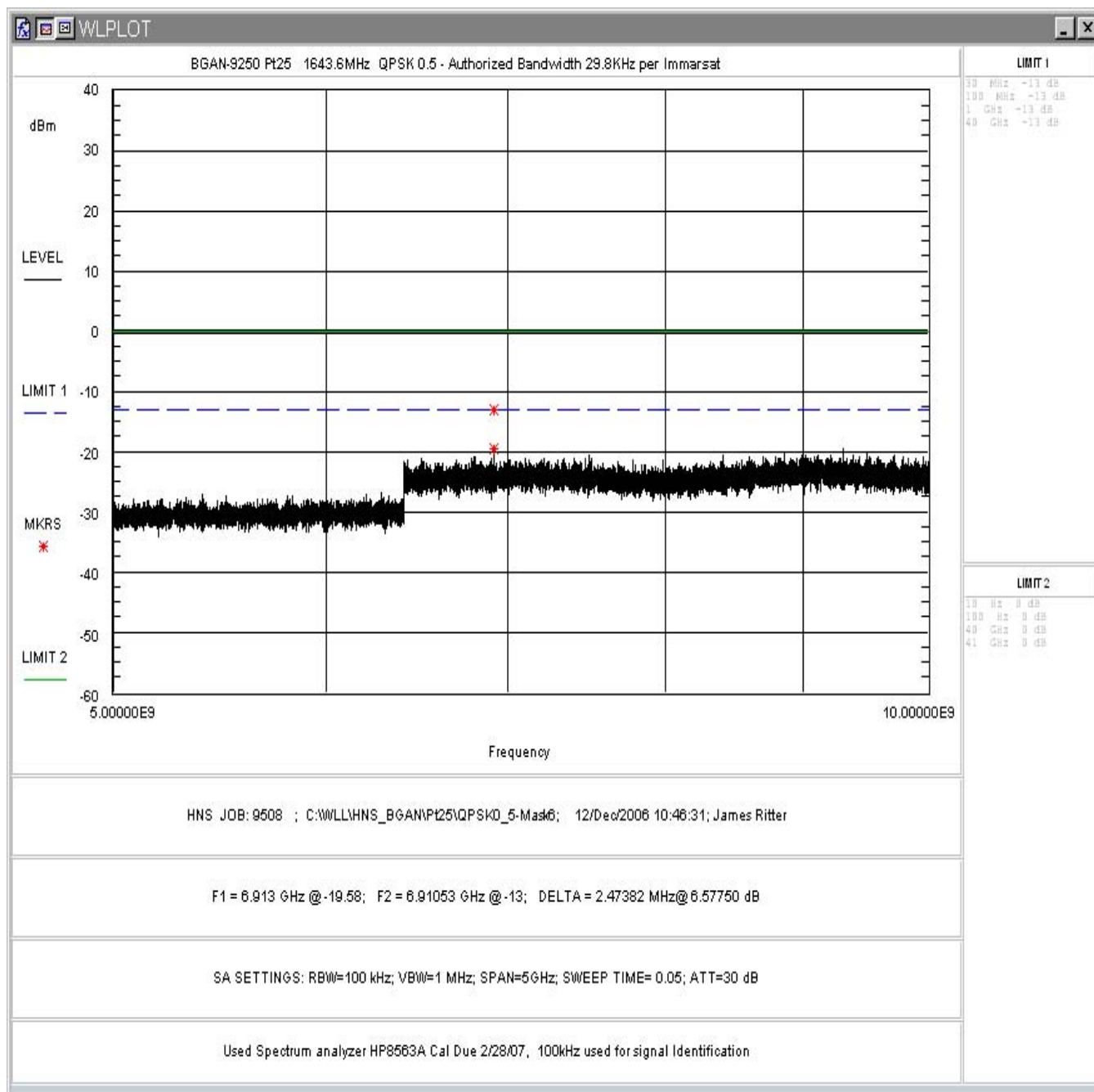
Figure 45: FCC Part 25 Conducted Spurious Emissions Data, QPSK 0.5 5 – 10GHz
