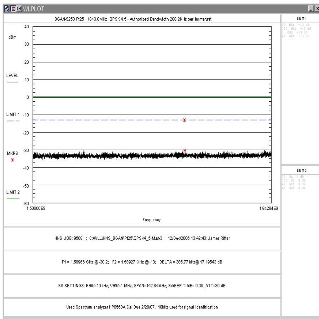
Figure 66: FCC Part 25 Conducted Spurious Emissions Data, QPSK 4.5 1500 – 1643MHz
