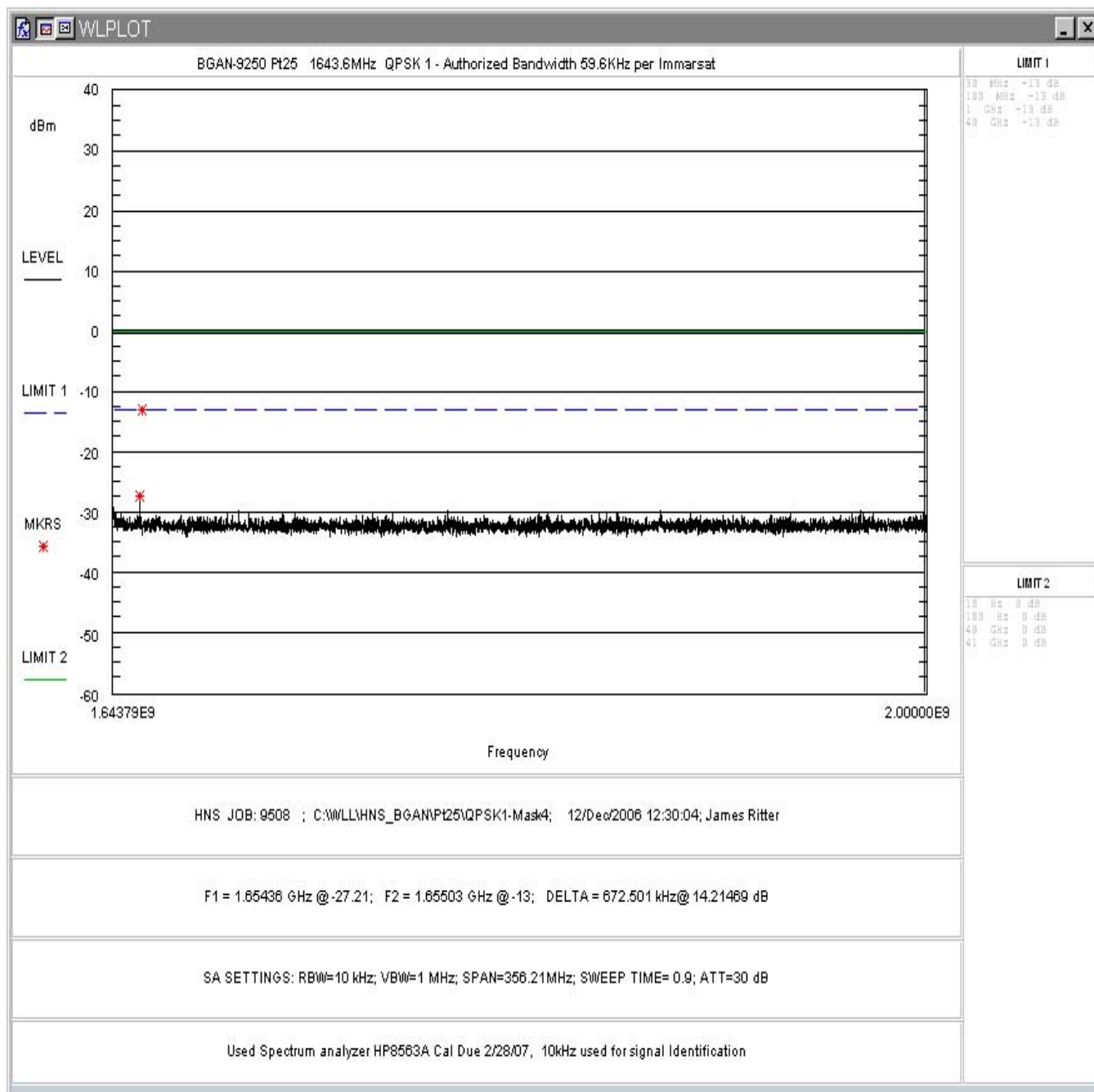
Figure 51: FCC Part 25 Conducted Spurious Emissions Data, QPSK 1 1643MHz – 2GHz
