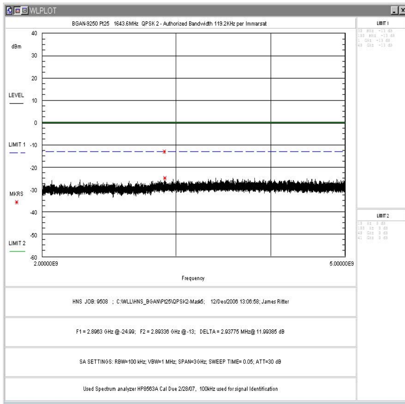
Figure 60: FCC Part 25 Conducted Spurious Emissions Data, QPSK 2 2 – 5GHz
