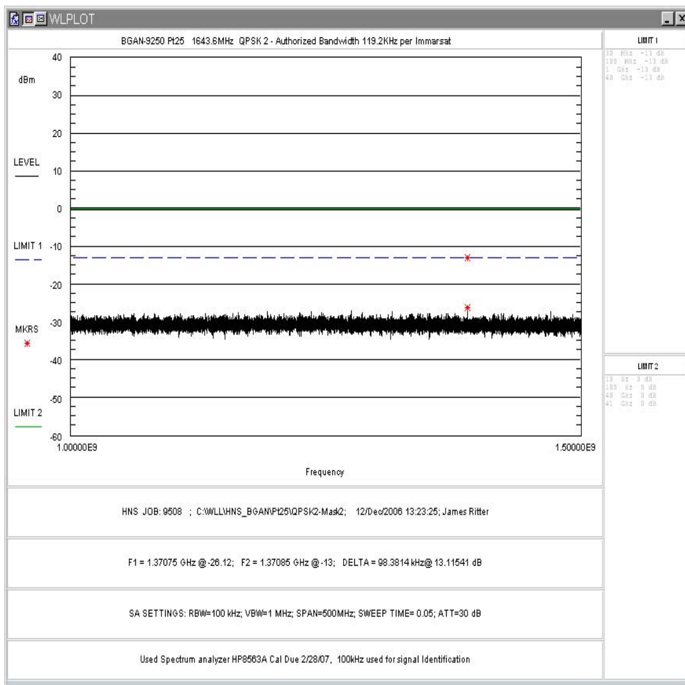
Figure 57: FCC Part 25 Conducted Spurious Emissions Data, QPSK 2 1000 – 1500MHz
