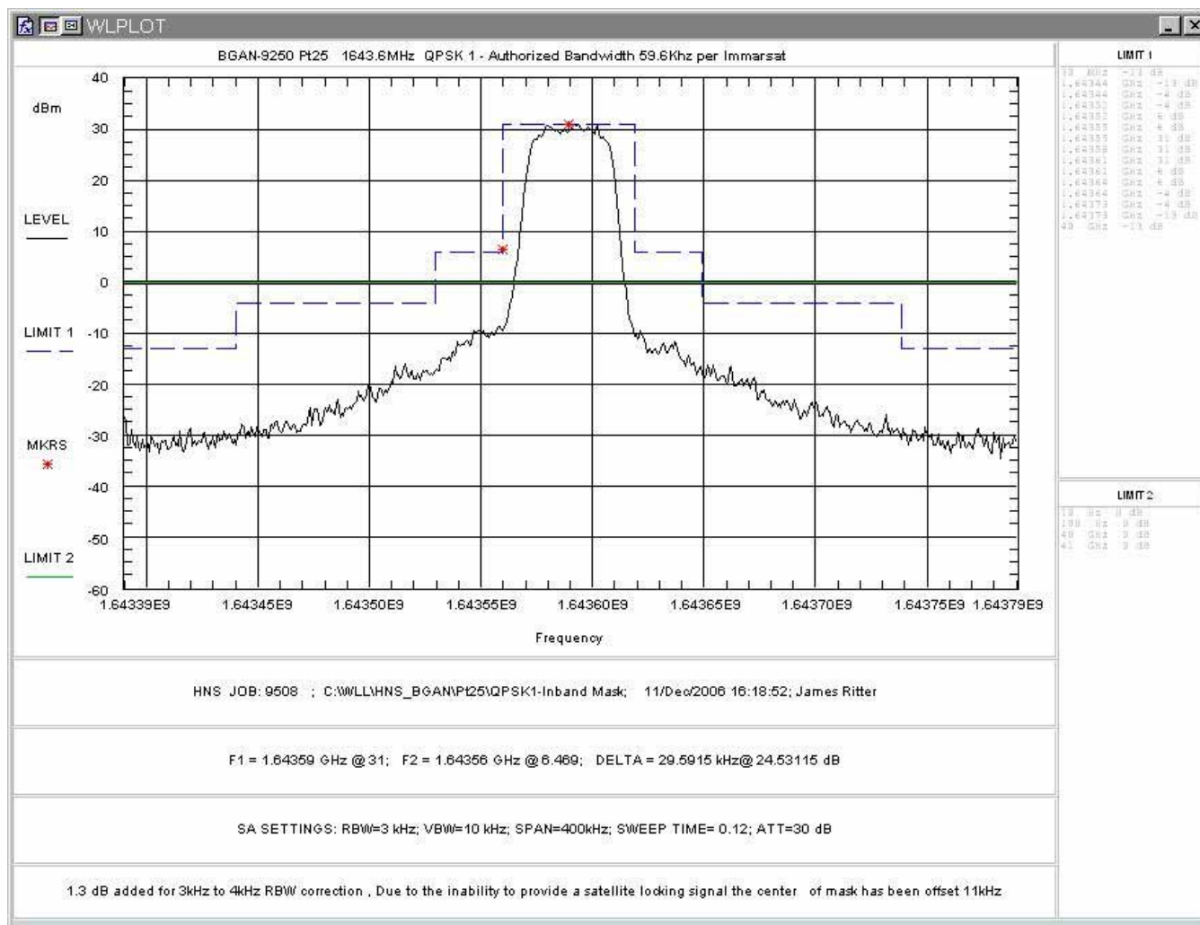
Figure 47: FCC Part 25 QPSK 1 Emission Mask
