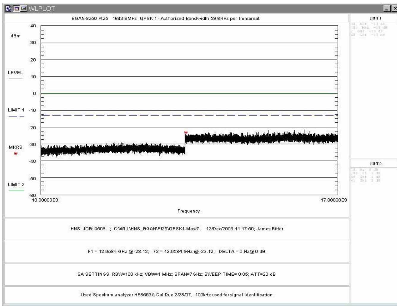
Figure 54: FCC Part 25 Conducted Spurious Emissions Data, QPSK 1 10 – 17GHz
