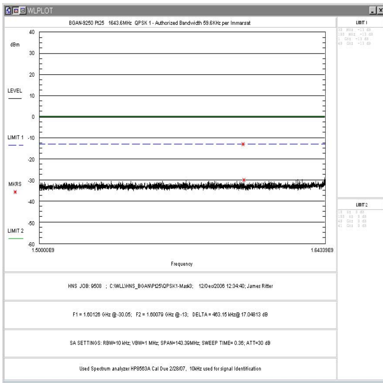
Figure 50: FCC Part 25 Conducted Spurious Emissions Data, QPSK 1 1500 – 1643MHz
