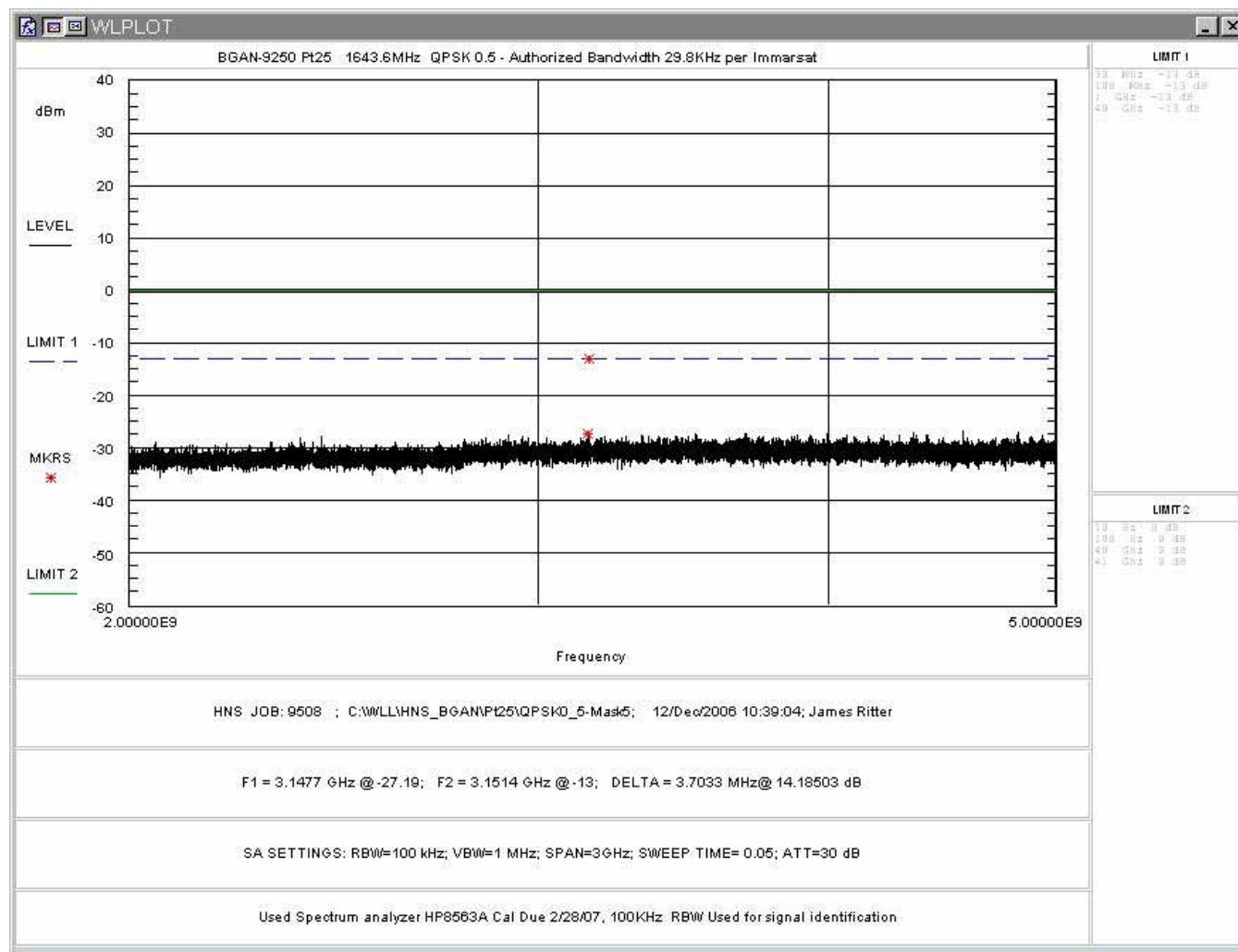
Figure 44: FCC Part 25 Conducted Spurious Emissions Data, QPSK 0.5 2 – 5GHz
