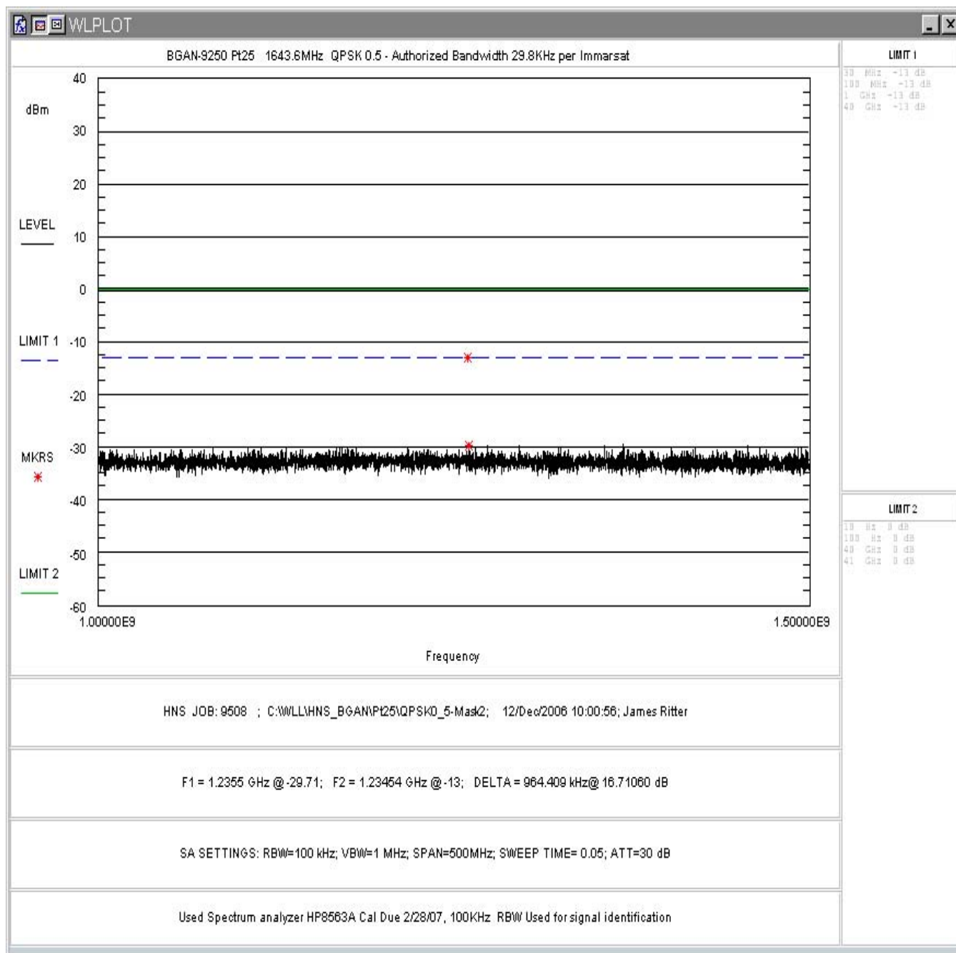
Figure 41: FCC Part 25 Conducted Spurious Emissions Data, QPSK 0.5 1000 – 1500MHz
