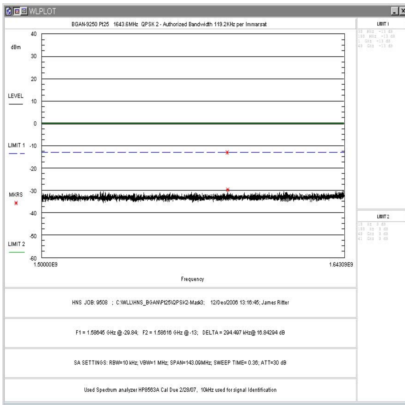
Figure 58: FCC Part 25 Conducted Spurious Emissions Data, QPSK 2 1500 – 1643MHz
