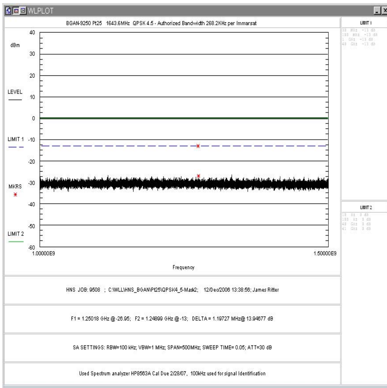
Figure 65: FCC Part 25 Conducted Spurious Emissions Data, QPSK 4.5 1000 – 1500MHz
