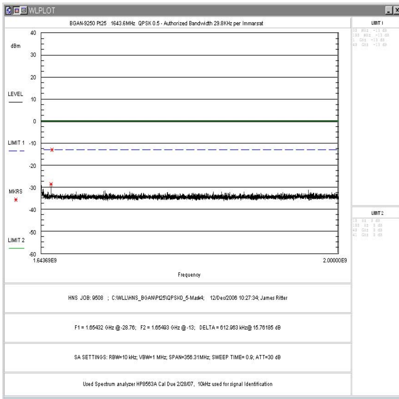
Figure 43: FCC Part 25 Conducted Spurious Emissions Data, QPSK 0.5 1643MHz – 2GHz
