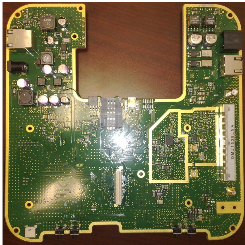
Interface Board - Underside
