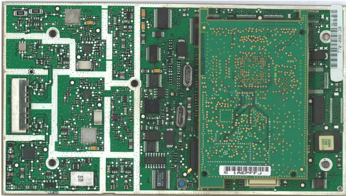
Core Module Topside – with WLAN Card installed
