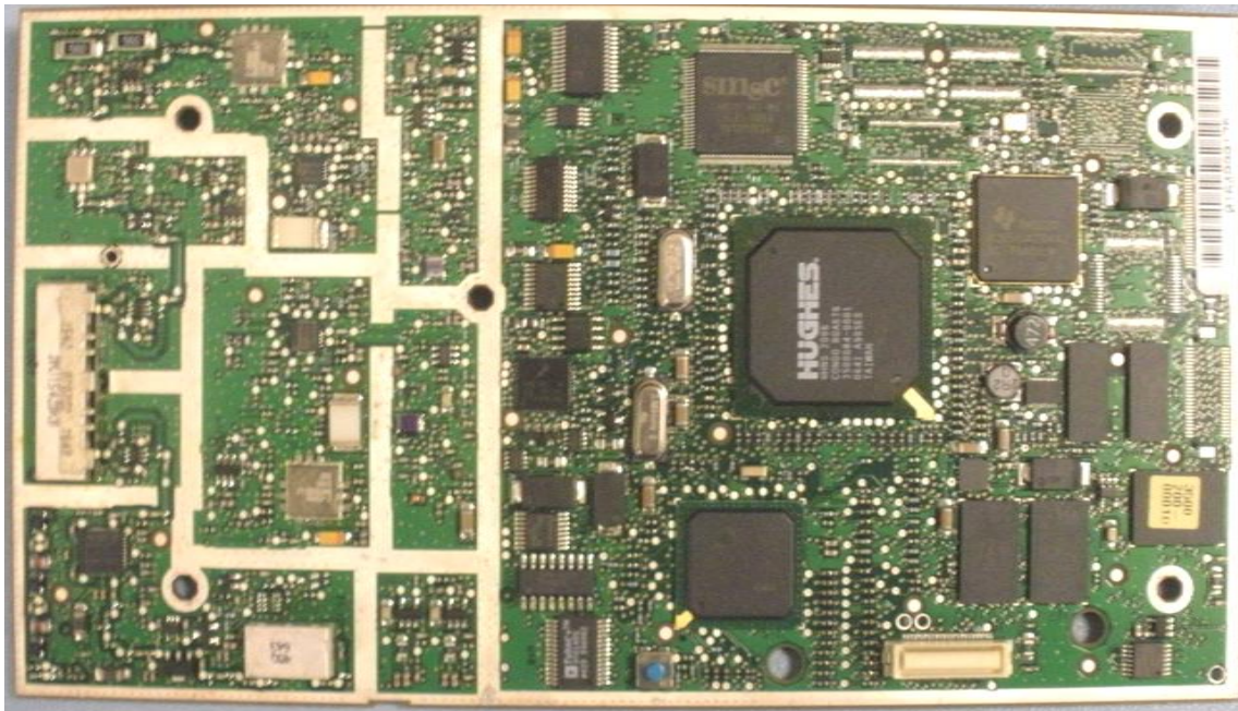
Core Module – Top side without WLAN card
