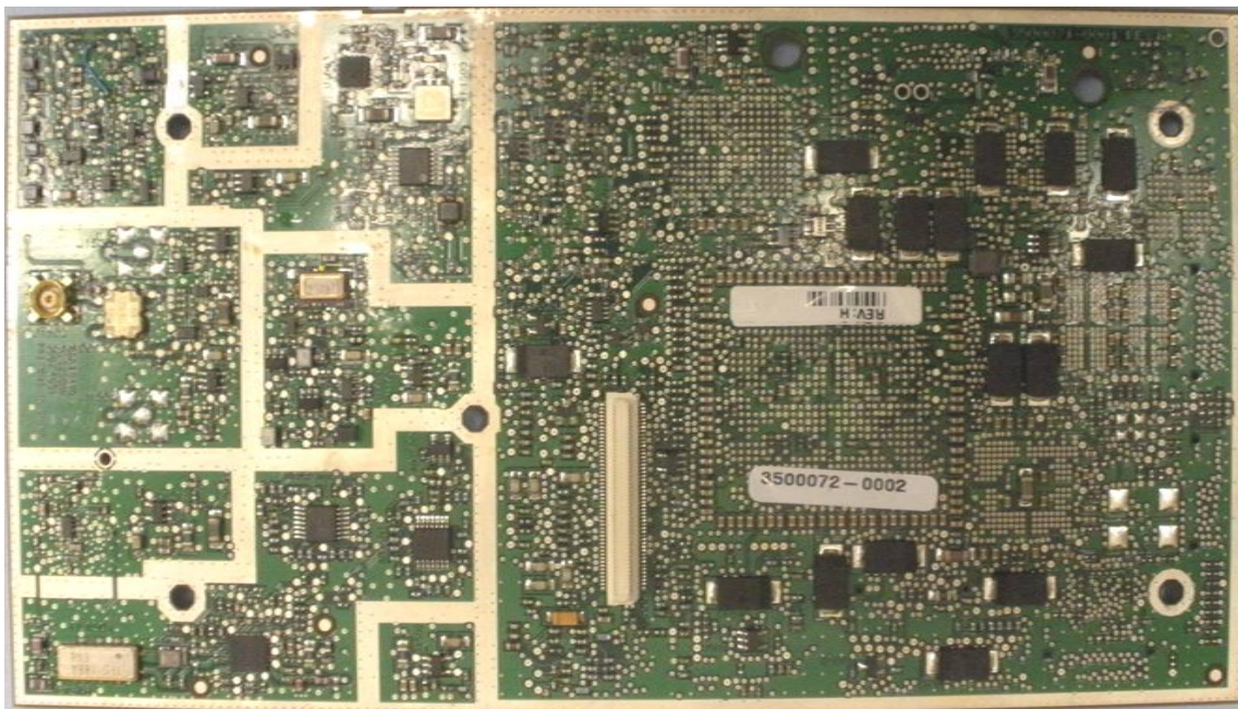
Core Module – Under side
