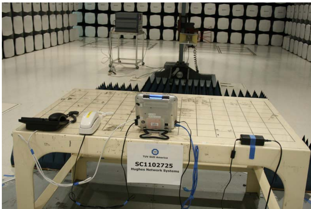
Radiated Emissions Test Setup (with AC adapter*)
