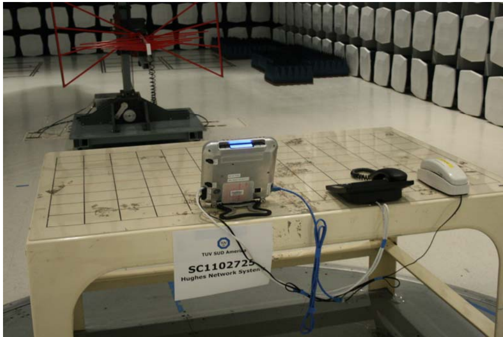
Radiated Emissions Test Setup (Freshly Charged Battery)
