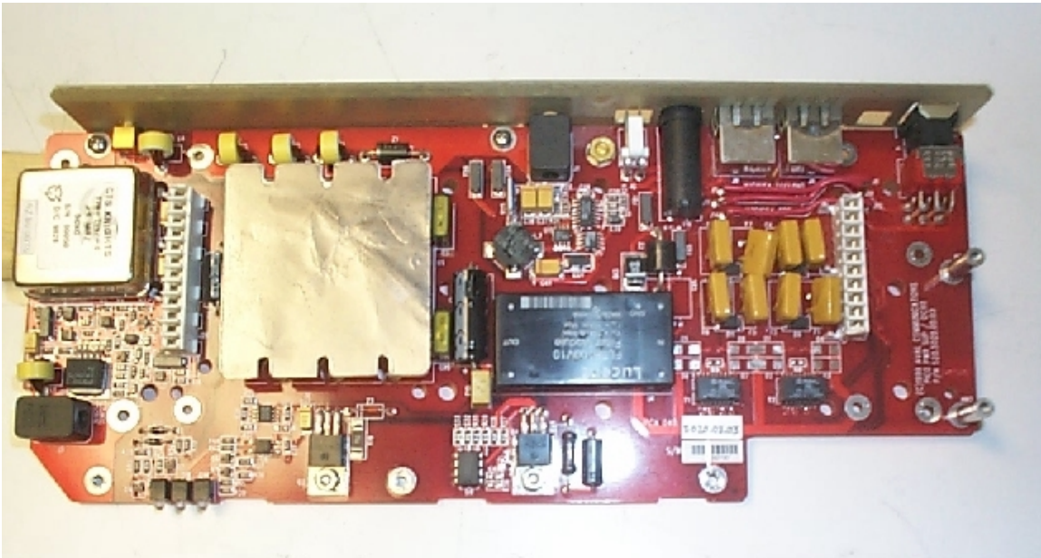
Figure 9.7: Picocell System Power Supply Module
