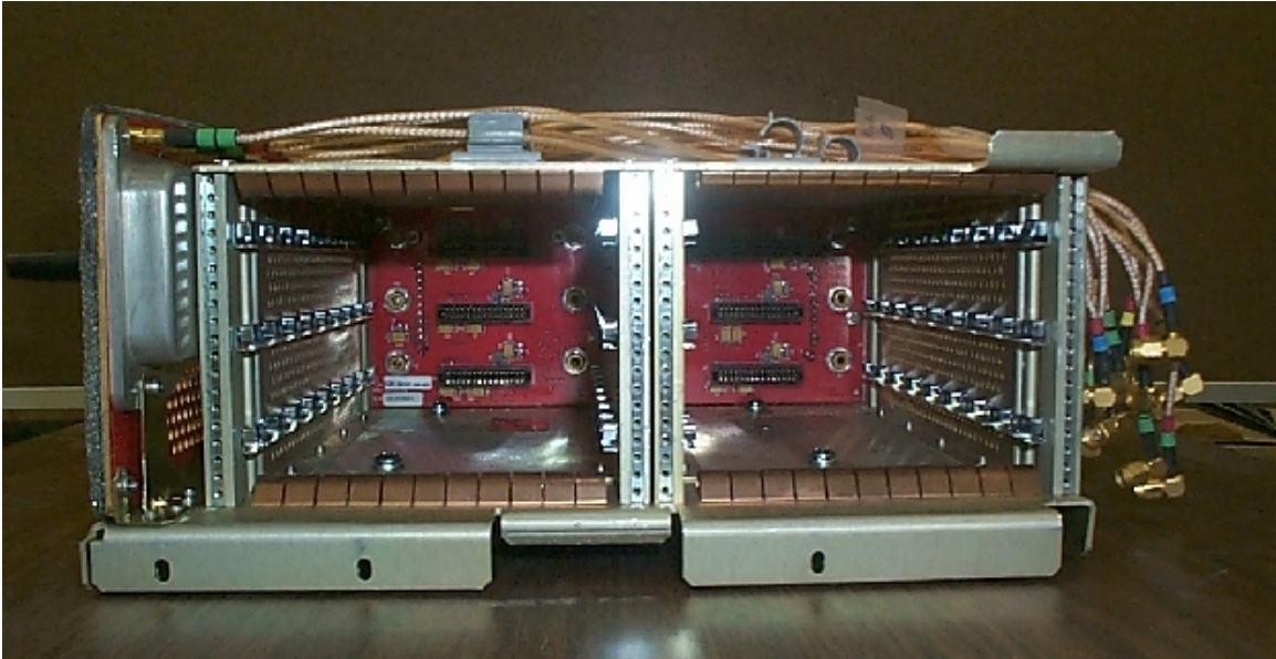
Figure 9.1: Picocell System Case with Backplane
