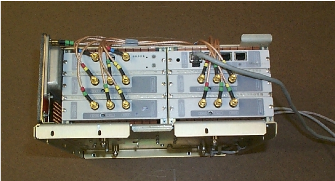
Figure 9.2: Picocell System with All Modules
