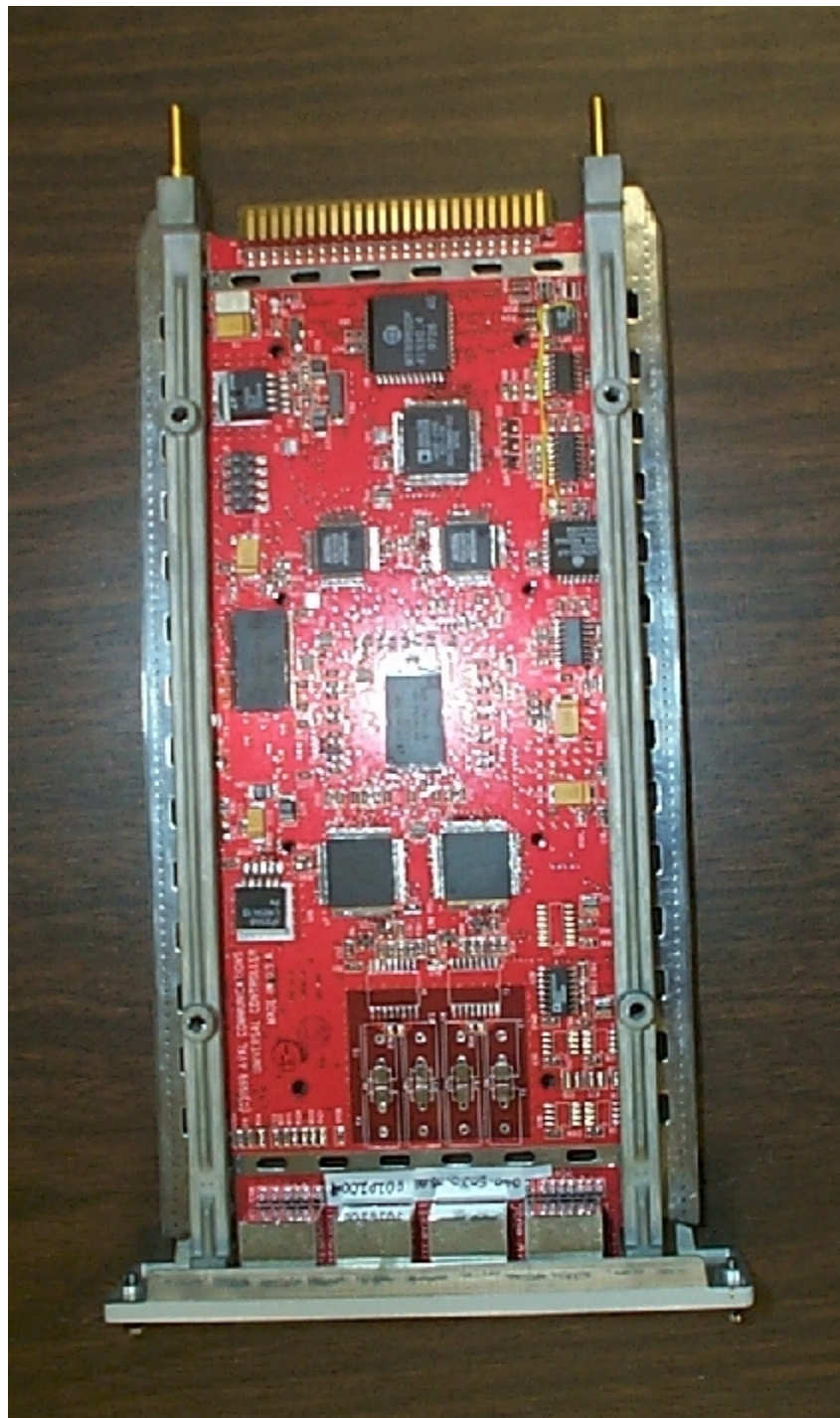
Figure 9.11: Picocell System Inside Front View of Controller Module
