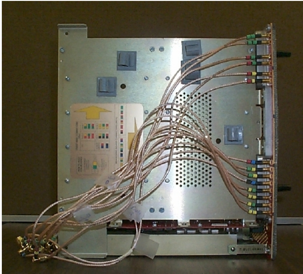
Figure 9.5: Picocell System Antenna Ports
