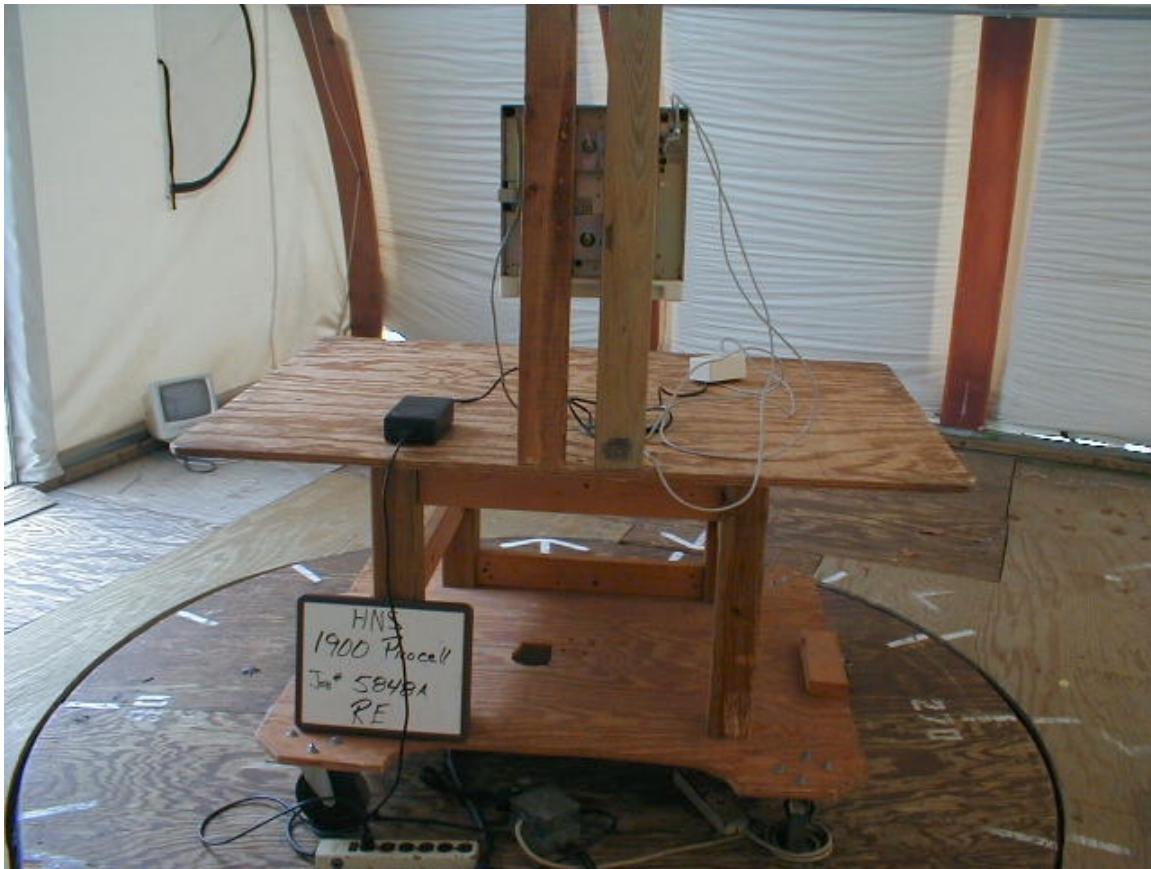
Figure 7.4: Radiated Emission OATS Test Setup
