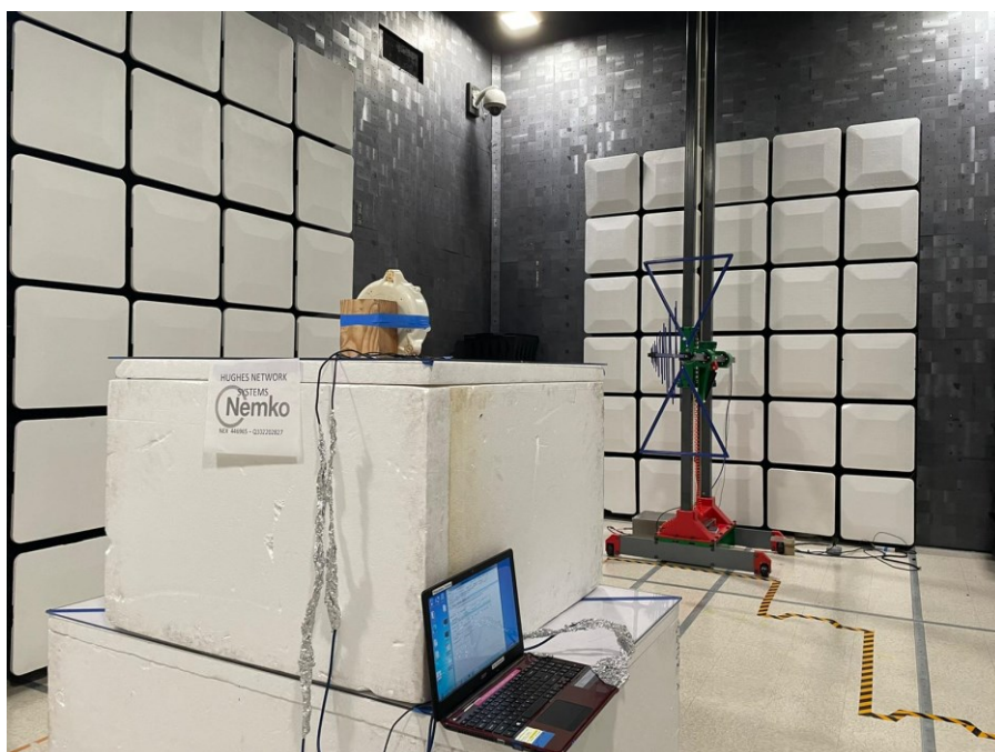
Figure 10 - Radiated emissions below 1 GHz (0.03 – 1 GHz), rear view.
