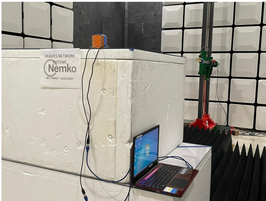
Figure 21 - Radiated emissions above 1 GHz (18 – 26 GHz), rear view.
