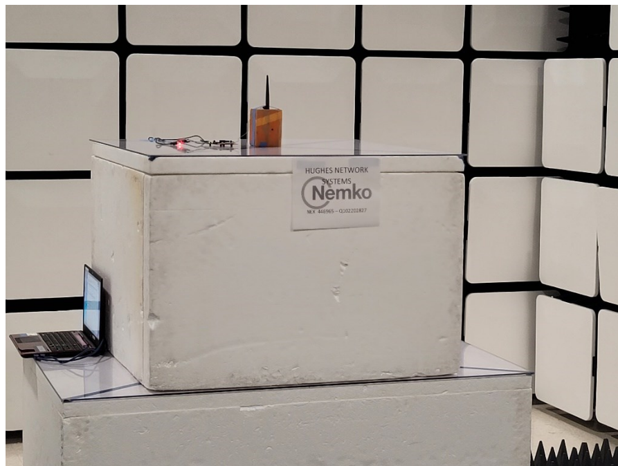
Figure 15 – Test setup.
