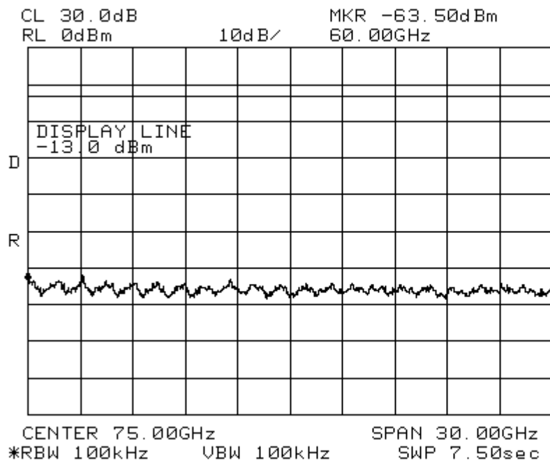
Figure 43 Conducted Emissions in 60-90GHz, for transmitting -12dBm QPSK on Channel 7A4
