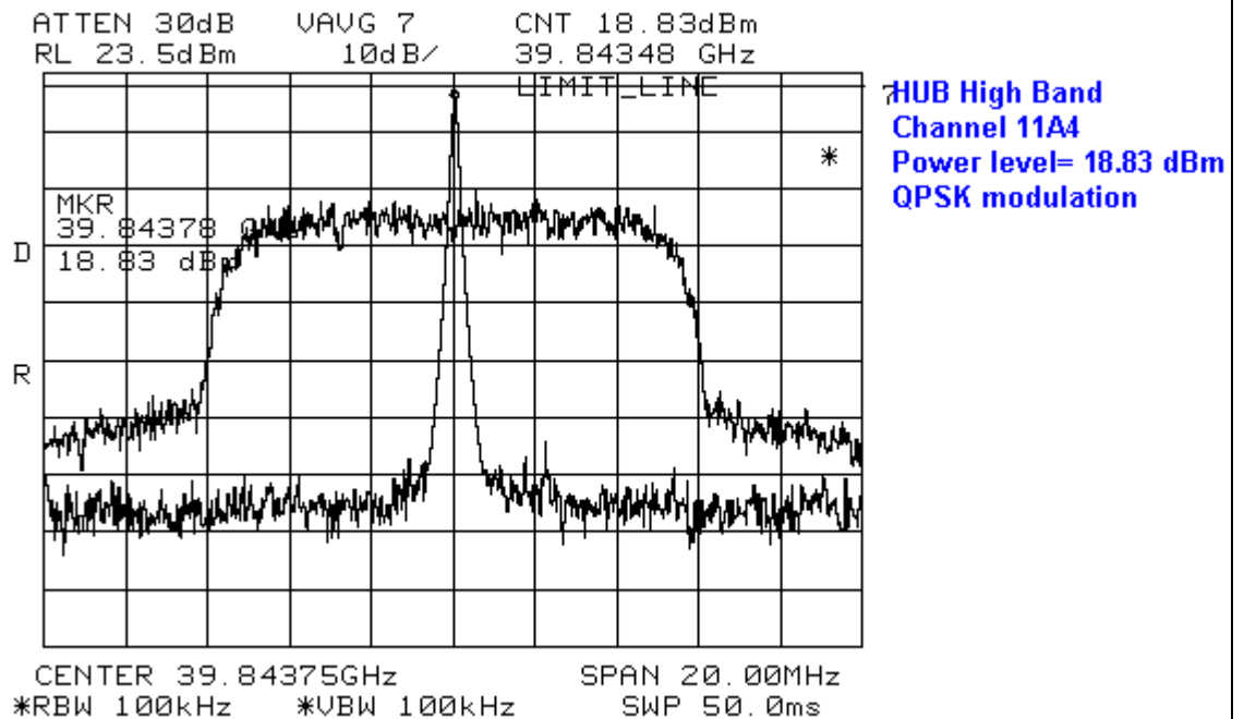
Figure 7 Output Power for QPSK modulation on Ch. 11A4
