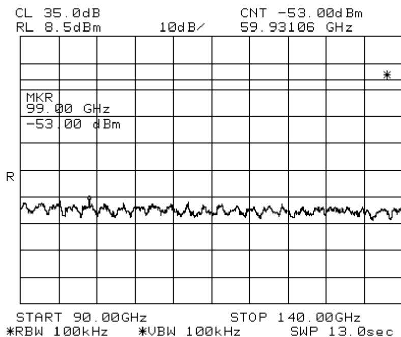
Figure 51 Radiated Emissions in 90-140GHz, VP, for transmitting 18dBm QPSK on Channel 14A4
