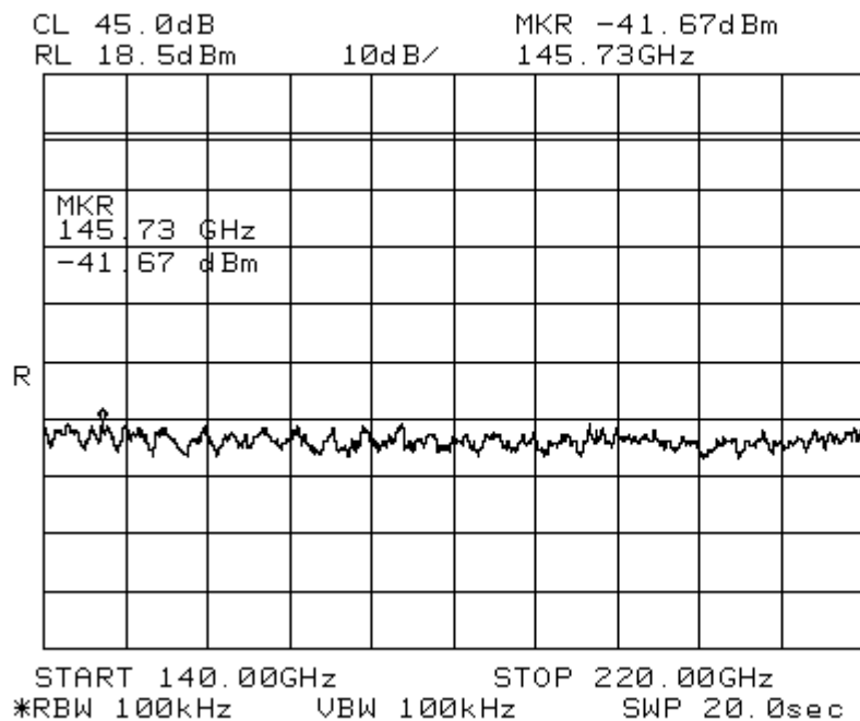
Figure 29 Conducted Emissions in 140-220GHz, for transmitting 18dBm QPSK on Channel 8A1
