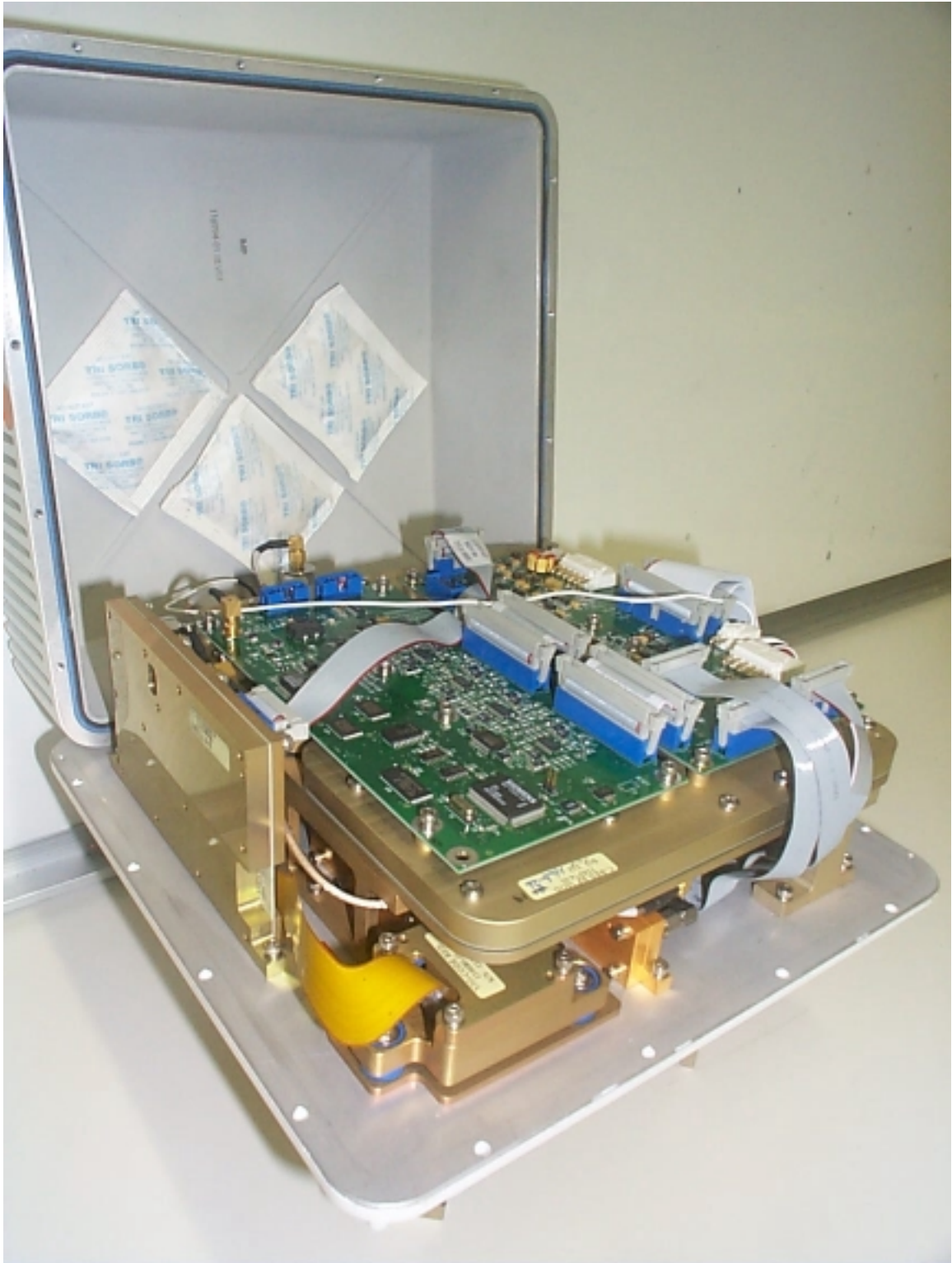
Figure 3 ODU HUB – Open cover
