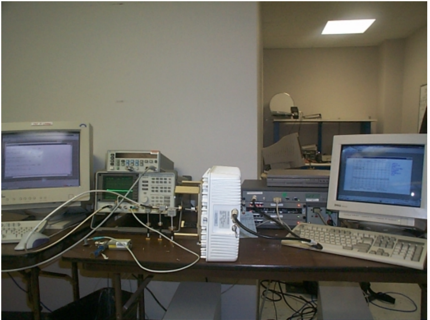
Figure 1 Conducted Spurious Emissions – Test setup
