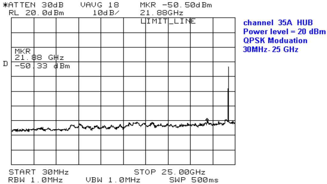
Figure 31: Conducted Emission for 30MHz-25Ghz band Tx Power=20dBm
