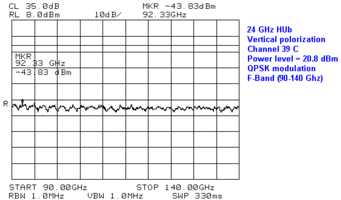
Figure 54 Radiated Emissions in 90-140GHz, VP, for transmitting 20dBm QPSK on Channel 39C
