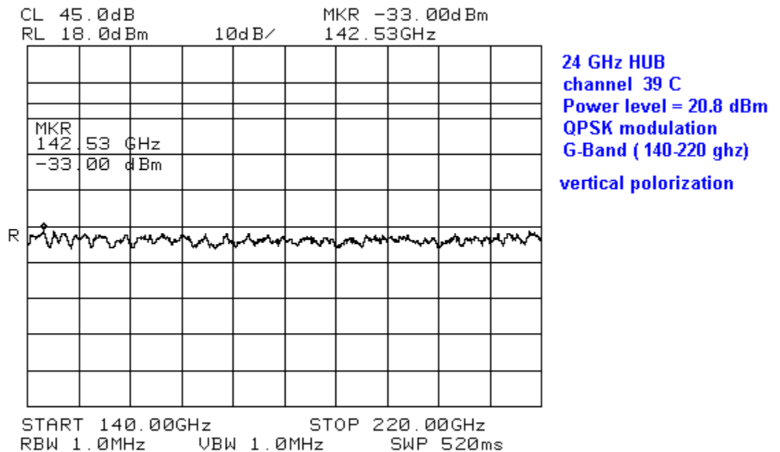
Figure 55 Radiated Emissions in 140-220GHz, VP, for transmitting 20dBm QPSK on Channel 39C
