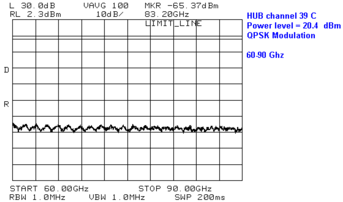
Figure 38 Conducted Emission 60-90Ghz band channel 39C Tx Power=20dBm
