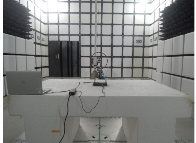
FCC_15_407_WLAN Radiated_Setup
