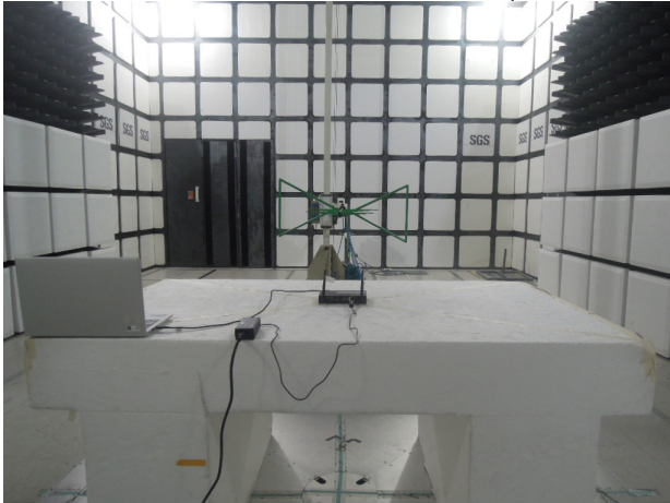
FCC_15_407_WLAN Radiated_Setup
