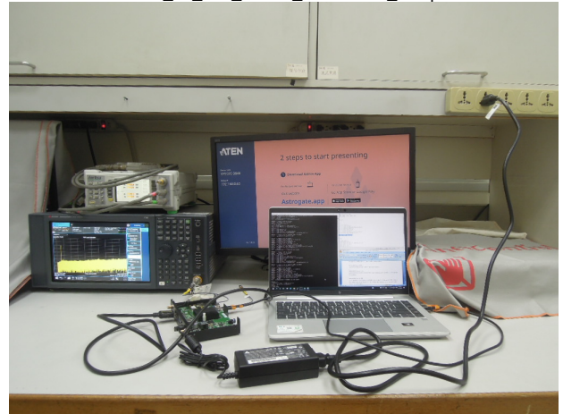
FCC_15_407_WLAN_Conducted_setup
