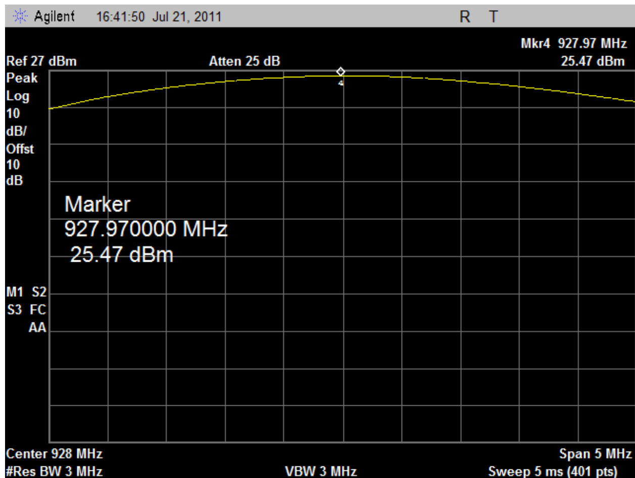
Plot 8 – Highest Channel – Output Power
