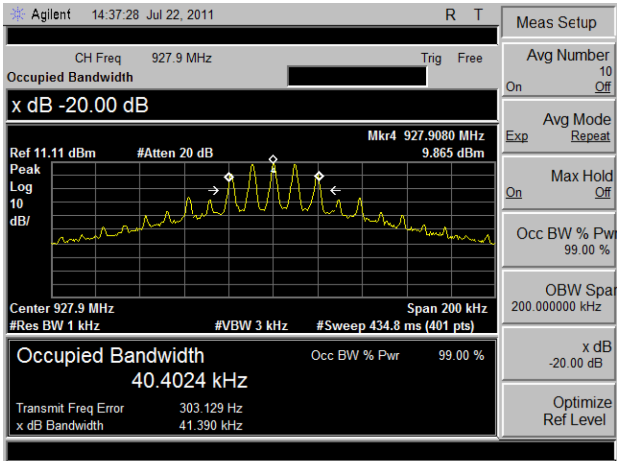
Plot 5 – Highest Channel – 20dB BW FM Modulation
