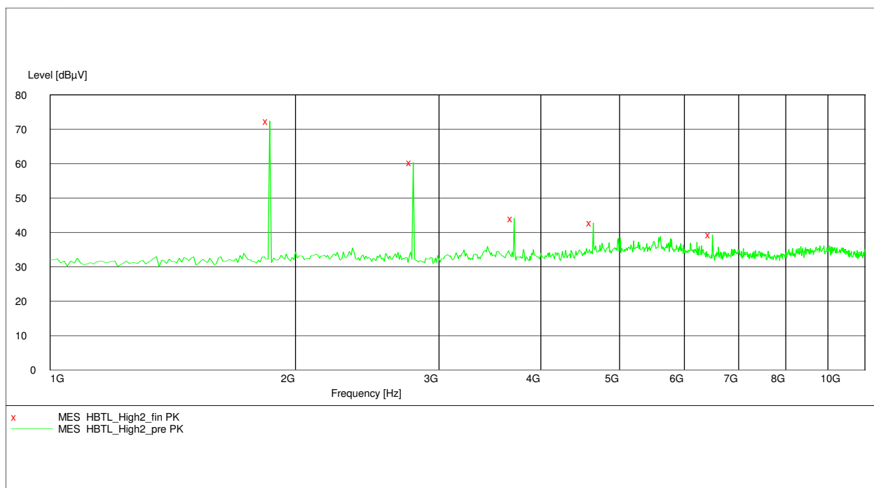
Plot 14 – Highest Channel (1GHz to 10GHz)
