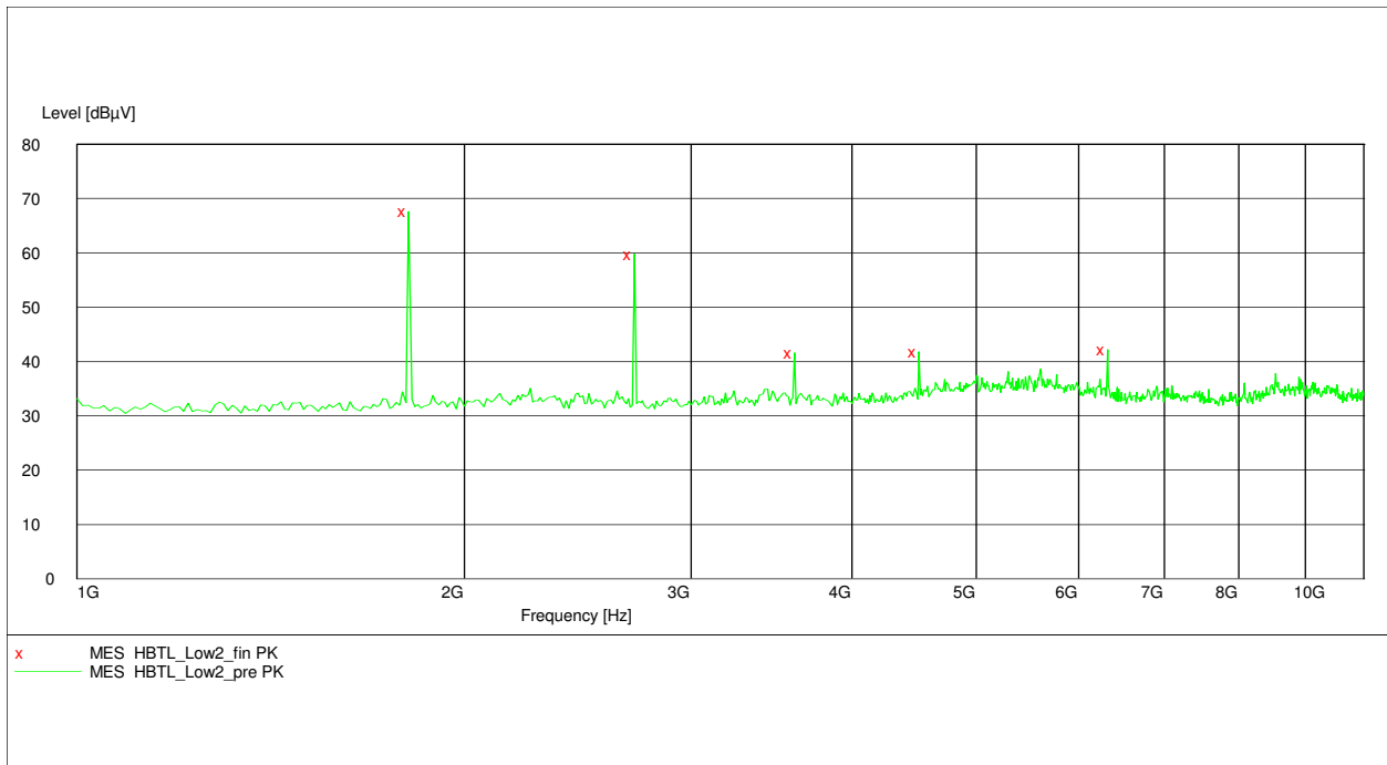
Plot 10 – Lowest Channel (1GHz to 10GHz)
