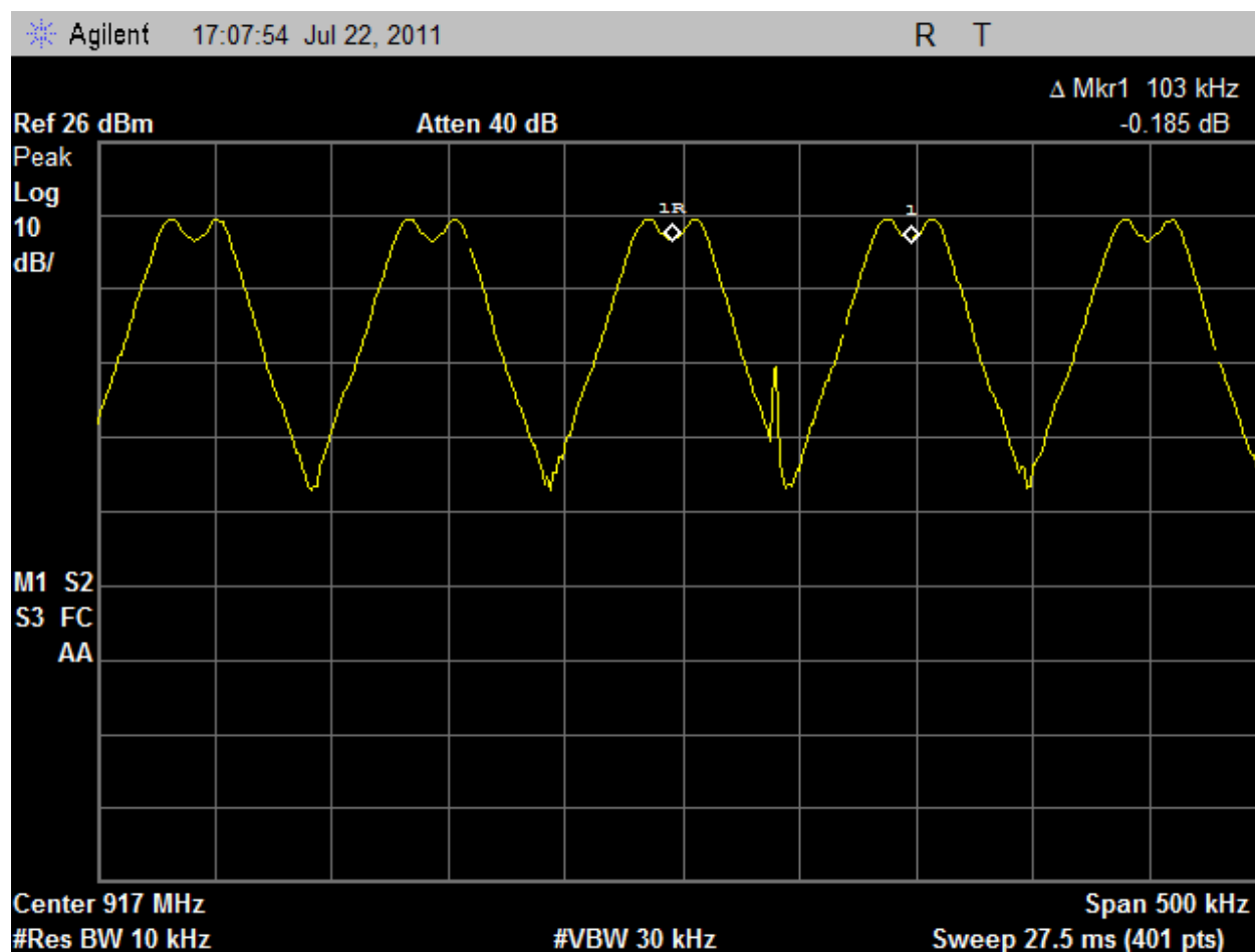
Plot 25 – Carrier Frequency Separation (Using Delta Marker Method)
