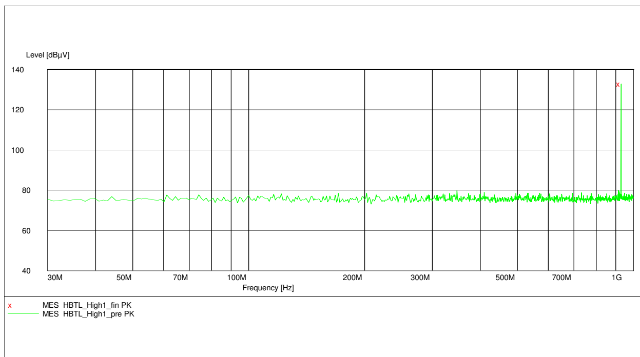
Plot 13 – Highest Channel (30MHz to 1GHz)
