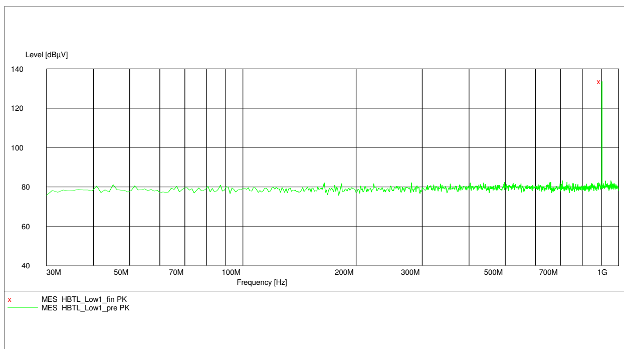
Plot 9 – Lowest Channel (30MHz to 1GHz)
