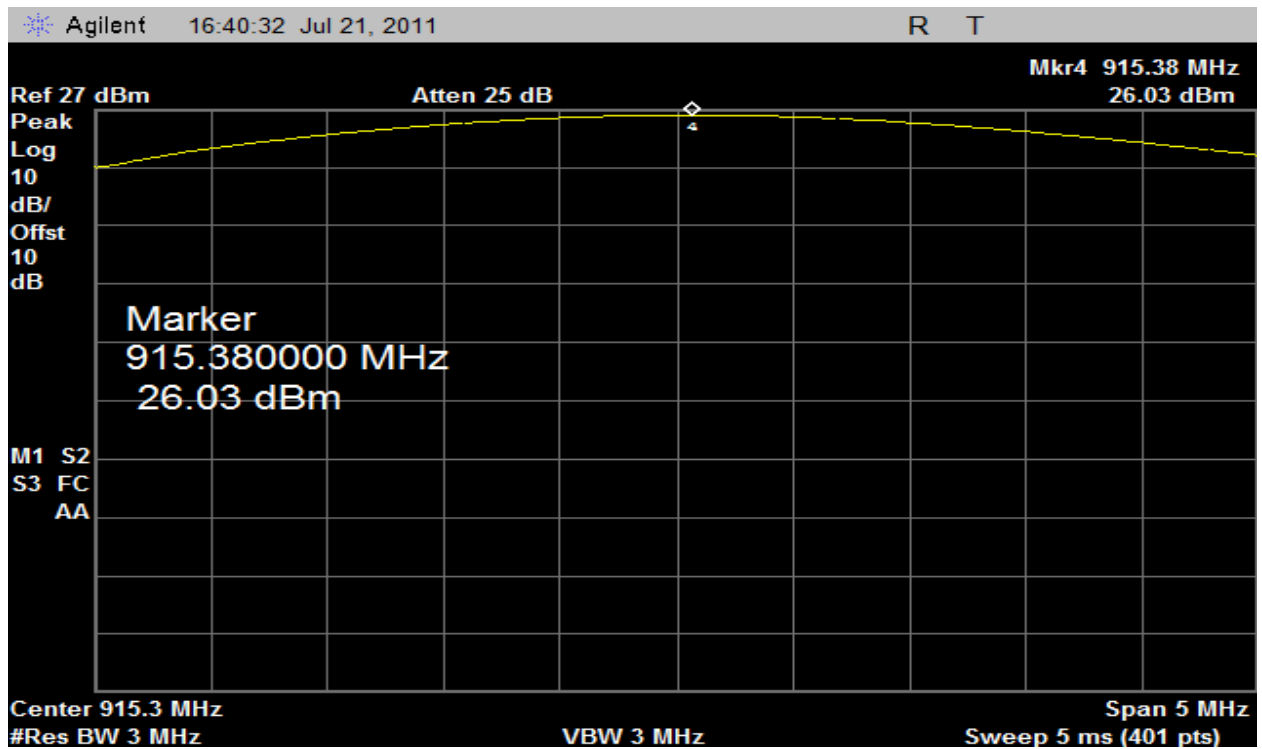
Plot 7 – Middle Channel -Output Power
