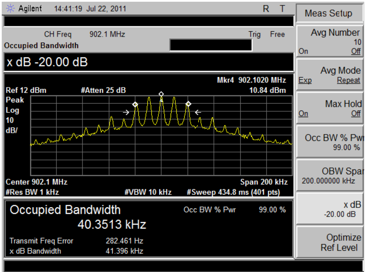
Plot 3 – Lowest Channel – 20dB BW FM Modulation
