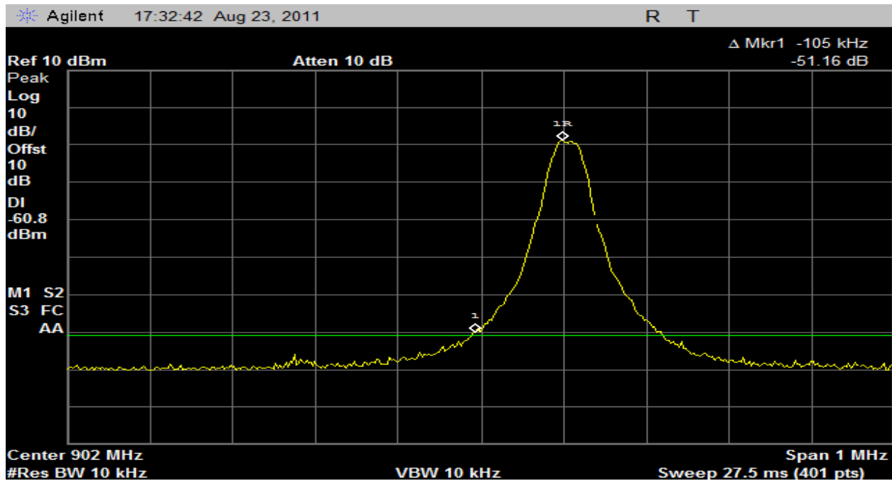
Plot 15 – Lowest Channel (Band Edge) 7.2dBi Antenna
