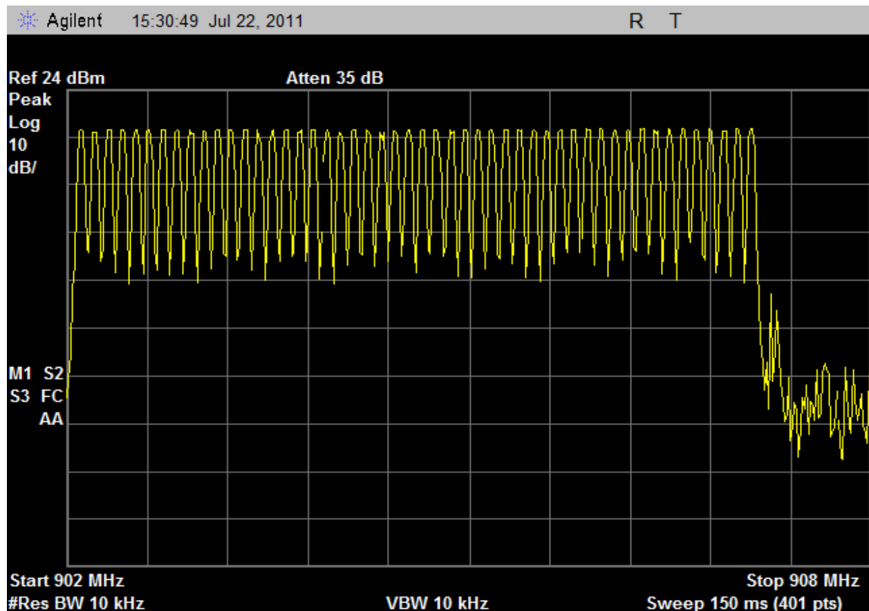
Plot 21 – Set 1 (902-907MHz)
