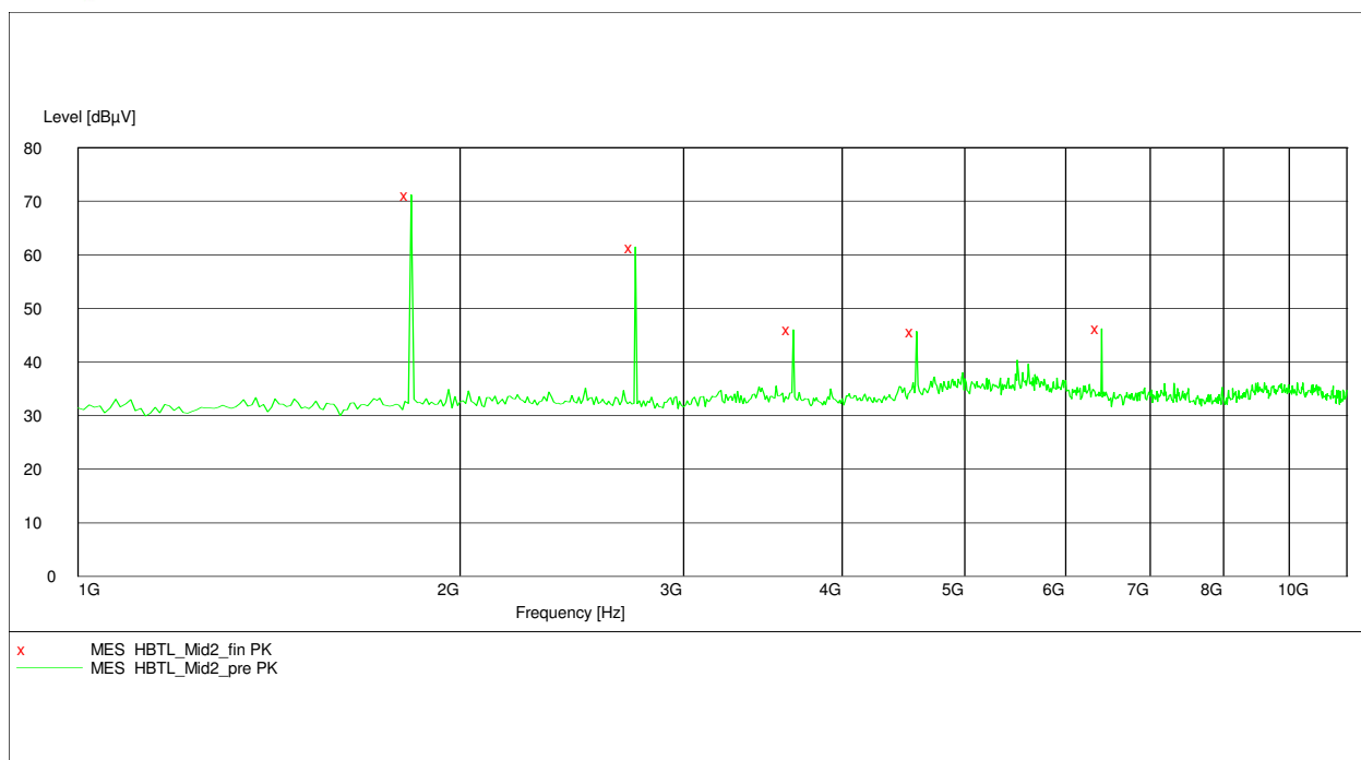
Plot 12 – Middle Channel (1GHz to 10GHz)
