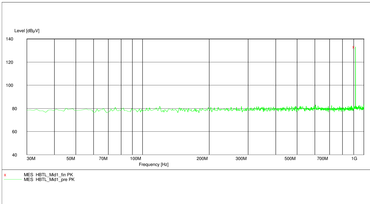
Plot 11 – Middle Channel (30MHz to 1GHz)
