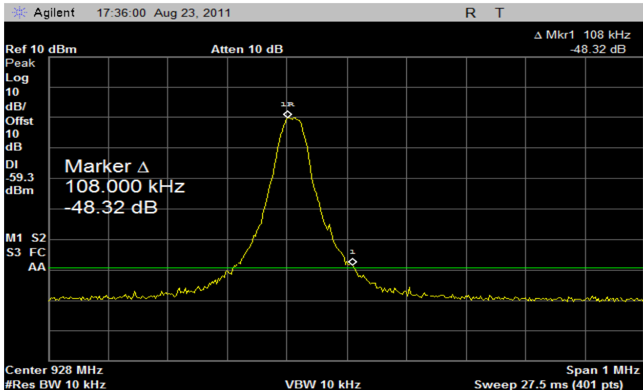
Plot 16 – Highest Channel (Band Edge) 7.2dBi Antenna
