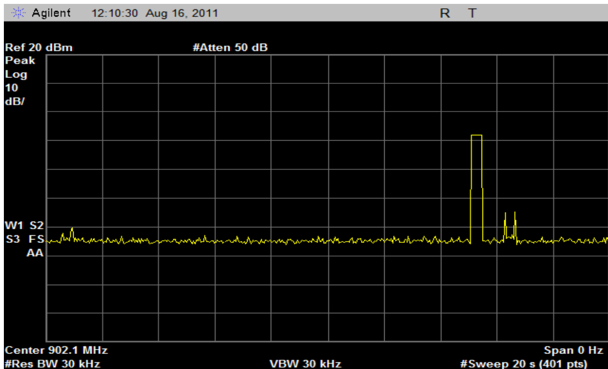
Plot 20 – # of Hops in 20 second period
