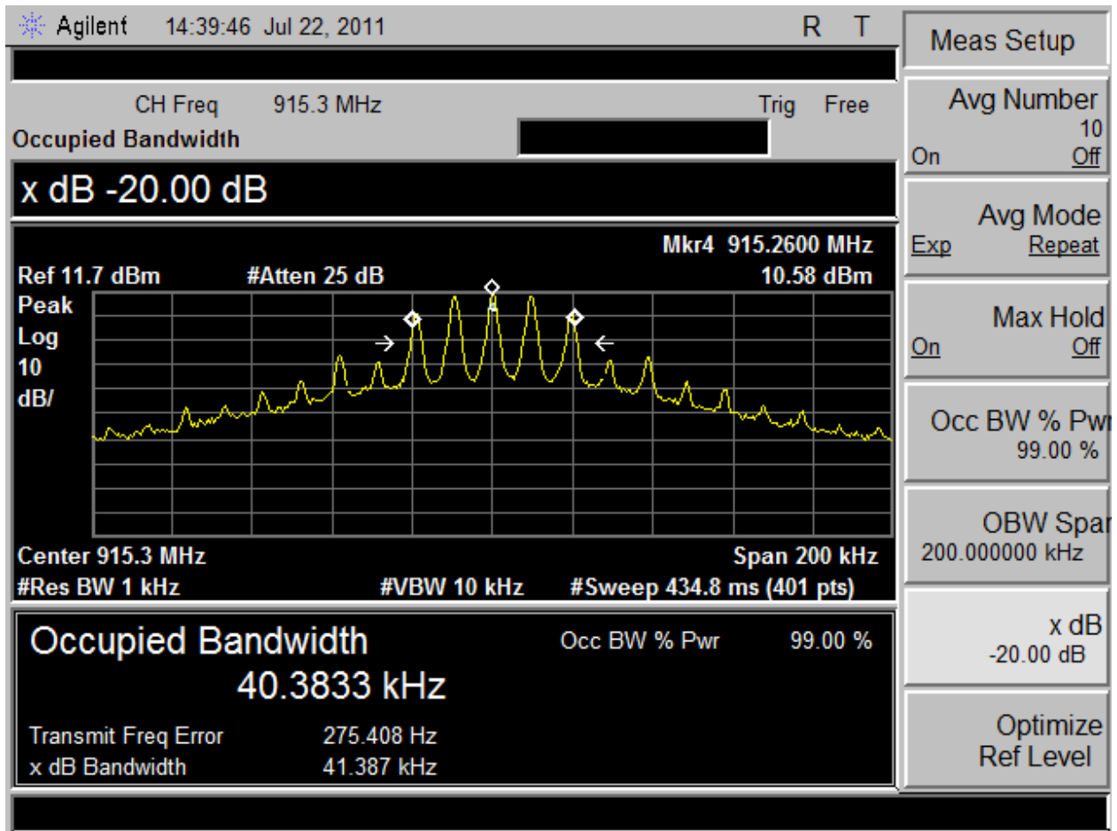
Plot 4 – Middle Channel – 20 BW FM Modulation
