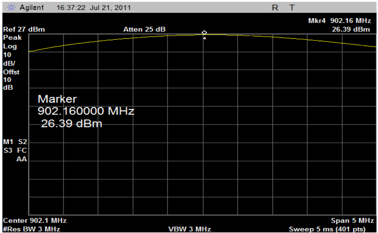
Plot 6 – Lowest Channel - Output Power
