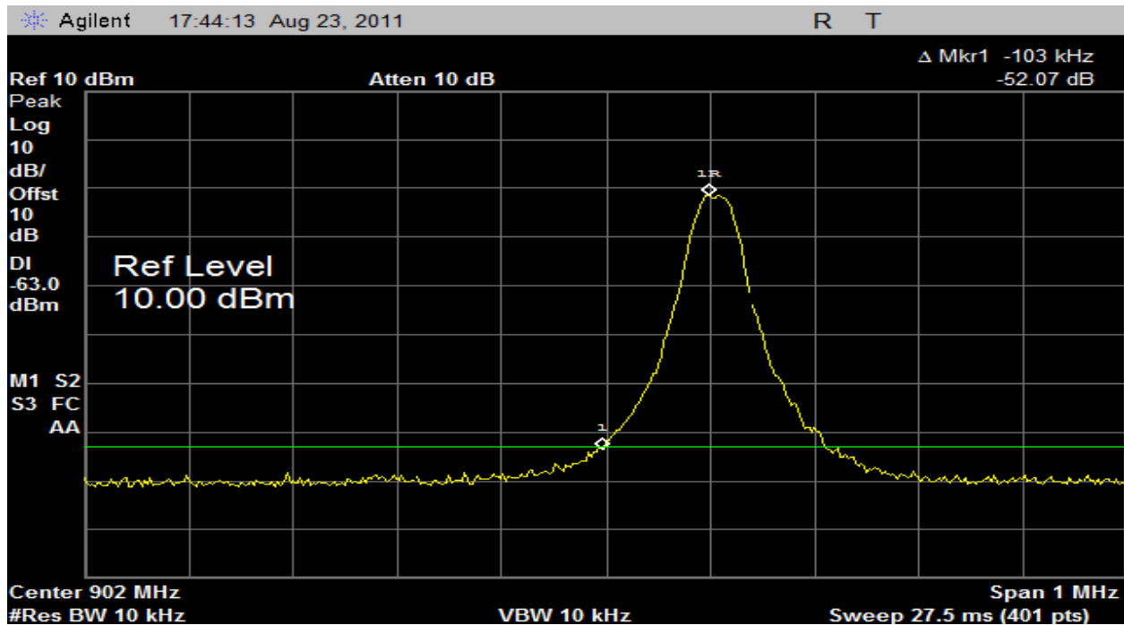
Plot 17 – Lowest Channel (Band Edge) Blade Antenna
