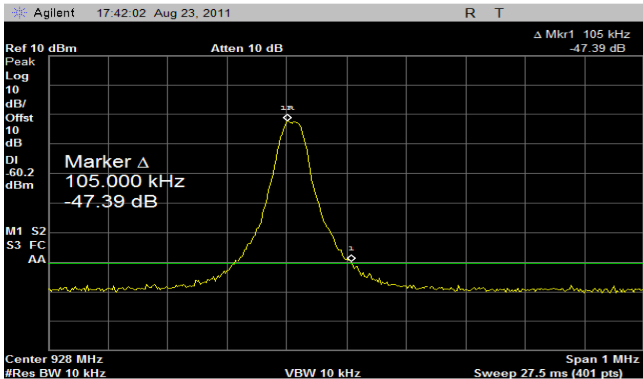
Plot 18 – Highest Channel (Band Edge) Blade Antenna
